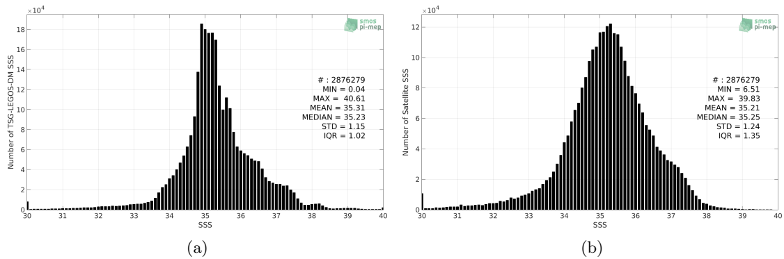
Figure 2: Histograms of SSS from TSG-LEGOS-DM (a) and SMOS L3 v317 - 10 Days - 25 km (CATDS-CPDC) (b) considering all match-up pairs per bins of 0.1 over the Global Ocean Pi-MEP region and for the full satellite product period.
