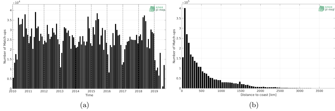
Figure 1: Number of match-ups between TSG-LEGOS-DM and SMOS L3 v317 - 10 Days - 25 km (CATDS-CPDC) SSS as a function of time (a) and as function of the distance to coast (b) over the Global Ocean Pi-MEP region and for the full satellite product period.
