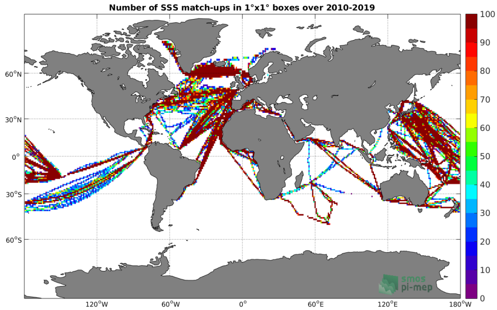
Figure 4: Number of SSS match-ups between TSG-LEGOS-DM SSS and the SMOS L3 v317 - 10 Days - 25 km (CATDS-CPDC) SSS product for the Global Ocean Pi-MEP region over 1°x1° boxes and for the full satellite product period.
