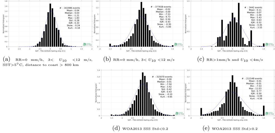
Figure 13: Normalized histogram of \Delta SSS (SMOS L3 v317 - 10 Days - 25 km (CATDS-CPDC) - TSG-GOSUD-Sailing-ship) for 5 different subdatasets corresponding to: RR=0 mm/h, 3 < U_{10} < 12 m/s, SST>5°C, distance to coast > 800 km (a), RR=0 mm/h, 3 < U_{10} < 12 m/s (b), RR>1mm/h and U_{10} < 4 m/s (c), WOA2013 SSS Std<0.2 (d), WOA2013 SSS Std>0.2 (e).
