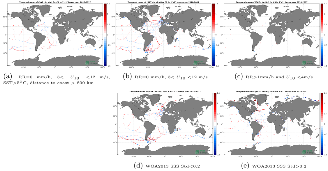
Figure 12: Temporal mean gridded over spatial boxes of size 1^\circ \times 1^\circ of \Delta SSS (SMOS L3 v317 - 10 Days - 25 km (CATDS-CPDC) - TSG-GOSUD-Sailing-ship) for 5 different subdatasets corresponding to:RR=0 mm/h, 3 < U_{10} < 12 m/s, SST>5°C, distance to coast > 800 km (a), RR=0 mm/h, 3 < U_{10} < 12 m/s (b), RR>1mm/h and U_{10} < 4 m/s (c), WOA2013 SSS Std<0.2 (d), WOA2013 SSS Std>0.2 (e).
