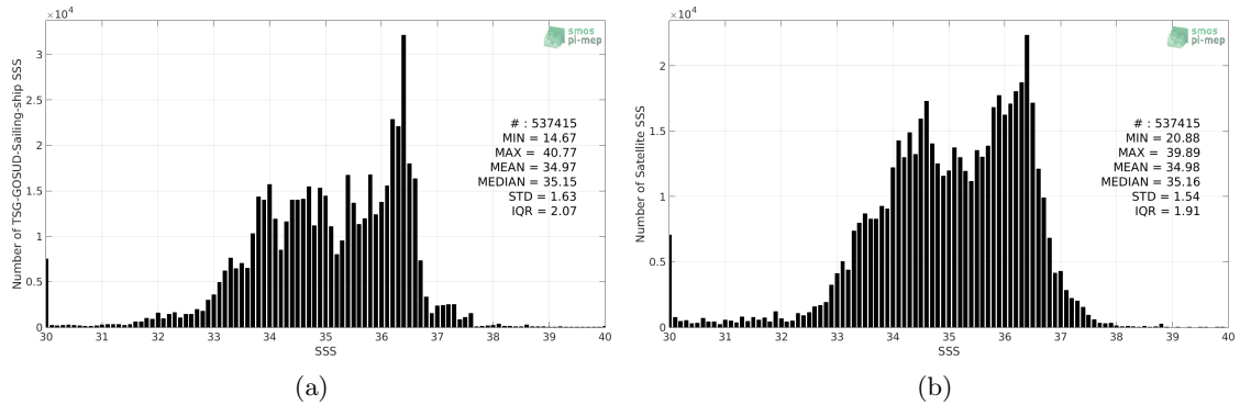
Figure 2: Histograms of SSS from TSG-GOSUD-Sailing-ship (a) and SMOS L3 v317 - 10 Days - 25 km (CATDS-CPDC) (b) considering all match-up pairs per bins of 0.1 over the Global Ocean Pi-MEP region and for the full satellite product period.
