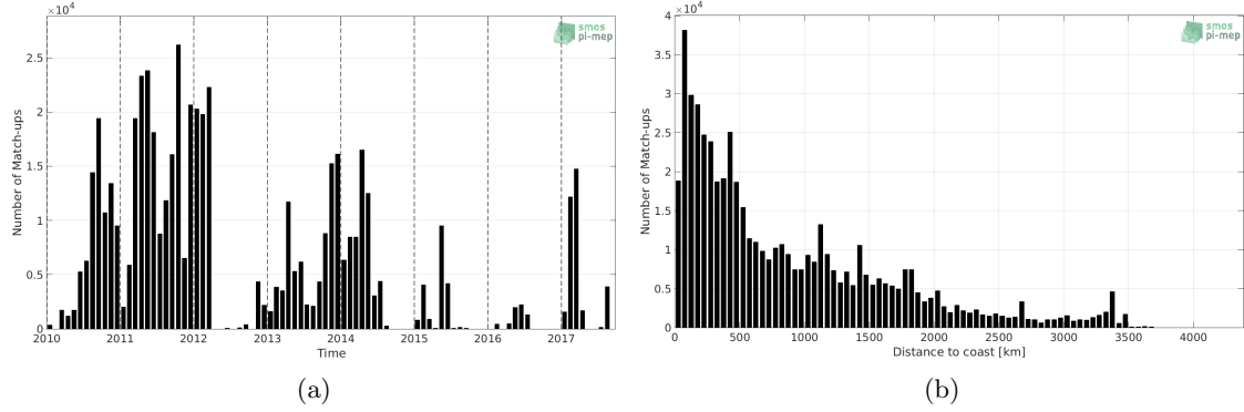
Figure 1: Number of match-ups between TSG-GOSUD-Sailing-ship and SMOS L3 v317 - 10 Days - 25 km (CATDS-CPDC) SSS as a function of time (a) and as function of the distance to coast (b) over the Global Ocean Pi-MEP region and for the full satellite product period.
