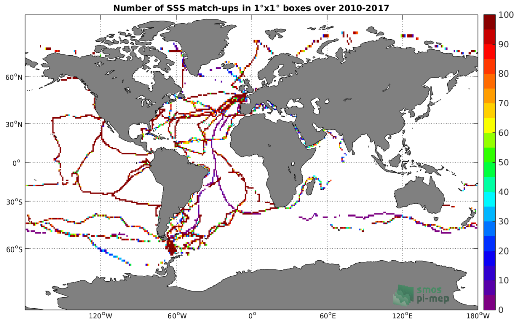
Figure 4: Number of SSS match-ups between TSG-GOSUD-Sailing-ship SSS and the SMOS L3 v317 - 10 Days - 25 km (CATDS-CPDC) SSS product for the Global Ocean Pi-MEP region over 1°x1° boxes and for the full satellite product period.
