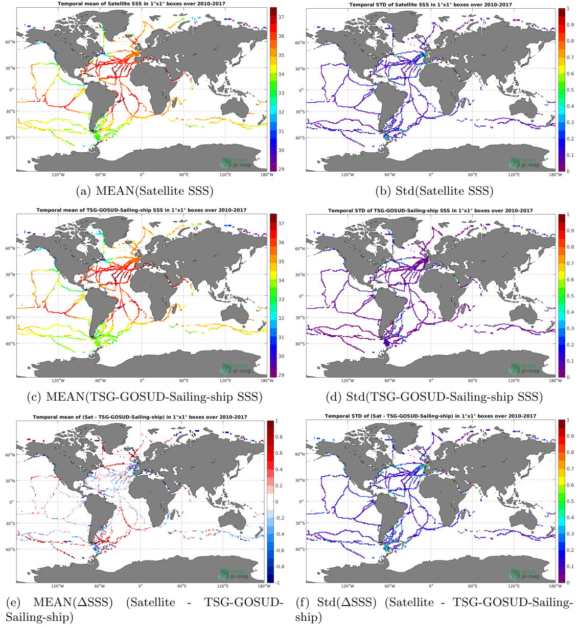
Figure 6: Temporal mean (left) and Std (right) of SSS from SMOS L3 v317 - 10 Days - 25 km (CATDS-CPDC) (top), TSG-GOSUD-Sailing-ship (middle), and of \Delta SSS (Satellite - TSG-GOSUD-Sailing-ship). Only match-up pairs are used to generate these maps.
