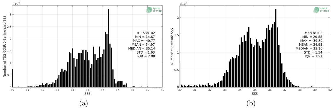
Figure 2: Histograms of SSS from TSG-GOSUD-Sailing-ship (a) and SMOS-L3-CATDS-CPDC-V317-10DAYS-25KM (b) considering all match-up pairs per bins of 0.1 over the Global Ocean Pi-MEP region and for the full satellite product period.
