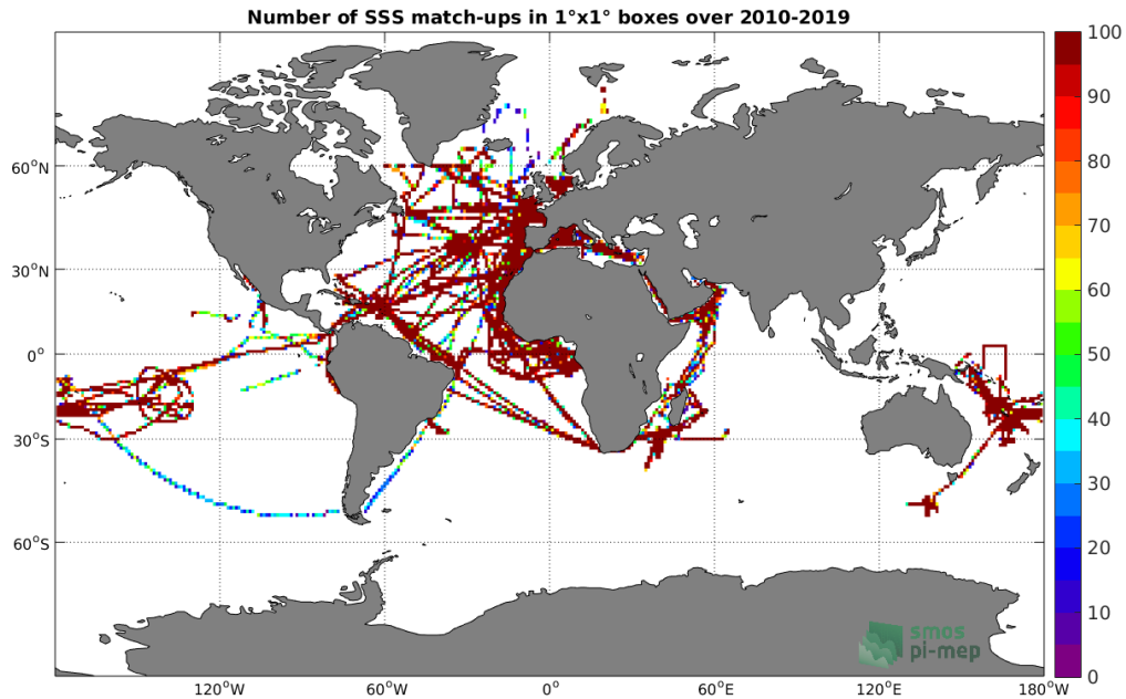
Figure 4: Number of SSS match-ups between TSG (GOSUD-Research-vessel) SSS and the SMOS SSS L3 v317 - 10 Days - 25 km (CATDS-CPDC) SSS product for the Global Ocean Pi-MEP region over 1°x1° boxes and for the full satellite product period.
