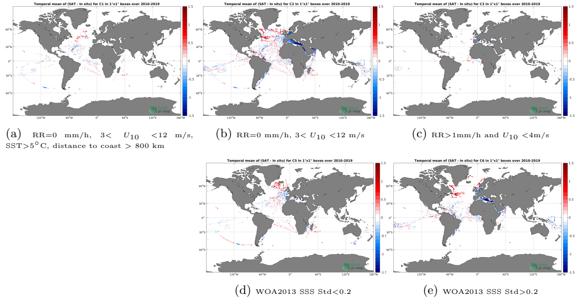
Figure 12: Temporal mean gridded over spatial boxes of size 1^\circ \times 1^\circ of \Delta SSS (SMOS SSS L3 v317 - 10 Days - 25 km (CATDS-CPDC) - TSG (GOSUD-Research-vessel)) for 5 different subdatasets corresponding to: RR=0 mm/h, 3 < U_{10} < 12 m/s, SST > 5^\circ C , distance to coast > 800 km (a), RR=0 mm/h, 3 < U_{10} < 12 m/s (b), RR > 1 mm/h and U_{10} < 4 m/s (c), WOA2013 SSS Std < 0.2 (d), WOA2013 SSS Std > 0.2 (e).
