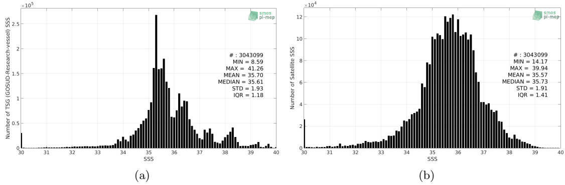
Figure 2: Histograms of SSS from TSG (GOSUD-Research-vessel) (a) and SMOS SSS L3 v317 - 10 Days - 25 km (CATDS-CPDC) (b) considering all match-up pairs per bins of 0.1 over the Global Ocean Pi-MEP region and for the full satellite product period.
