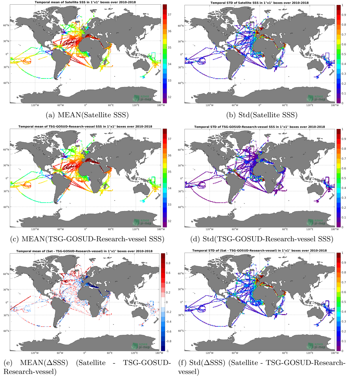
Figure 6: Temporal mean (left) and Std (right) of SSS from SMOS L3 v317 - 10 Days - 25 km (CATDS-CPDC) (top), TSG-GOSUD-Research-vessel (middle), and of \Delta SSS (Satellite - TSG-GOSUD-Research-vessel). Only match-up pairs are used to generate these maps.
