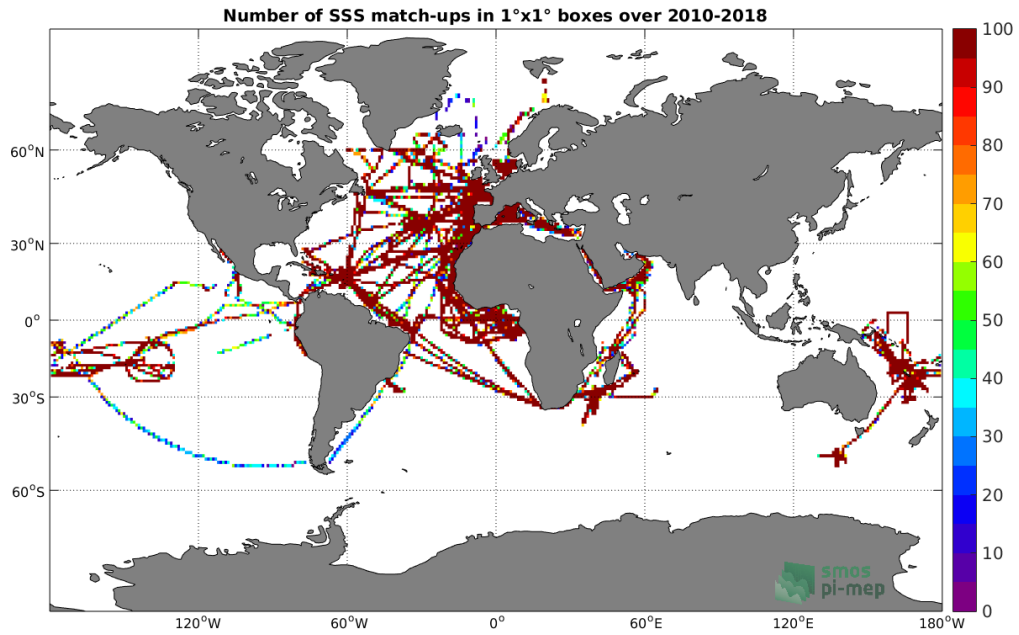
Figure 4: Number of SSS match-ups between TSG-GOSUD-Research-vessel SSS and the SMOS L3 v317 - 10 Days - 25 km (CATDS-CPDC) SSS product for the Global Ocean Pi-MEP region over 1^\circ \times 1^\circ boxes and for the full satellite product period.
