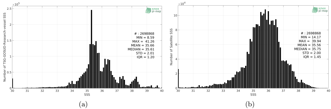
Figure 2: Histograms of SSS from TSG-GOSUD-Research-vessel (a) and SMOS L3 v317 - 10 Days - 25 km (CATDS-CPDC) (b) considering all match-up pairs per bins of 0.1 over the Global Ocean Pi-MEP region and for the full satellite product period.
