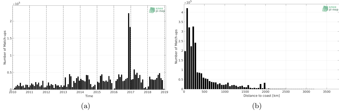
Figure 1: Number of match-ups between TSG-GOSUD-Research-vessel and SMOS L3 v317 - 10 Days - 25 km (CATDS-CPDC) SSS as a function of time (a) and as function of the distance to coast (b) over the Global Ocean Pi-MEP region and for the full satellite product period.
