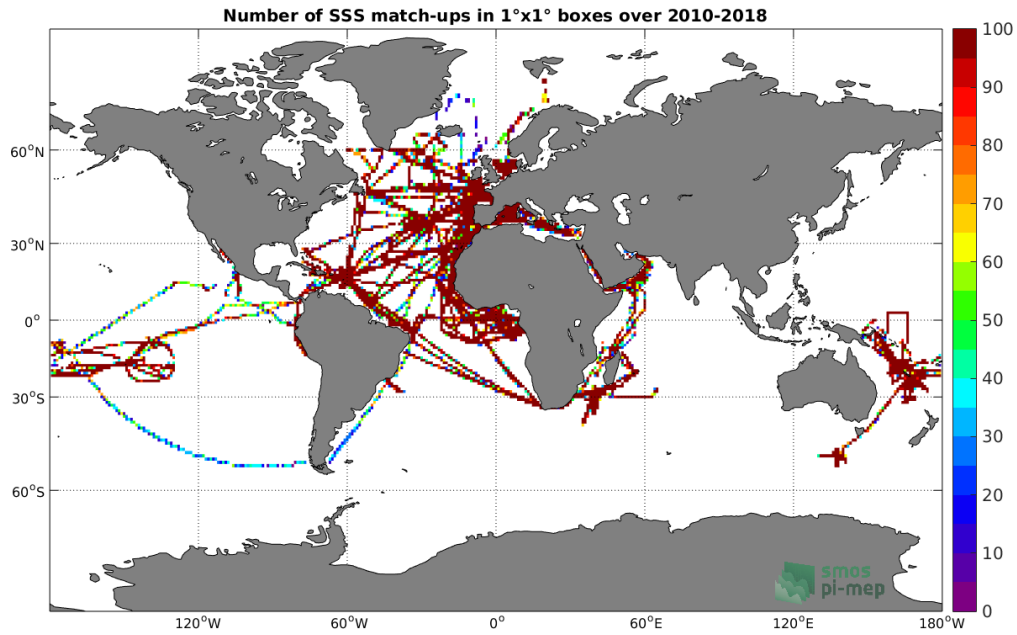
Figure 4: Number of SSS match-ups between TSG-GOSUD-Research-vessel SSS and the SMOS-L3-CATDS-CPDC-V317-10DAYS-25KM SSS product for the Global Ocean Pi-MEP region over 1°x1° boxes and for the full satellite product period.
