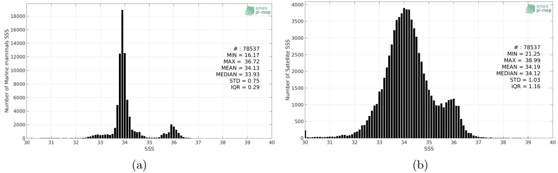
Figure 2: Histograms of SSS from Marine mammals (a) and SMOS SSS L3 v317 - 10 Days - 25 km (CATDS-CPDC) (b) considering all match-up pairs per bins of 0.1 over the Global Ocean Pi-MEP region and for the full satellite product period.
