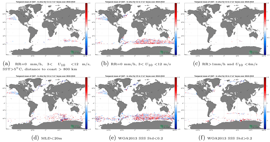
Figure 12: Temporal mean gridded over spatial boxes of size 1^\circ \times 1^\circ of \Delta SSS (SMOS SSS L3 v317 - 10 Days - 25 km (CATDS-CPDC) - Marine mammals) for 6 different subdatasets corresponding to: RR=0 mm/h, 3 < U_{10} < 12 m/s, SST > 5^\circ C , distance to coast > 800 km (a), RR=0 mm/h, 3 < U_{10} < 12 m/s (b), RR > 1 mm/h and U_{10} < 4 m/s (c), MLD < 20 m (d), WOA2013 SSS Std < 0.2 (e), WOA2013 SSS Std > 0.2 (f).
