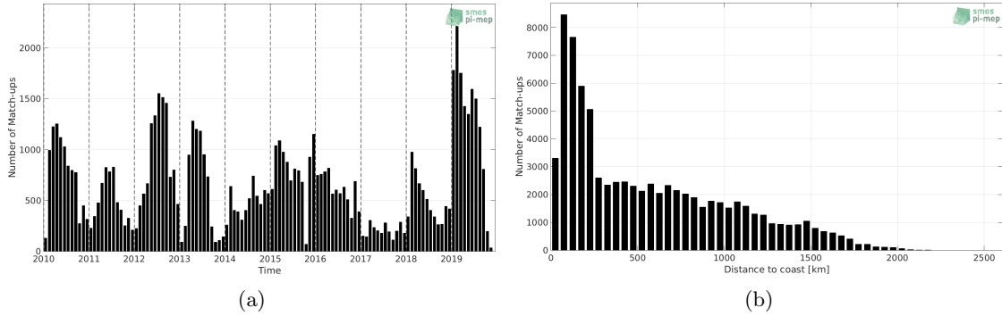
Figure 1: Number of match-ups between Marine mammals and SMOS SSS L3 v317 - 10 Days - 25 km (CATDS-CPDC) SSS as a function of time (a) and as function of the distance to coast (b) over the Global Ocean Pi-MEP region and for the full satellite product period.
