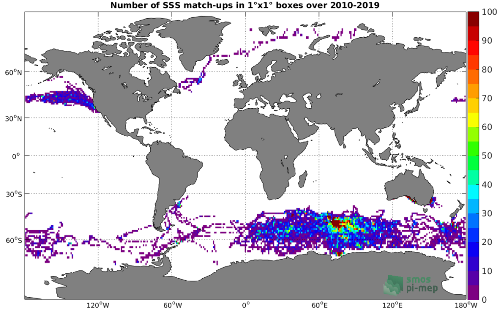
Figure 4: Number of SSS match-ups between Marine mammals SSS and the SMOS SSS L3 v317 - 10 Days - 25 km (CATDS-CPDC) SSS product for the Global Ocean Pi-MEP region over 1^\circ \times 1^\circ boxes and for the full satellite product period.
