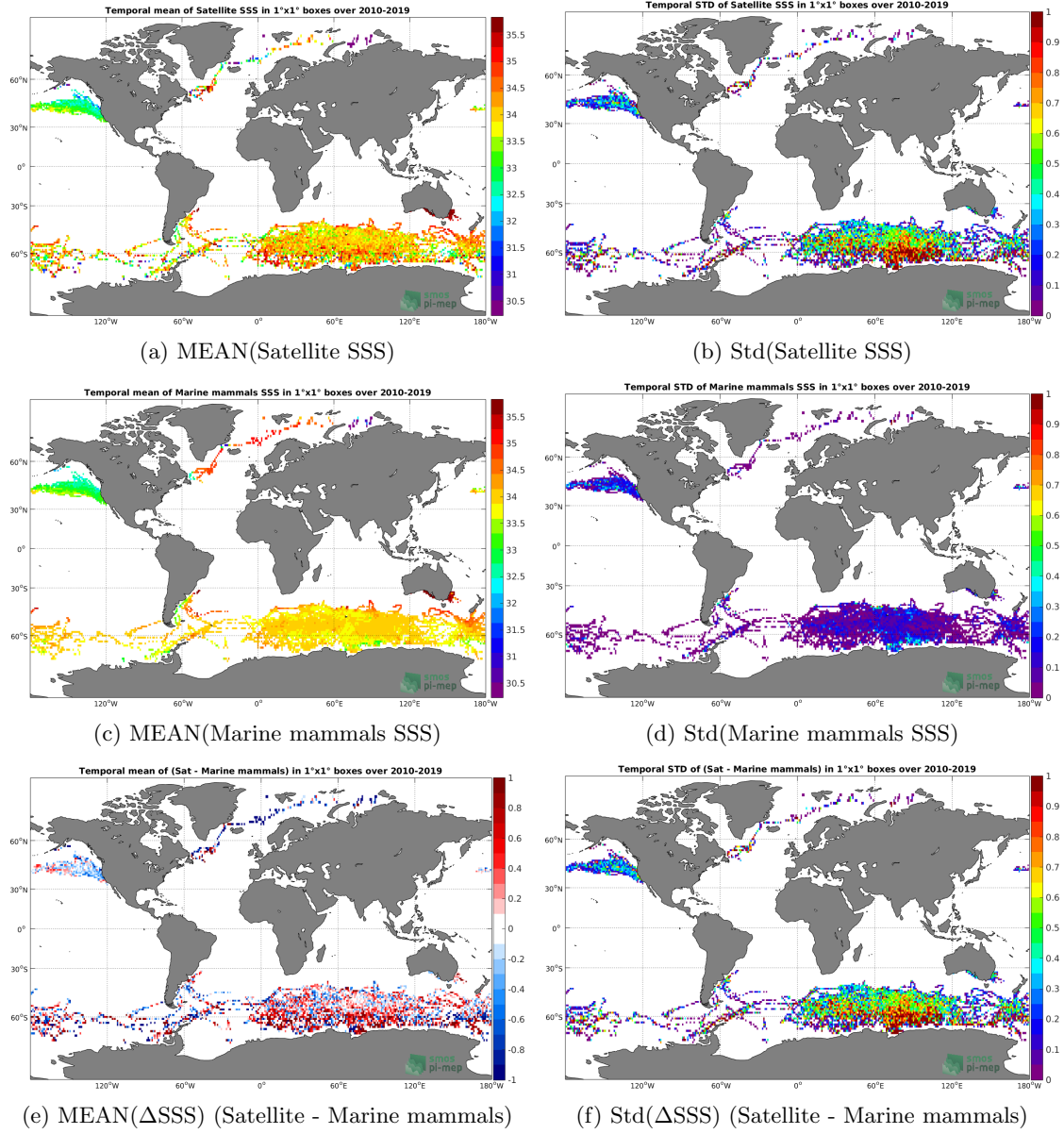
Figure 6: Temporal mean (left) and Std (right) of SSS from SMOS SSS L3 v317 - 10 Days - 25 km (CATDS-CPDC) (top), Marine mammals (middle), and of \Delta SSS (Satellite - Marine mammals). Only match-up pairs are used to generate these maps.
