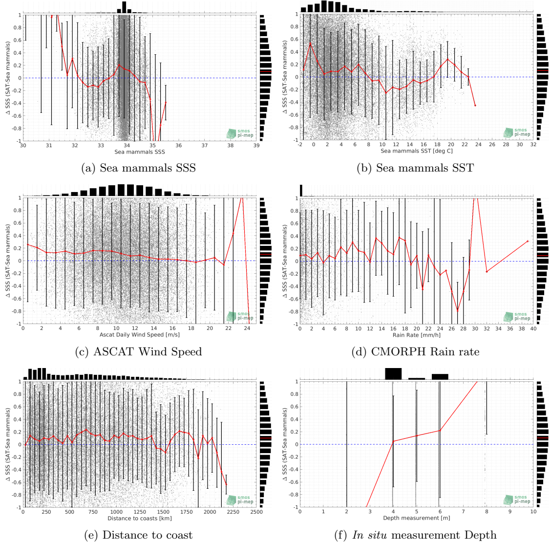
Figure 11: \Delta SSS (Satellite - Sea mammals) sorted as function of Sea mammals SSS values (a), Sea mammals SST (b), ASCAT Wind speed (c), CMORPH rain rate (d), distance to coast (e) and in situ measurement depth (f). In all plots the median and Std of \Delta SSS for each bin is indicated by the red curves and black vertical thick bars ( \pm 1 Std)
