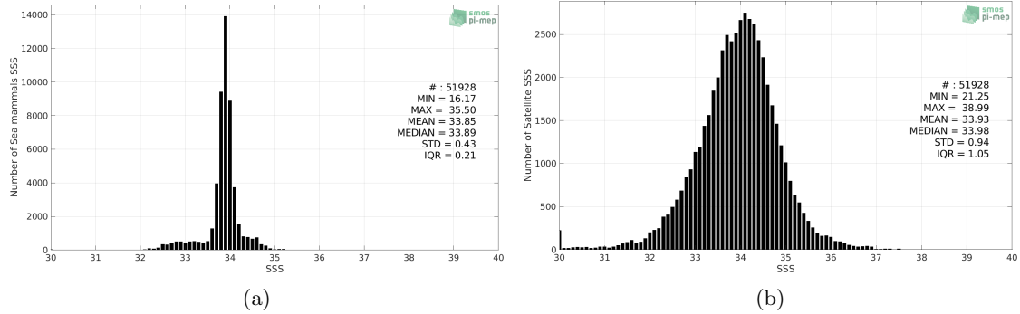
Figure 2: Histograms of SSS from Sea mammals (a) and SMOS SSS L3 v317 - 10 Days - 25 km (CATDS-CPDC) (b) considering all match-up pairs per bins of 0.1 over the Global Ocean Pi-MEP region and for the full satellite product period.
