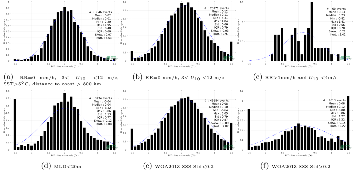
Figure 13: Normalized histogram of \Delta\text{SSS} (SMOS SSS L3 v317 - 10 Days - 25 km (CATDS-CPDC) - Sea mammals) for 6 different subdatasets corresponding to: RR=0 mm/h, 3 < U_{10} < 12 m/s, SST>5°C, distance to coast > 800 km (a), RR=0 mm/h, 3 < U_{10} < 12 m/s (b), RR>1mm/h and U_{10} < 4 m/s (c), MLD<20m (d), WOA2013 SSS Std<0.2 (e), WOA2013 SSS Std>0.2 (f).
