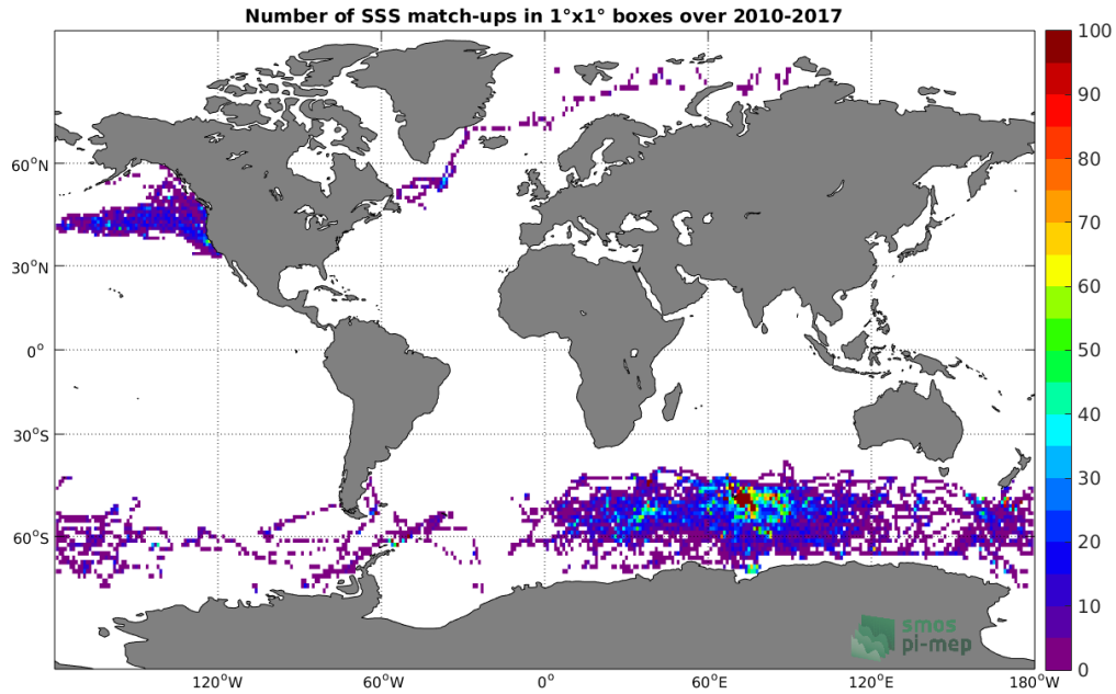
Figure 4: Number of SSS match-ups between Sea mammals SSS and the SMOS SSS L3 v317 - 10 Days - 25 km (CATDS-CPDC) SSS product for the Global Ocean Pi-MEP region over 1^\circ \times 1^\circ boxes and for the full satellite product period.
