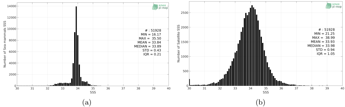
Figure 2: Histograms of SSS from Sea mammals (a) and SMOS SSS L3 v317 - 10 Days - 25 km (CATDS-CPDC) (b) considering all match-up pairs per bins of 0.1 over the Global Ocean Pi-MEP region and for the full satellite product period.
