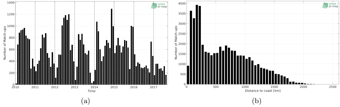
Figure 1: Number of match-ups between Sea mammals and SMOS SSS L3 v317 - 10 Days - 25 km (CATDS-CPDC) SSS as a function of time (a) and as function of the distance to coast (b) over the Global Ocean Pi-MEP region and for the full satellite product period.
