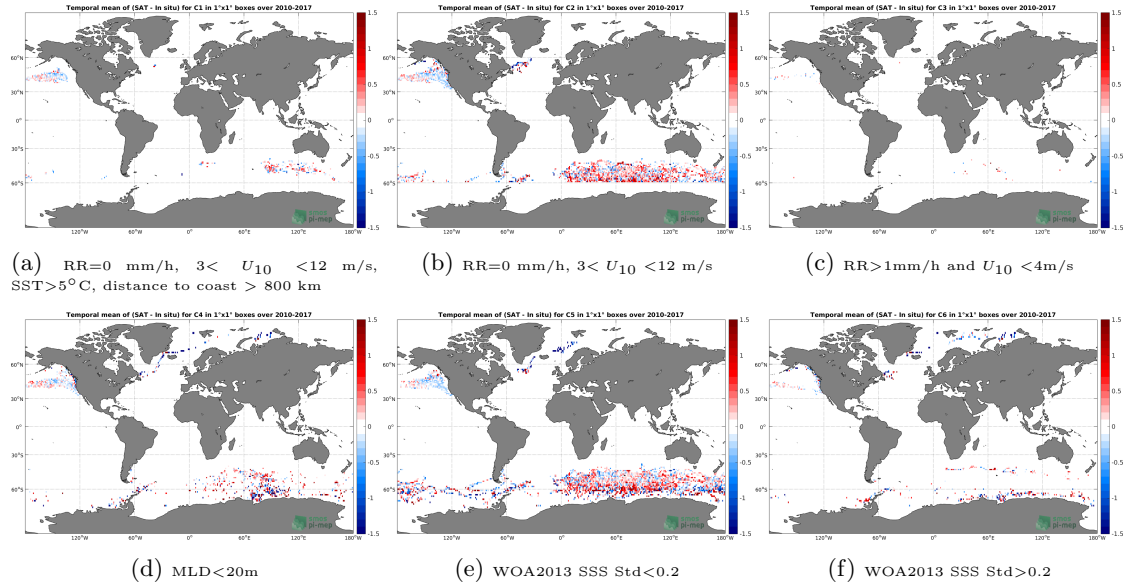
Figure 12: Temporal mean gridded over spatial boxes of size 1^\circ \times 1^\circ of \Delta SSS (SMOS SSS L3 v317 - 10 Days - 25 km (CATDS-CPDC) - Sea mammals) for 6 different subdatasets corresponding to: RR=0 mm/h, 3 < U_{10} < 12 m/s, SST > 5^\circ C , distance to coast > 800 km (a), RR=0 mm/h, 3 < U_{10} < 12 m/s (b), RR > 1 mm/h and U_{10} < 4 m/s (c), MLD < 20 m (d), WOA2013 SSS Std < 0.2 (e), WOA2013 SSS Std > 0.2 (f).
