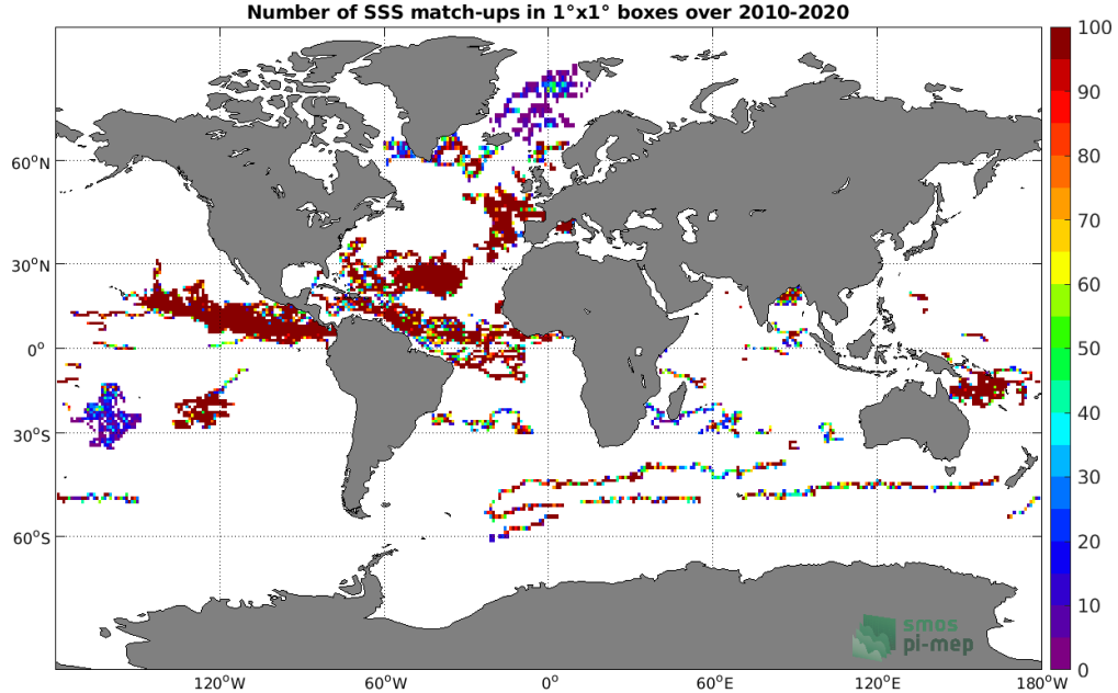
Figure 3: Number of SSS match-ups between Surface drifters SSS and the SMOS SSS L3 v317 - 10 Days - 25 km (CATDS-CPDC) SSS product for the Global Ocean Pi-MEP region over 1^\circ \times 1^\circ boxes and for the full satellite product period.
