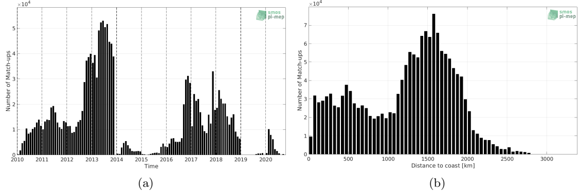
Figure 1: Number of match-ups between Surface drifters and SMOS SSS L3 v317 - 10 Days - 25 km (CATDS-CPDC) SSS as a function of time (a) and as function of the distance to coast (b) over the Global Ocean Pi-MEP region and for the full satellite product period.
