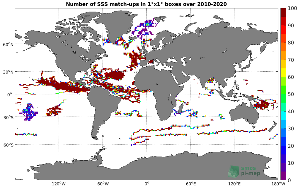
Figure 3: Number of SSS match-ups between Surface drifters SSS and the SMOS SSS L3 v317 - 10 Days - 25 km (CATDS-CPDC) SSS product for the Global Ocean Pi-MEP region over 1^\circ \times 1^\circ boxes and for the full satellite product period.
