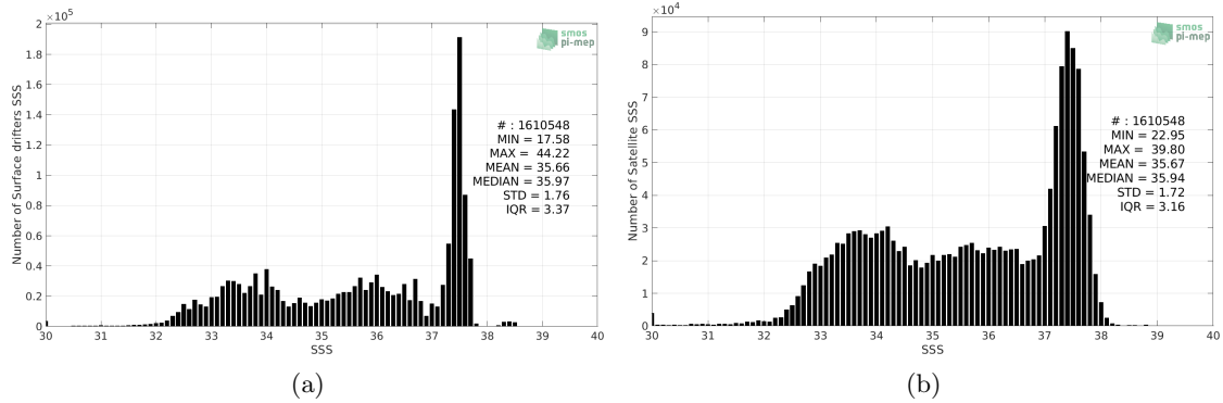
Figure 2: Histograms of SSS from Surface drifters (a) and SMOS SSS L3 v317 - 10 Days - 25 km (CATDS-CPDC) (b) considering all match-up pairs per bins of 0.1 over the Global Ocean Pi-MEP region and for the full satellite product period.
