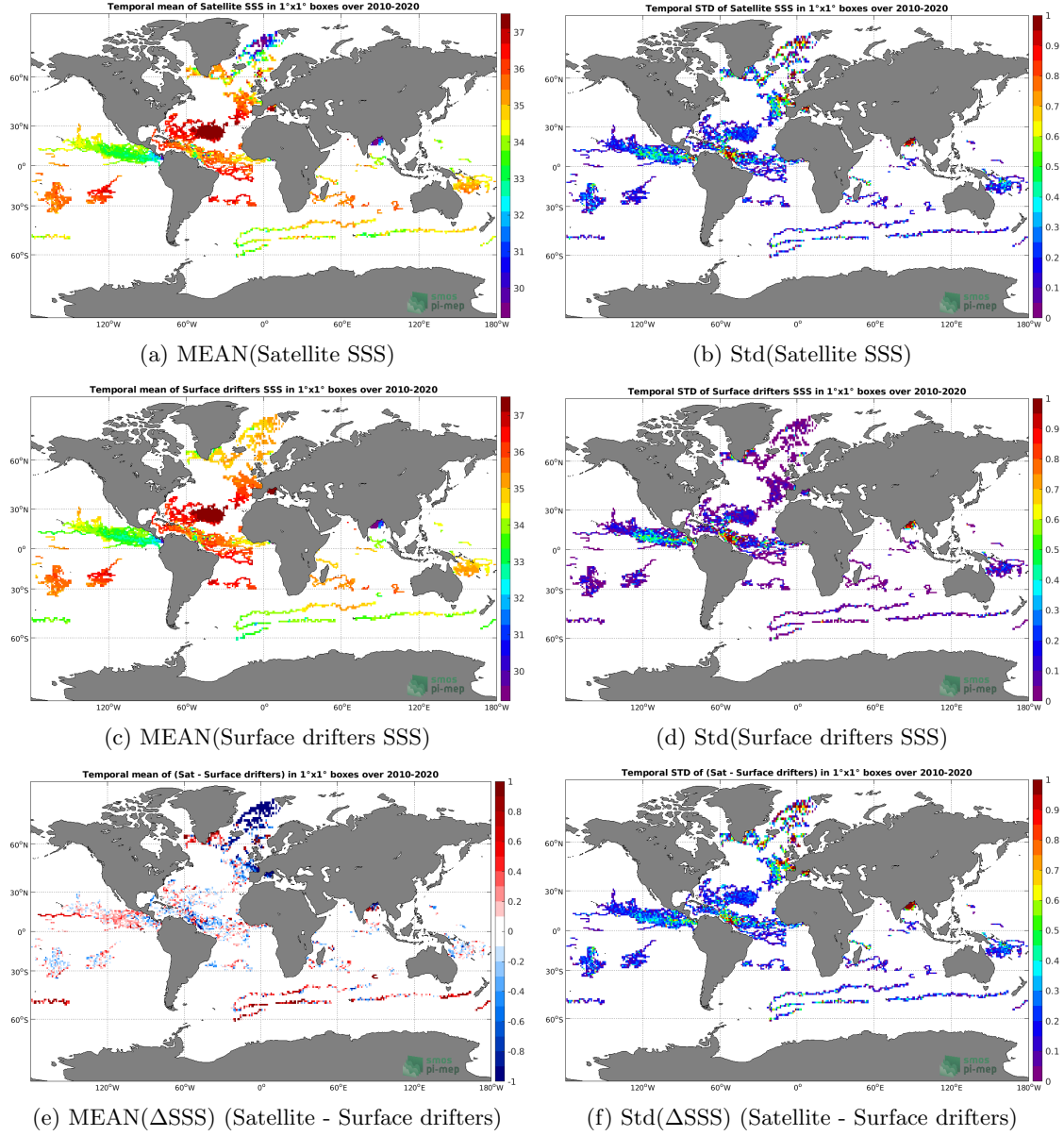
Figure 5: Temporal mean (left) and Std (right) of SSS from SMOS SSS L3 v317 - 10 Days - 25 km (CATDS-CPDC) (top), Surface drifters (middle), and of \Delta SSS (Satellite - Surface drifters). Only match-up pairs are used to generate these maps.
