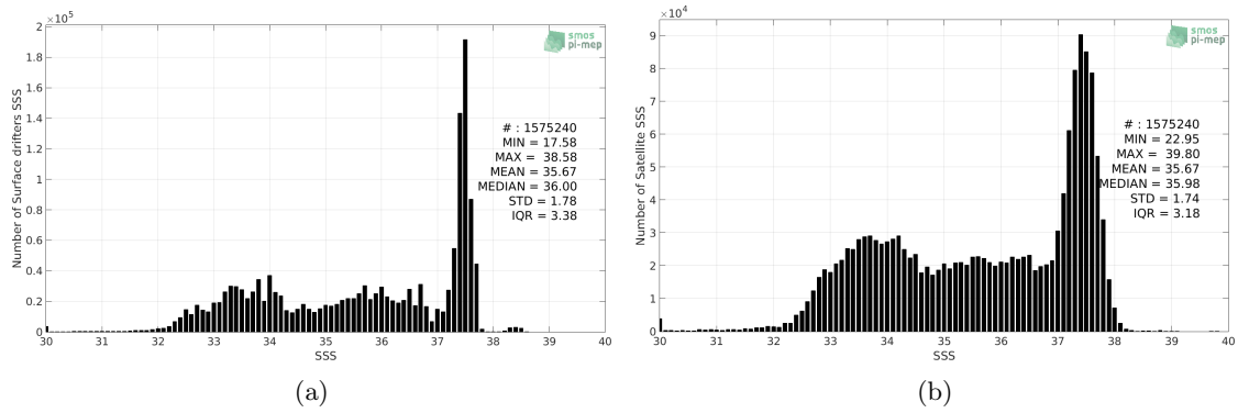
Figure 2: Histograms of SSS from Surface drifters (a) and SMOS L3 v317 - 10 Days - 25 km (CATDS-CPDC) (b) considering all match-up pairs per bins of 0.1 over the Global Ocean Pi-MEP region and for the full satellite product period.
