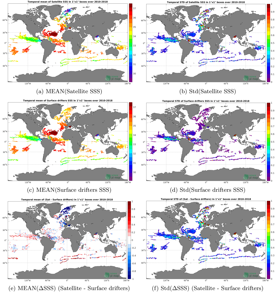
Figure 5: Temporal mean (left) and Std (right) of SSS from SMOS L3 v317 - 10 Days - 25 km (CATDS-CPDC) (top), Surface drifters (middle), and of \Delta SSS (Satellite - Surface drifters). Only match-up pairs are used to generate these maps.
