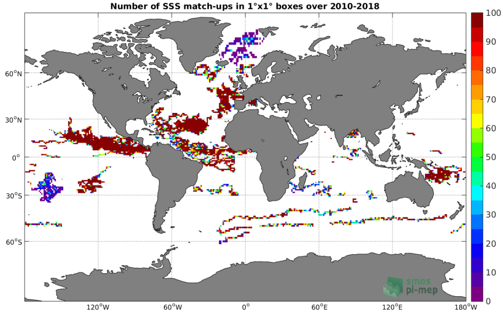
Figure 3: Number of SSS match-ups between Surface drifters SSS and the SMOS L3 v317 - 10 Days - 25 km (CATDS-CPDC) SSS product for the Global Ocean Pi-MEP region over 1^\circ \times 1^\circ boxes and for the full satellite product period.
