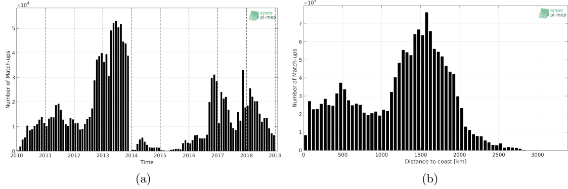
Figure 1: Number of match-ups between Surface drifters and SMOS L3 v317 - 10 Days - 25 km (CATDS-CPDC) SSS as a function of time (a) and as function of the distance to coast (b) over the Global Ocean Pi-MEP region and for the full satellite product period.
