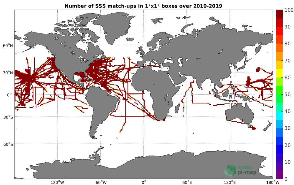
Figure 4: Number of SSS match-ups between TSG-SAMOS SSS and the SMOS-L3-CATDS-CPDC-V3-MONTHLY-25KM SSS product for the Global Ocean Pi-MEP region over 1^\circ \times 1^\circ boxes and for the full satellite product period.
