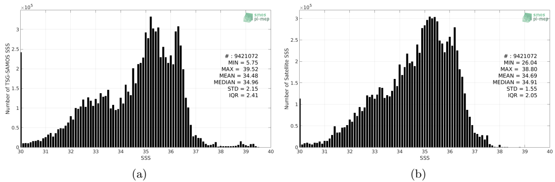
Figure 2: Histograms of SSS from TSG-SAMOS (a) and SMOS-L3-CATDS-CPDC-V3-MONTHLY-25KM (b) considering all match-up pairs per bins of 0.1 over the Global Ocean Pi-MEP region and for the full satellite product period.
