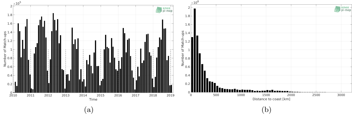
Figure 1: Number of match-ups between TSG-SAMOS and SMOS-L3-CATDS-CPDC-V3-MONTHLY-25KM SSS as a function of time (a) and as function of the distance to coast (b) over the Global Ocean Pi-MEP region and for the full satellite product period.
