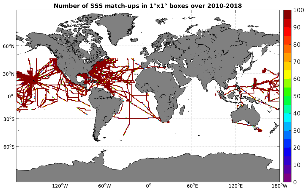
Figure 4: Number of SSS match-ups between TSG-SAMOS SSS and the SMOS-L3-CATDS-CPDC-V3-MONTHLY-25KM SSS product for the Global Ocean Pi-MEP region over 1^\circ \times 1^\circ boxes and for the full satellite product period.
