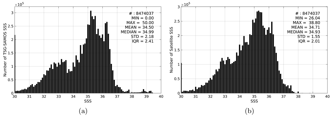
Figure 2: Histograms of SSS from TSG-SAMOS (a) and SMOS-L3-CATDS-CPDC-V3-MONTHLY-25KM (b) considering all match-up pairs per bins of 0.1 over the Global Ocean Pi-MEP region and for the full satellite product period.
