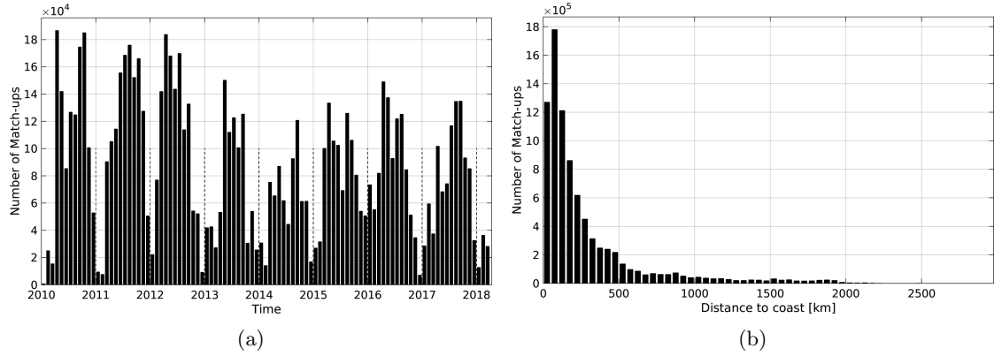
Figure 1: Number of match-ups between TSG-SAMOS and SMOS-L3-CATDS-CPDC-V3-MONTHLY-25KM SSS as a function of time (a) and as function of the distance to coast (b) over the Global Ocean Pi-MEP region and for the full satellite product period.
