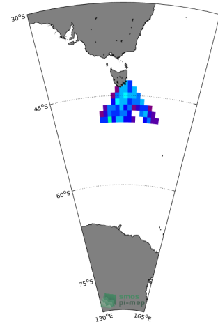
(f) STD( \Delta SSS) (Satellite - TSG-LEGOS-Survostral)
