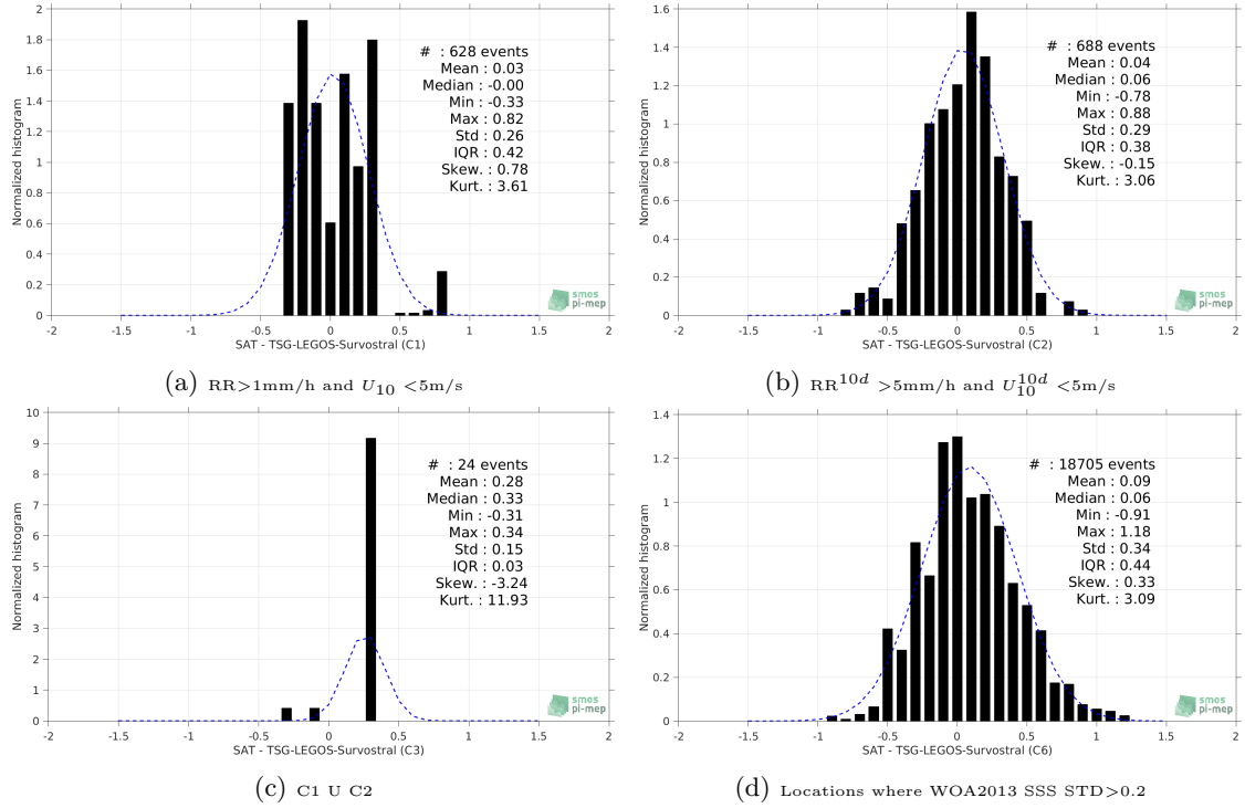
Figure 13: Normalized histogram of \Delta\text{SSS} (SMOS-L3-CATDS-CPDC-V3-MONTHLY-25KM - TSG-LEGOS-Survostral) for 6 different subdatasets corresponding to: RR > 1mm/h and U_{10} < 5\text{m/s} (a), RR^{10d} > 5\text{mm/h} and U_{10}^{10d} < 5\text{m/s} (b), C1 U C2 (c), Locations where WOA2013 SSS STD > 0.2 (d).
