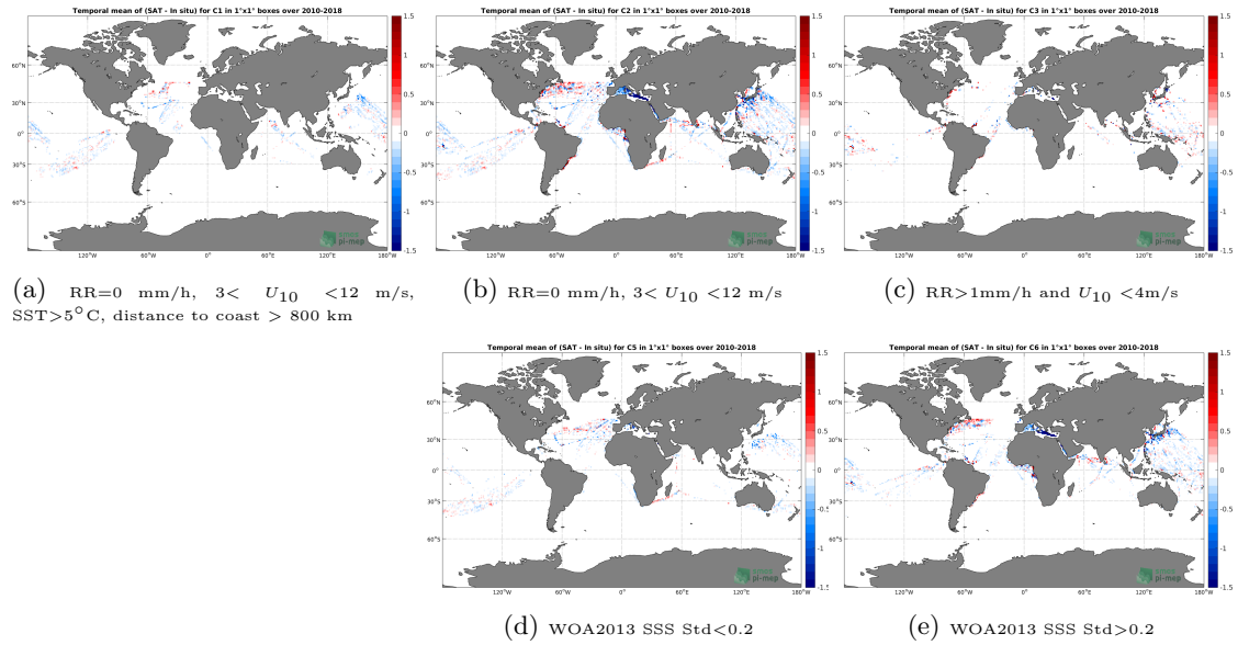
Figure 12: Temporal mean gridded over spatial boxes of size 1^\circ \times 1^\circ of \Delta SSS (SMOS-L3-CATDS-CPDC-V3-MONTHLY-25KM - TSG-LEGOS-DM) for 5 different subdatasets corresponding to:RR=0 mm/h, 3 < U_{10} < 12 m/s, SST >5^\circ C, distance to coast > 800 km (a), RR=0 mm/h, 3 < U_{10} < 12 m/s (b), RR >1 mm/h and U_{10} < 4 m/s (c), WOA2013 SSS Std <0.2 (d), WOA2013 SSS Std >0.2 (e).
