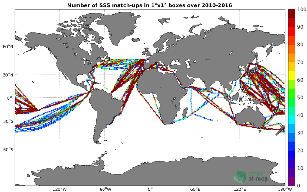
Figure 4: Number of SSS match-ups between TSG-LEGOS-DM SSS and the SMOS-L3-CATDS-CPDC-V3-MONTHLY-25KM SSS product for the Global Ocean Pi-MEP region over 1^\circ \times 1^\circ boxes and for the full satellite product period.
