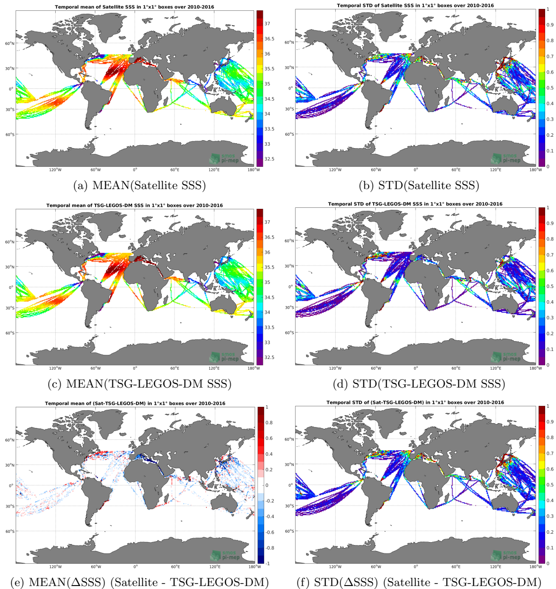
Figure 6: Temporal mean (left) and STD (right) of SSS from SMOS-L3-CATDS-CPDC-V3-MONTHLY-25KM (top), TSG-LEGOS-DM (middle), and of \Delta SSS (Satellite - TSG-LEGOS-DM). Only match-up pairs are used to generate these maps.
