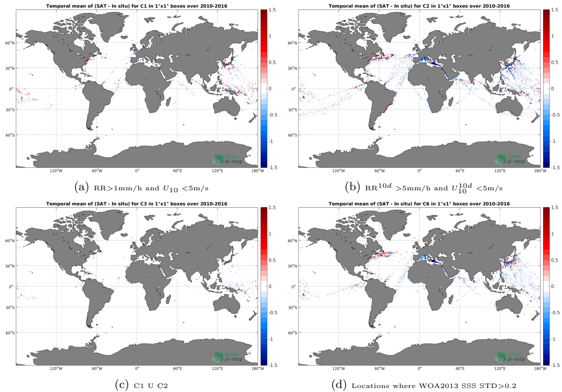
Figure 12: Temporal mean gridded over spatial boxes of size 1^\circ \times 1^\circ of \Delta\text{SSS} (SMOS-L3-CATDS-CPDC-V3-MONTHLY-25KM - TSG-LEGOS-DM) for 4 different subdatasets corresponding to: RR > 1\text{mm/h} and U_{10} < 5\text{m/s} (a), RR^{10d} > 5\text{mm/h} and U_{10}^{10d} < 5\text{m/s} (b), C1 U C2 (c), Locations where WOA2013 SSS STD > 0.2 (d).
