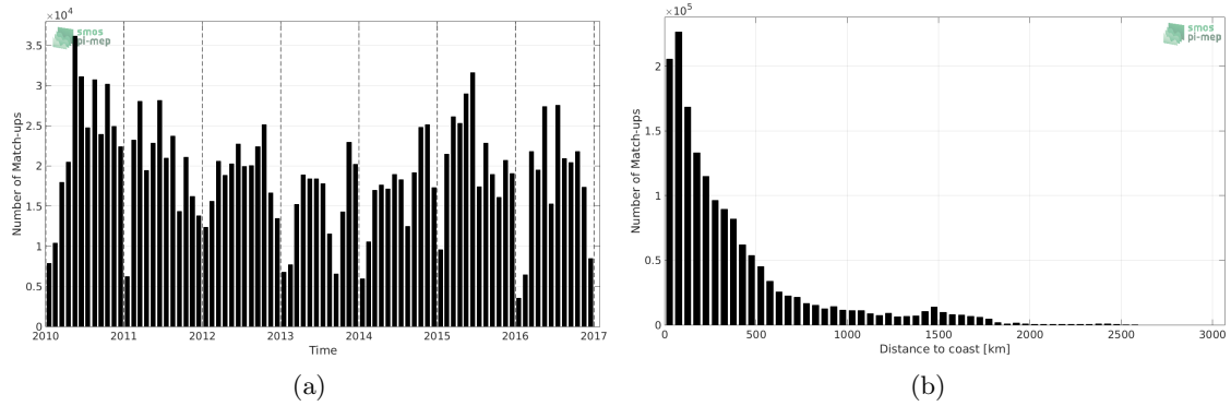
Figure 1: Number of match-ups between TSG-LEGOS-DM and SMOS-L3-CATDS-CPDC-V3-MONTHLY-25KM SSS as a function of time (a) and as function of the distance to coast (b) over the Global Ocean Pi-MEP region and for the full satellite product period.
