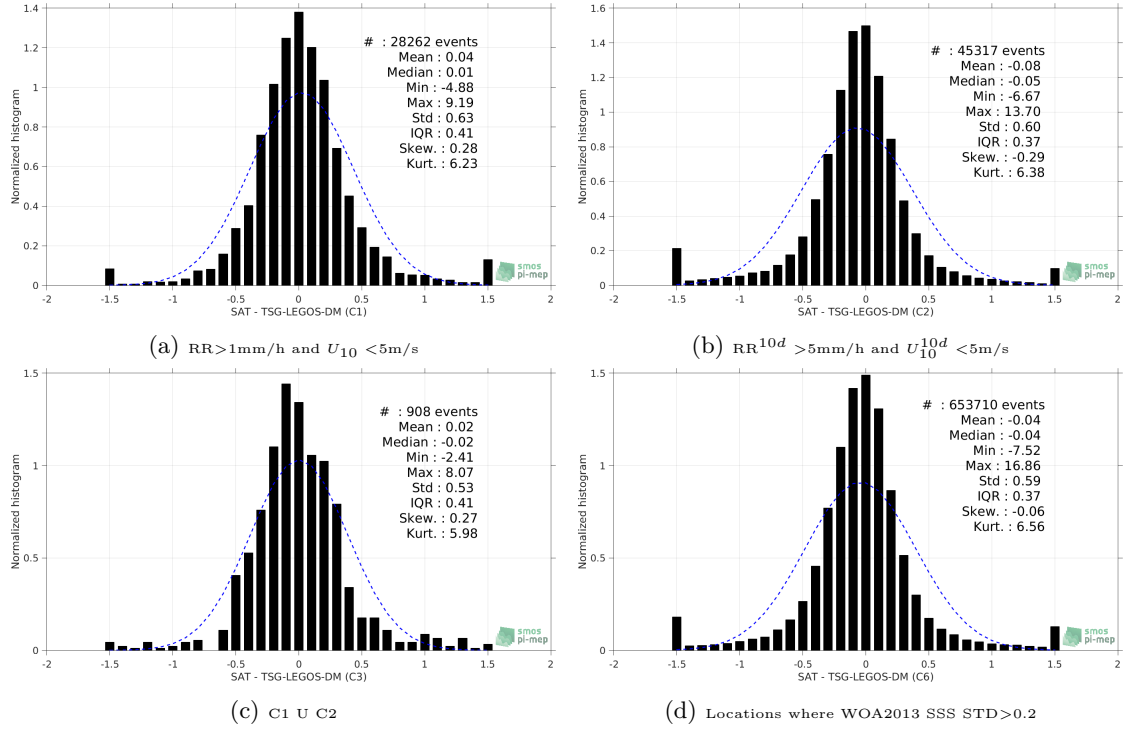
Figure 13: Normalized histogram of \Delta SSS (SMOS-L3-CATDS-CPDC-V3-MONTHLY-25KM - TSG-LEGOS-DM) for 6 different subdatasets corresponding to: RR > 1\text{mm/h} and U_{10} < 5\text{m/s} (a), RR^{10d} > 5\text{mm/h} and U_{10}^{10d} < 5\text{m/s} (b), C1 U C2 (c), Locations where WOA2013 SSS STD > 0.2 (d).
