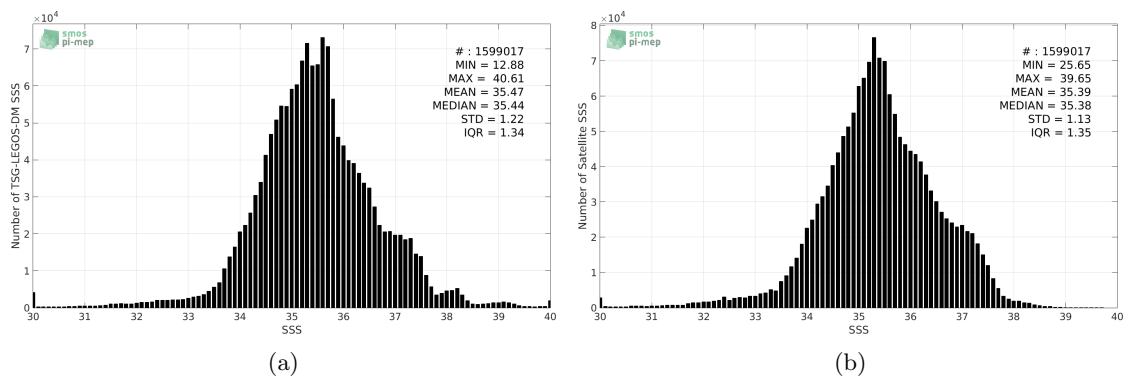
Figure 2: Histograms of SSS from TSG-LEGOS-DM (a) and SMOS-L3-CATDS-CPDC-V3-MONTHLY-25KM (b) considering all match-up pairs per bins of 0.1 over the Global Ocean Pi-MEP region and for the full satellite product period.
