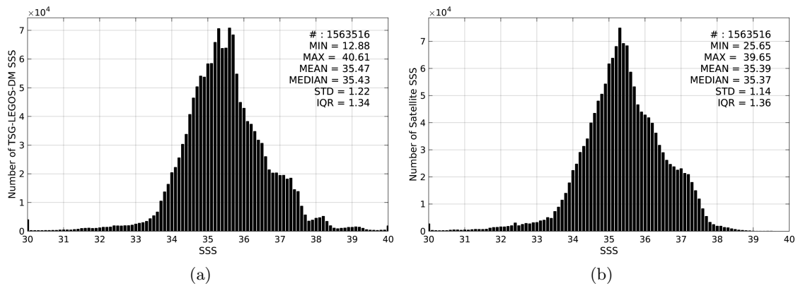
Figure 2: Histograms of SSS from TSG-LEGOS-DM (a) and SMOS-L3-CATDS-CPDC-V3-MONTHLY-25KM (b) considering all match-up pairs per bins of 0.1 over the Global Ocean Pi-MEP region and for the full satellite product period.
