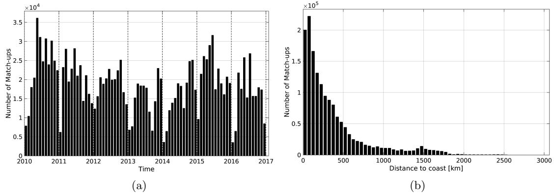
Figure 1: Number of match-ups between TSG-LEGOS-DM and SMOS-L3-CATDS-CPDC-V3-MONTHLY-25KM SSS as a function of time (a) and as function of the distance to coast (b) over the Global Ocean Pi-MEP region and for the full satellite product period.
