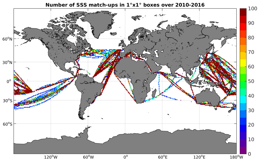
Figure 4: Number of SSS match-ups between TSG-LEGOS-DM SSS and the SMOS-L3-CATDS-CPDC-V3-MONTHLY-25KM SSS product for the Global Ocean Pi-MEP region over 1^\circ \times 1^\circ boxes and for the full satellite product period.
