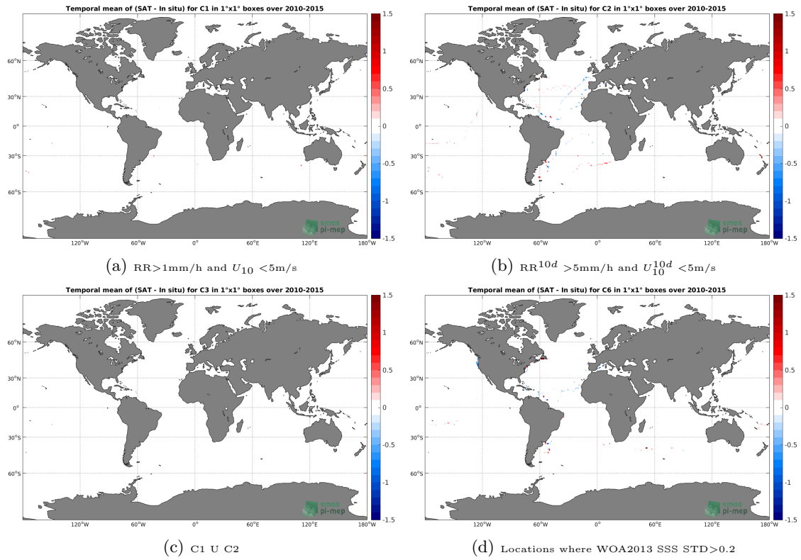
Figure 12: Temporal mean gridded over spatial boxes of size 1^\circ \times 1^\circ of \Delta SSS (SMOS-L3-CATDS-CPDC-V3-MONTHLY-25KM - TSG-GOSUD-Sailing-ship) for 4 different subdatasets corresponding to:RR>1mm/h and U_{10} < 5\text{m/s} (a), RR^{10d} > 5\text{mm/h} and U_{10}^{10d} < 5\text{m/s} (b), C1 U C2 (c),Locations where WOA2013 SSS STD>0.2 (d).
