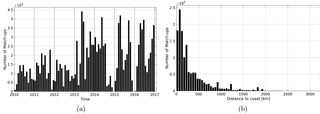
Figure 1: Number of match-ups between TSG-GOSUD-Research-vessel and SMOS-L3-CATDS-CPDC-V3-MONTHLY-25KM SSS as a function of time (a) and as function of the distance to coast (b) over the Global Ocean Pi-MEP region and for the full satellite product period.
