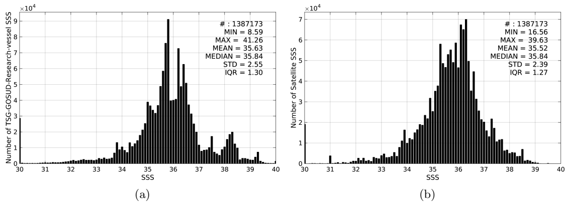
Figure 2: Histograms of SSS from TSG-GOSUD-Research-vessel (a) and SMOS-L3-CATDS-CPDC-V3-MONTHLY-25KM (b) considering all match-up pairs per bins of 0.1 over the Global Ocean Pi-MEP region and for the full satellite product period.
