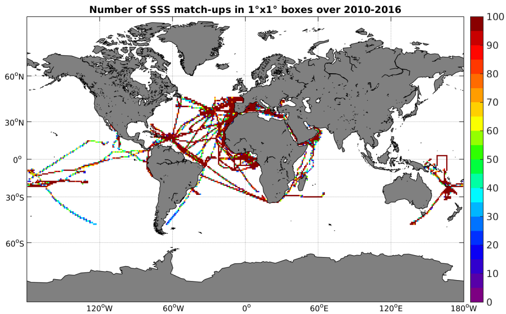
Figure 4: Number of SSS match-ups between TSG-GOSUD-Research-vessel SSS and the SMOS-L3-CATDS-CPDC-V3-MONTHLY-25KM SSS product for the Global Ocean Pi-MEP region over 1^\circ \times 1^\circ boxes and for the full satellite product period.
