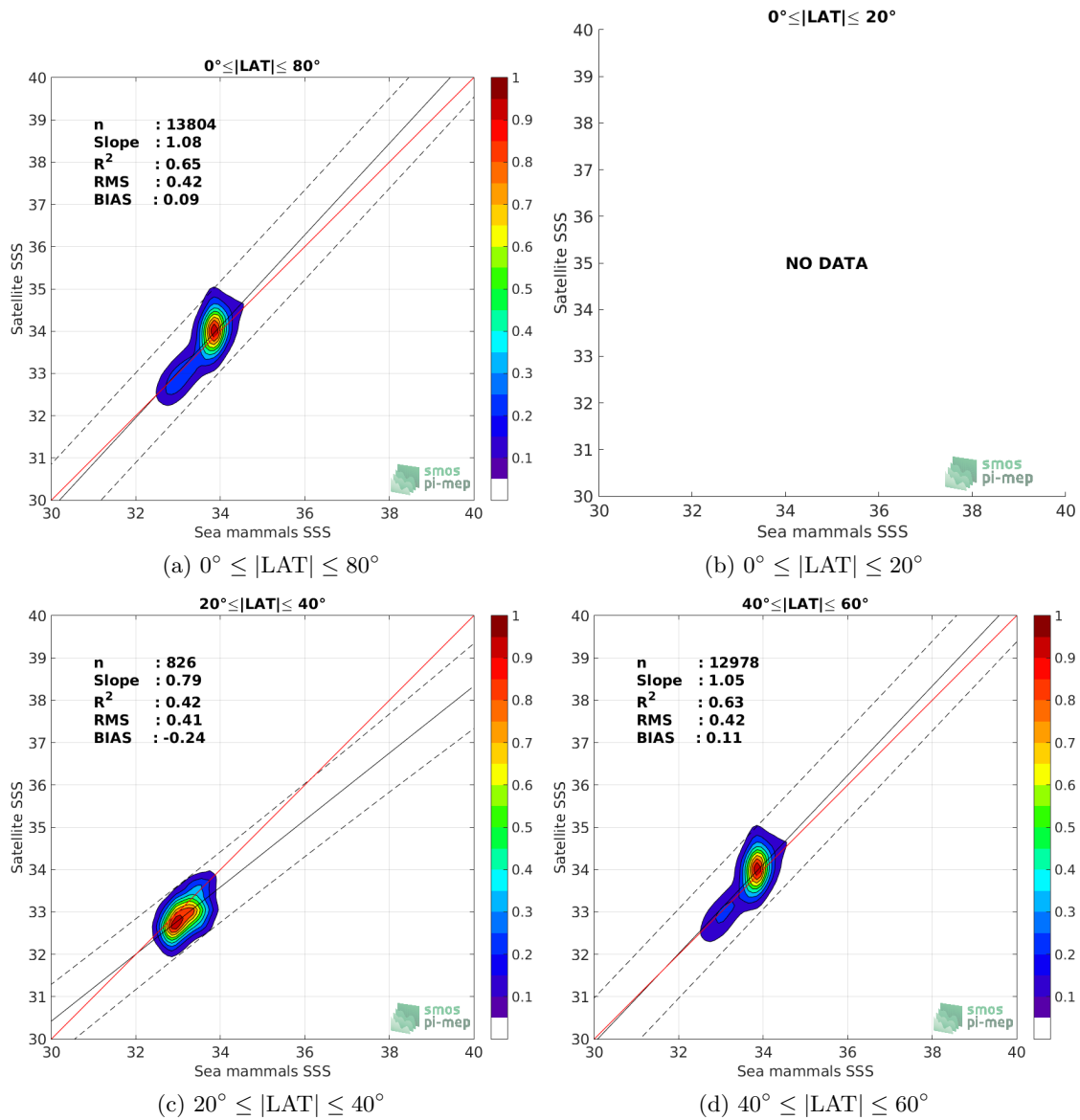
Figure 9: Contour maps of the concentration of SMOS-L3-CATDS-CPDC-V3-MONTHLY-25KM SSS (y-axis) versus Sea mammals SSS (x-axis) at match-up pairs for different latitude bands. For each plot, the red line shows x=y . The black thin and dashed lines indicate a linear fit through the data cloud and the \pm 95\% confidence levels, respectively. The number match-up pairs n , the slope and R^2 coefficient of the linear fit, the root mean square (RMS) and the mean bias between satellite and in situ data are indicated for each latitude band in each plots.
