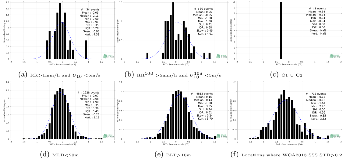
Figure 13: Normalized histogram of \Delta SSS (SMOS-L3-CATDS-CPDC-V3-MONTHLY-25KM - Sea mammals) for 6 different subdatasets corresponding to: RR > 1\text{mm/h} and U_{10} < 5\text{m/s} (a), RR^{10d} > 5\text{mm/h} and U_{10}^{10d} < 5\text{m/s} (b), C1 U C2 (c), MLD < 20\text{m} (d), BLT > 10\text{m} (e), Locations where WOA2013 SSS STD > 0.2 (f).
