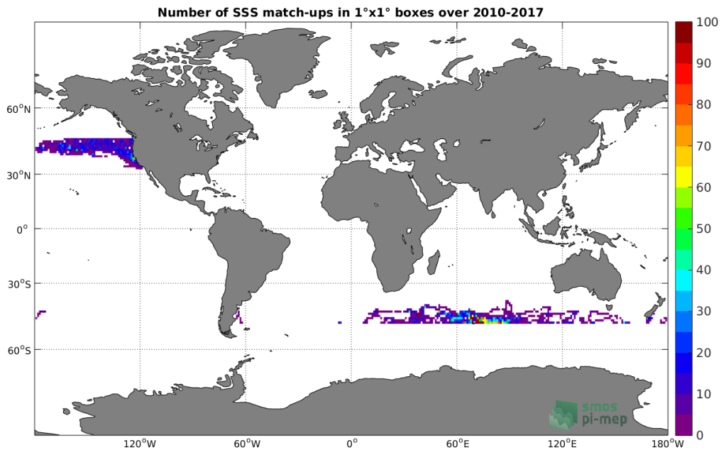
Figure 4: Number of SSS match-ups between Sea mammals SSS and the SMOS-L3-CATDS-CPDC-V3-MONTHLY-25KM SSS product for the Global Ocean Pi-MEP region over 1^\circ \times 1^\circ boxes and for the full satellite product period.
