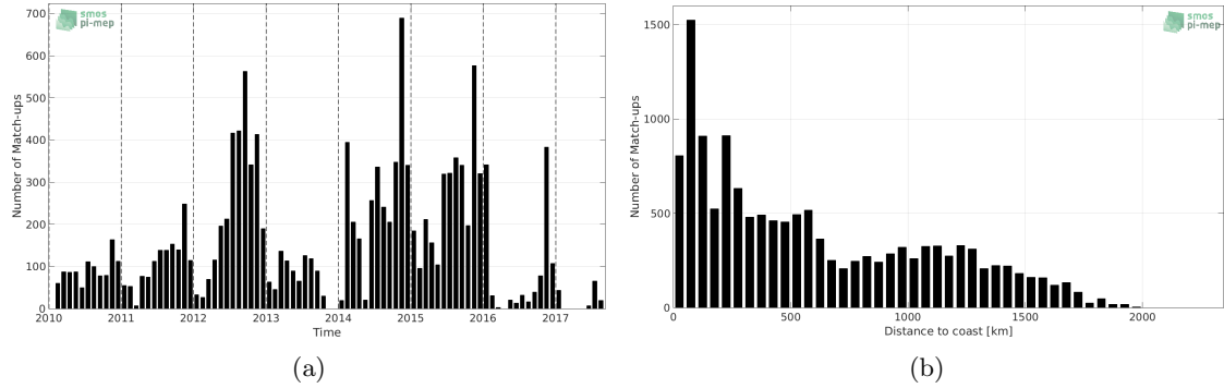
Figure 1: Number of match-ups between Sea mammals and SMOS-L3-CATDS-CPDC-V3-MONTHLY-25KM SSS as a function of time (a) and as function of the distance to coast (b) over the Global Ocean Pi-MEP region and for the full satellite product period.
