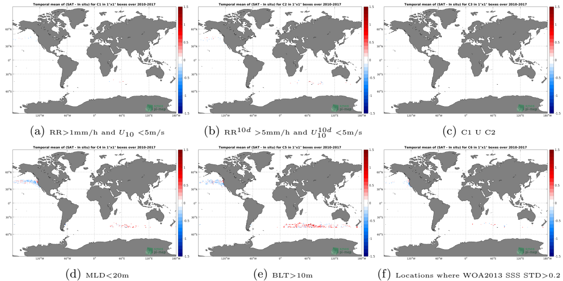
Figure 12: Temporal mean gridded over spatial boxes of size 1^\circ \times 1^\circ of \Delta\text{SSS} (SMOS-L3-CATDS-CPDC-V3-MONTHLY-25KM - Sea mammals) for 6 different subdatasets corresponding to: RR > 1\text{mm/h} and U_{10} < 5\text{m/s} (a), RR^{10d} > 5\text{mm/h} and U_{10}^{10d} < 5\text{m/s} (b), C1 U C2 (c), MLD < 20\text{m} (d), BLT > 10\text{m} (e), Locations where WOA2013 SSS STD > 0.2 (f).
