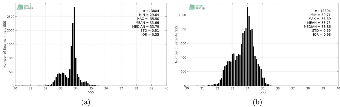
Figure 2: Histograms of SSS from Sea mammals (a) and SMOS-L3-CATDS-CPDC-V3-MONTHLY-25KM (b) considering all match-up pairs per bins of 0.1 over the Global Ocean Pi-MEP region and for the full satellite product period.
