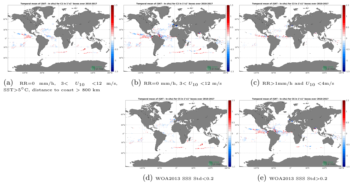
Figure 11: Temporal mean gridded over spatial boxes of size 1^\circ \times 1^\circ of \Delta SSS (SMOS-L3-CATDS-CPDC-V3-MONTHLY-25KM - Surface drifters) for 5 different subdatasets corresponding to:RR=0 mm/h, 3 < U_{10} < 12 m/s, SST > 5^\circ C, distance to coast > 800 km (a), RR=0 mm/h, 3 < U_{10} < 12 m/s (b), RR > 1 mm/h and U_{10} < 4 m/s (c), WOA2013 SSS Std < 0.2 (d), WOA2013 SSS Std > 0.2 (e).
