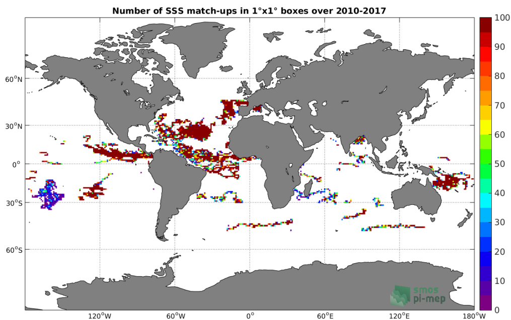
Figure 3: Number of SSS match-ups between Surface drifters SSS and the SMOS-L3-CATDS-CPDC-V3-MONTHLY-25KM SSS product for the Global Ocean Pi-MEP region over 1^\circ \times 1^\circ boxes and for the full satellite product period.
