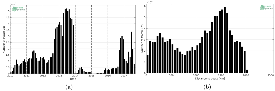
Figure 1: Number of match-ups between Surface drifters and SMOS-L3-CATDS-CPDC-V3-MONTHLY-25KM SSS as a function of time (a) and as function of the distance to coast (b) over the Global Ocean Pi-MEP region and for the full satellite product period.
