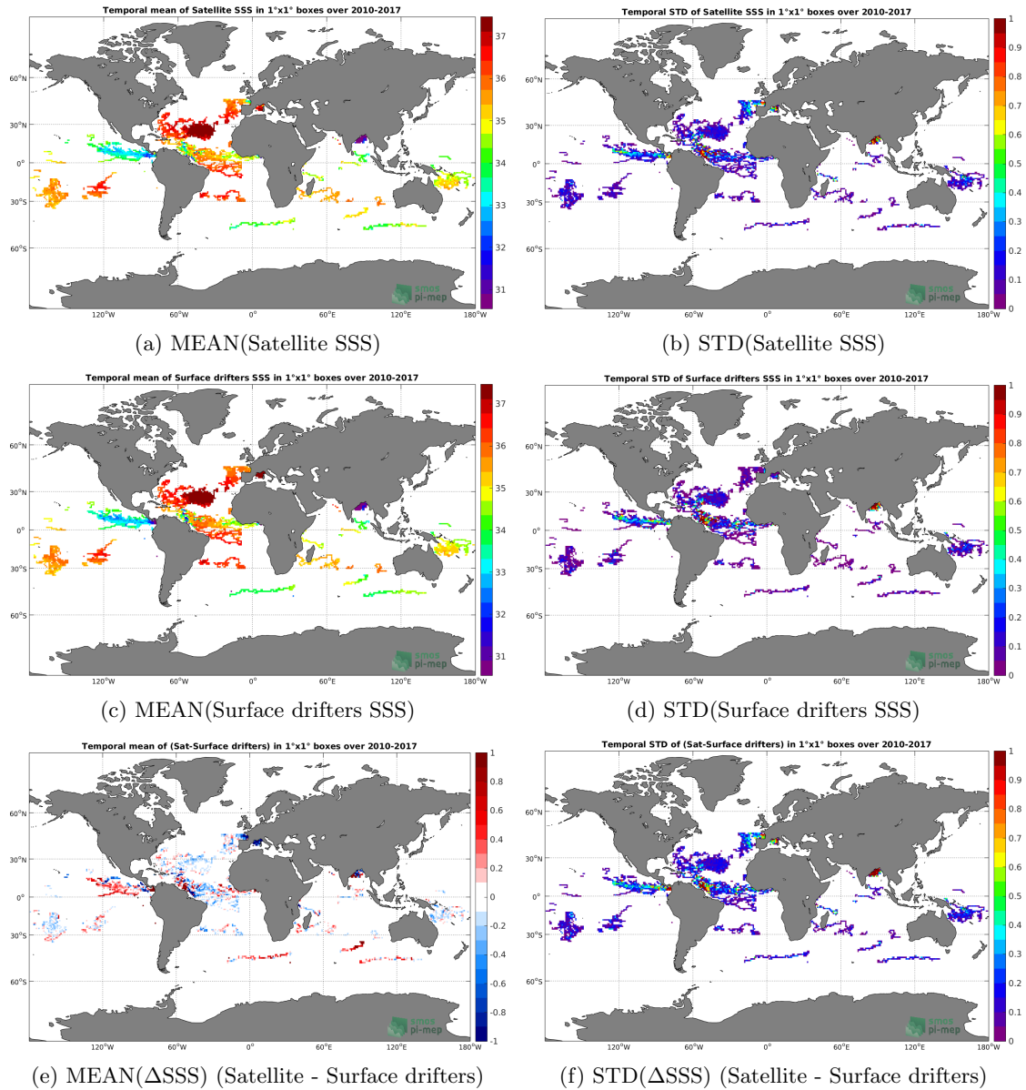
Figure 5: Temporal mean (left) and STD (right) of SSS from SMOS-L3-CATDS-CPDC-V3-MONTHLY-25KM (top), Surface drifters (middle), and of \Delta SSS (Satellite - Surface drifters). Only match-up pairs are used to generate these maps.
