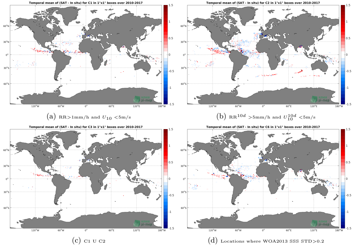
Figure 11: Temporal mean gridded over spatial boxes of size 1^\circ \times 1^\circ of \Delta SSS (SMOS-L3-CATDS-CPDC-V3-MONTHLY-25KM - Surface drifters) for 4 different subdatasets corresponding to: RR > 1\text{mm/h} and U_{10} < 5\text{m/s} (a), RR^{10d} > 5\text{mm/h} and U_{10}^{10d} < 5\text{m/s} (b), C1 U C2 (c), Locations where WOA2013 SSS STD > 0.2 (d).
