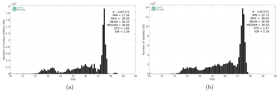
Figure 2: Histograms of SSS from Surface drifters (a) and SMOS-L3-CATDS-CPDC-V3-MONTHLY-25KM (b) considering all match-up pairs per bins of 0.1 over the Global Ocean Pi-MEP region and for the full satellite product period.
