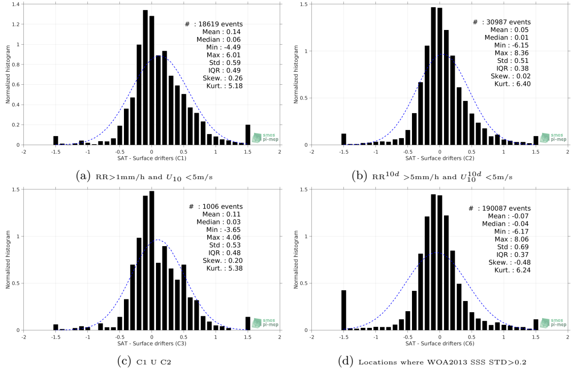
Figure 12: Normalized histogram of \Delta\text{SSS} (SMOS-L3-CATDS-CPDC-V3-MONTHLY-25KM - Surface drifters) for 6 different subdatasets corresponding to: RR > 1\text{mm/h} and U_{10} < 5\text{m/s} (a), RR^{10d} > 5\text{mm/h} and U_{10}^{10d} < 5\text{m/s} (b), C1 \cup C2 (c), Locations where WOA2013 SSS STD > 0.2 (d).
