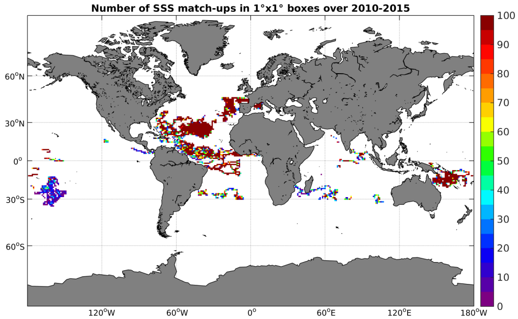
Figure 3: Number of SSS match-ups between Surface drifters SSS and the SMOS-L3-CATDS-CPDC-V3-MONTHLY-25KM SSS product for the Global Ocean Pi-MEP region over 1°x1° boxes and for the full satellite product period.
