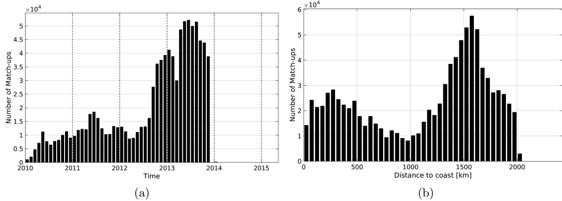
Figure 1: Number of match-ups between Surface drifters and SMOS-L3-CATDS-CPDC-V3-MONTHLY-25KM SSS as a function of time (a) and as function of the distance to coast (b) over the Global Ocean Pi-MEP region and for the full satellite product period.
