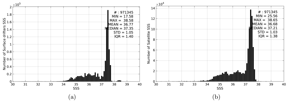
Figure 2: Histograms of SSS from Surface drifters (a) and SMOS-L3-CATDS-CPDC-V3-MONTHLY-25KM (b) considering all match-up pairs per bins of 0.1 over the Global Ocean Pi-MEP region and for the full satellite product period.
