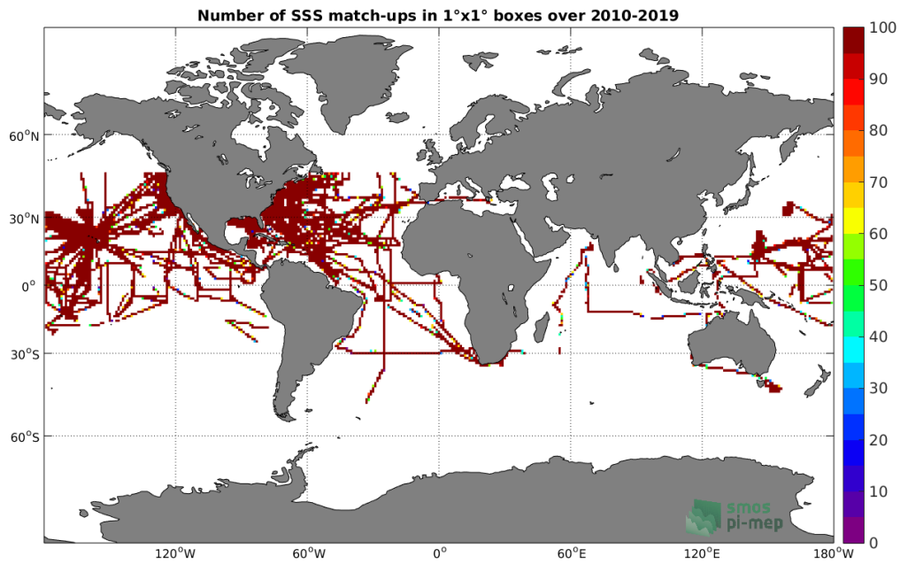
Figure 4: Number of SSS match-ups between TSG-SAMOS SSS and the SMOS-L3-CATDS-CPDC-V3-10DAYS-25KM SSS product for the Global Ocean Pi-MEP region over 1^\circ \times 1^\circ boxes and for the full satellite product period.
