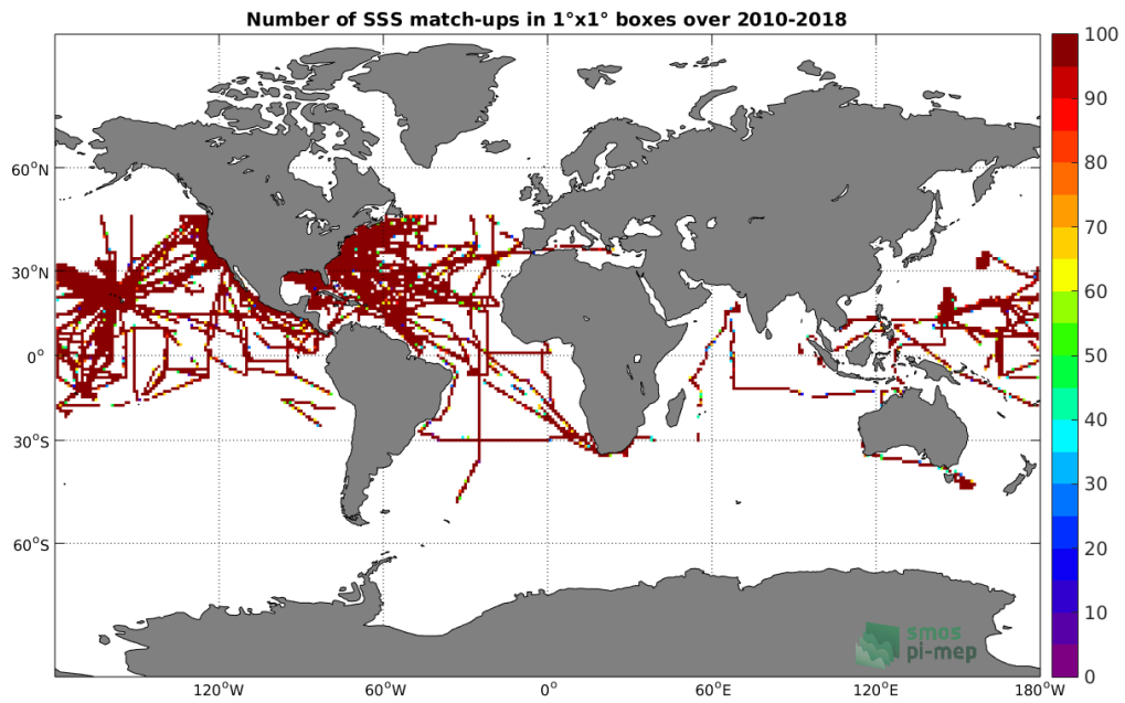
Figure 4: Number of SSS match-ups between TSG-SAMOS SSS and the SMOS-L3-CATDS-CPDC-V3-10DAYS-25KM SSS product for the Global Ocean Pi-MEP region over 1°x1° boxes and for the full satellite product period.
