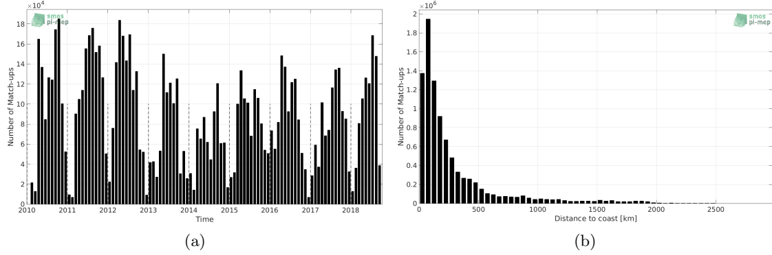
Figure 1: Number of match-ups between TSG-SAMOS and SMOS-L3-CATDS-CPDC-V3-10DAYS-25KM SSS as a function of time (a) and as function of the distance to coast (b) over the Global Ocean Pi-MEP region and for the full satellite product period.
