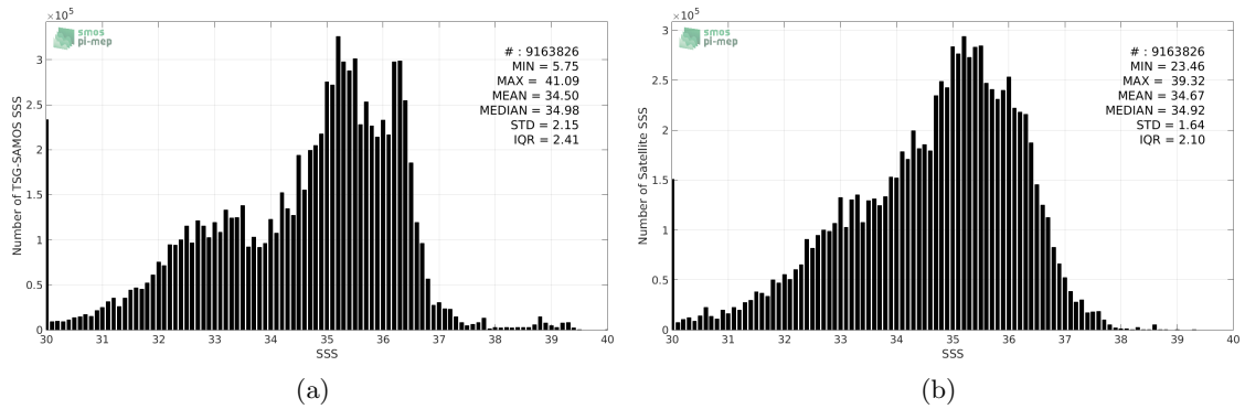
Figure 2: Histograms of SSS from TSG-SAMOS (a) and SMOS-L3-CATDS-CPDC-V3-10DAYS-25KM (b) considering all match-up pairs per bins of 0.1 over the Global Ocean Pi-MEP region and for the full satellite product period.
