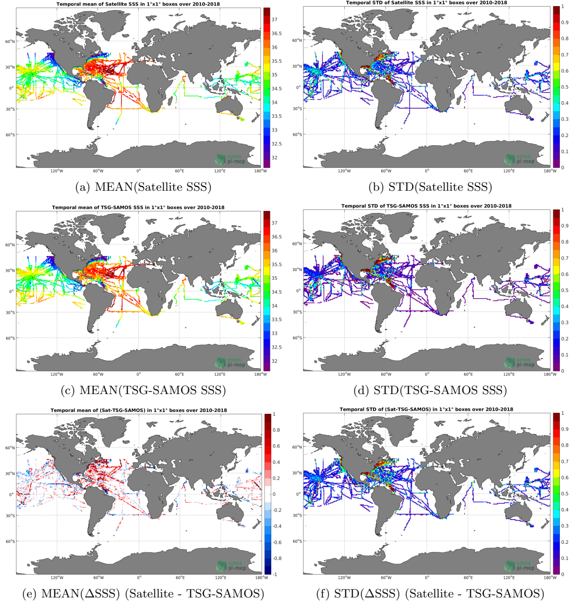
Figure 6: Temporal mean (left) and STD (right) of SSS from SMOS-L3-CATDS-CPDC-V3-10DAYS-25KM (top), TSG-SAMOS (middle), and of \Delta SSS (Satellite - TSG-SAMOS). Only match-up pairs are used to generate these maps.
