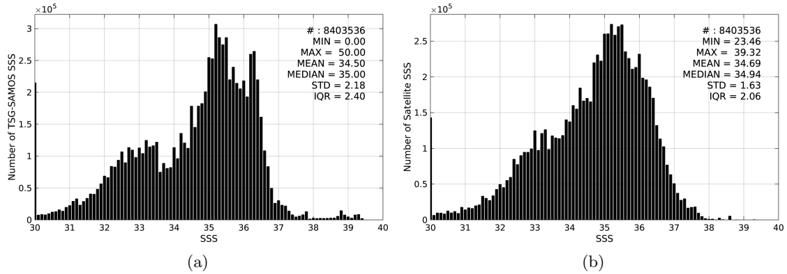
Figure 2: Histograms of SSS from TSG-SAMOS (a) and SMOS-L3-CATDS-CPDC-V3-10DAYS-25KM (b) considering all match-up pairs per bins of 0.1 over the Global Ocean Pi-MEP region and for the full satellite product period.
