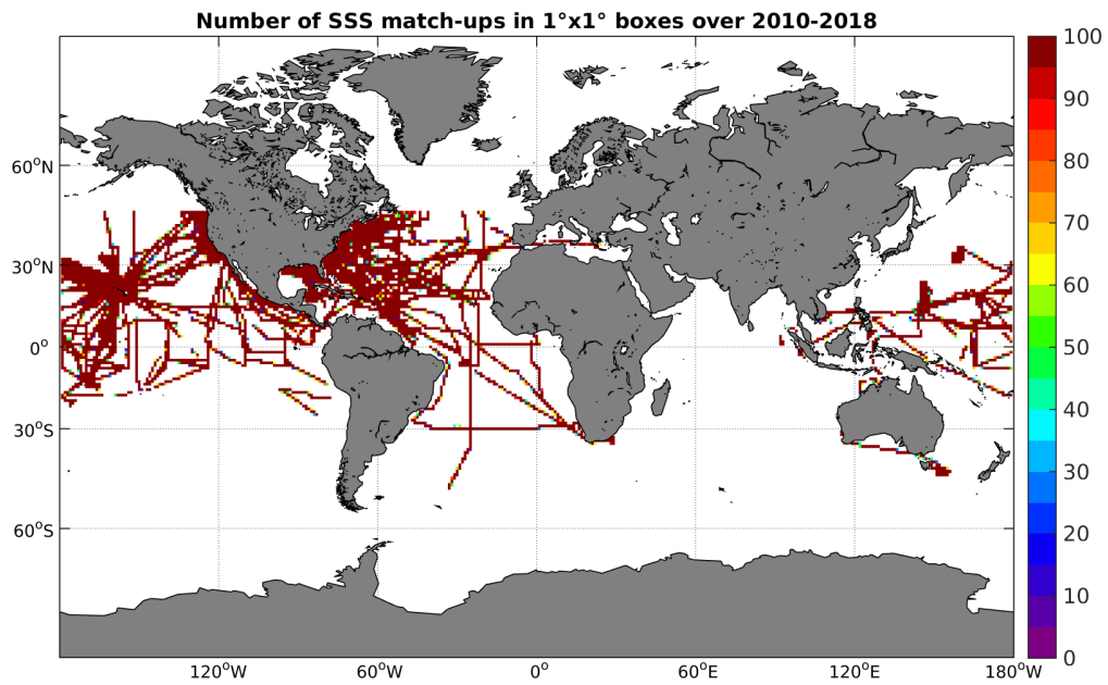
Figure 4: Number of SSS match-ups between TSG-SAMOS SSS and the SMOS-L3-CATDS-CPDC-V3-10DAYS-25KM SSS product for the Global Ocean Pi-MEP region over 1°x1° boxes and for the full satellite product period.
