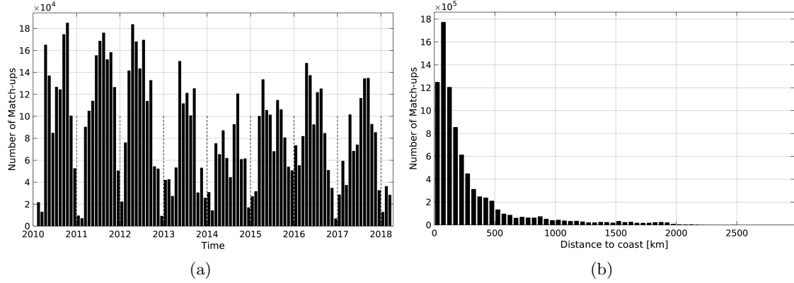
Figure 1: Number of match-ups between TSG-SAMOS and SMOS-L3-CATDS-CPDC-V3-10DAYS-25KM SSS as a function of time (a) and as function of the distance to coast (b) over the Global Ocean Pi-MEP region and for the full satellite product period.
