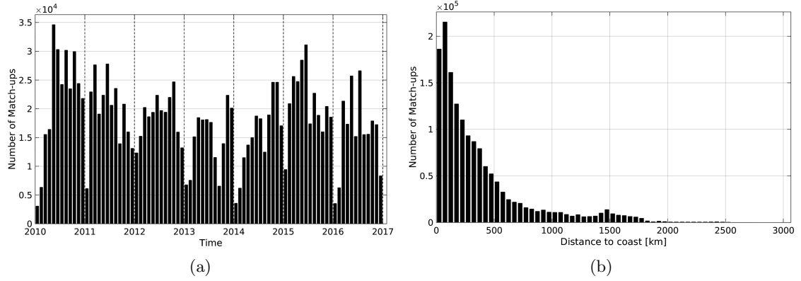
Figure 1: Number of match-ups between TSG-LEGOS-DM and SMOS-L3-CATDS-CPDC-V3-10DAYS-25KM SSS as a function of time (a) and as function of the distance to coast (b) over the Global Ocean Pi-MEP region and for the full satellite product period.
