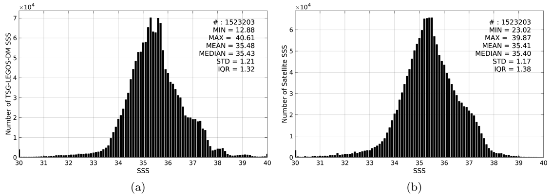
Figure 2: Histograms of SSS from TSG-LEGOS-DM (a) and SMOS-L3-CATDS-CPDC-V3-10DAYS-25KM (b) considering all match-up pairs per bins of 0.1 over the Global Ocean Pi-MEP region and for the full satellite product period.
