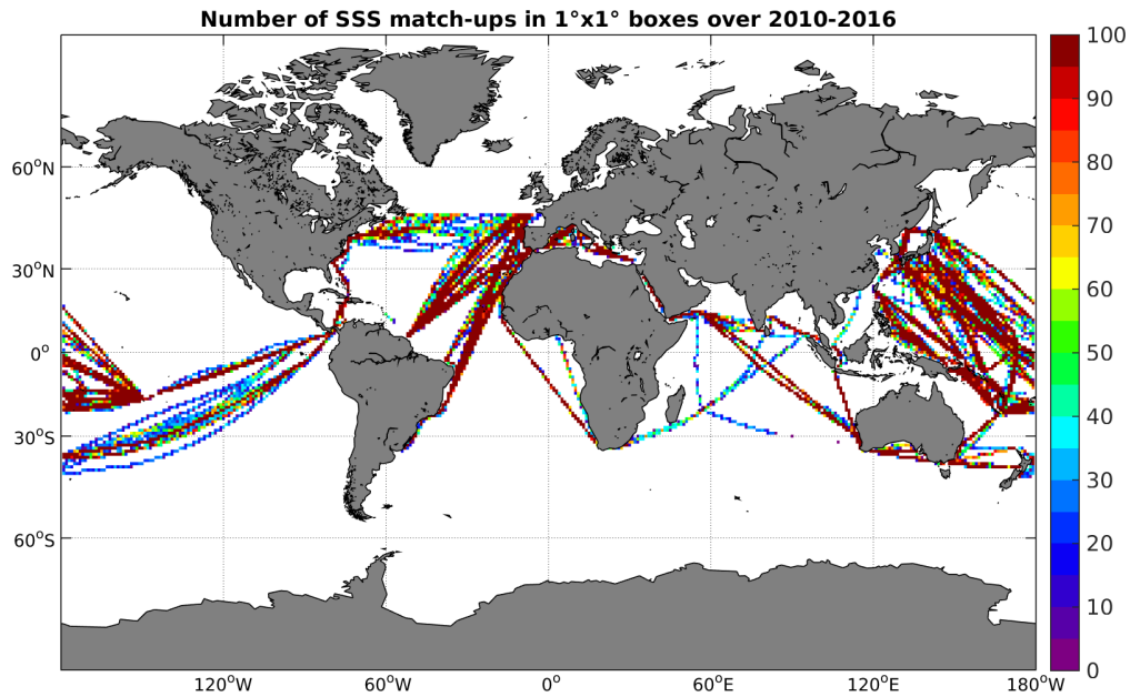
Figure 4: Number of SSS match-ups between TSG-LEGOS-DM SSS and the SMOS-L3-CATDS-CPDC-V3-10DAYS-25KM SSS product for the Global Ocean Pi-MEP region over 1^\circ \times 1^\circ boxes and for the full satellite product period.
