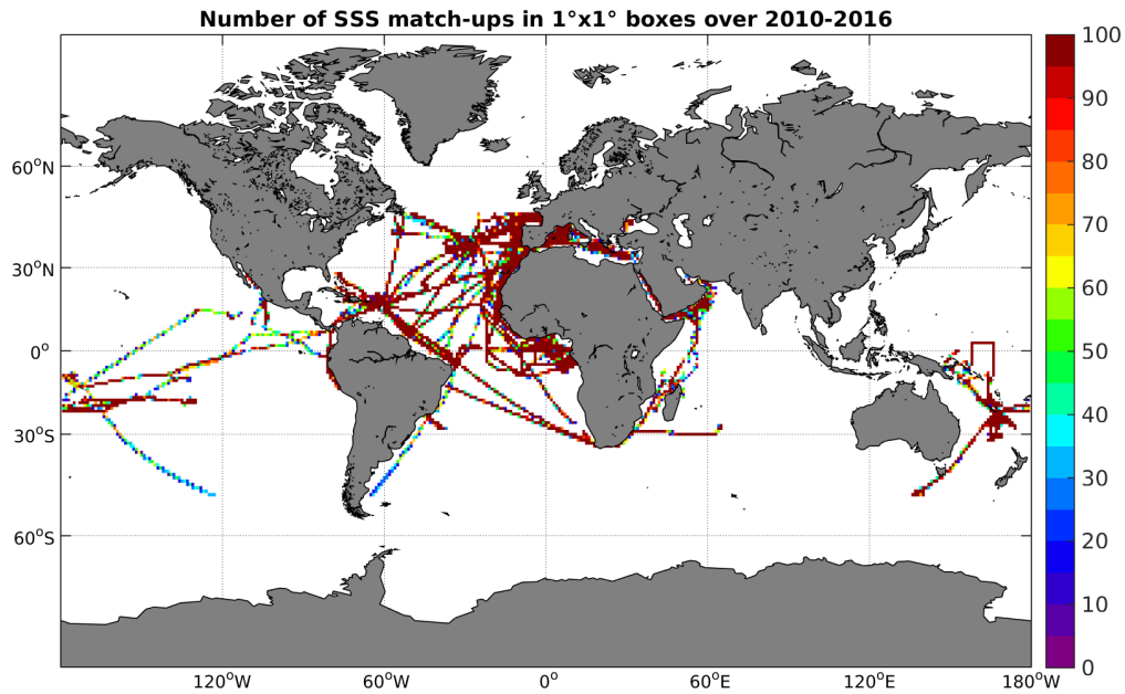
Figure 4: Number of SSS match-ups between TSG-GOSUD-Research-vessel SSS and the SMOS-L3-CATDS-CPDC-V3-10DAYS-25KM SSS product for the Global Ocean Pi-MEP region over 1^\circ \times 1^\circ boxes and for the full satellite product period.
