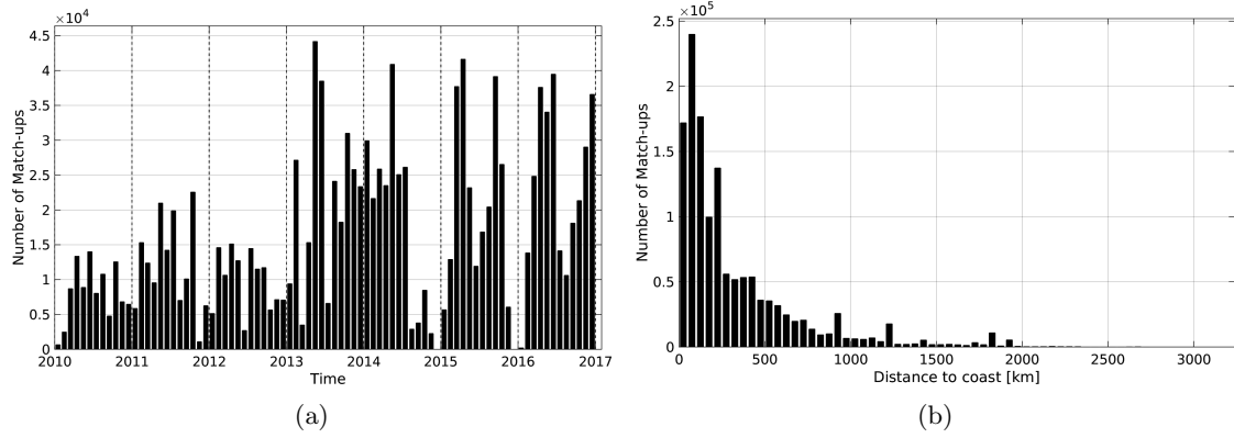
Figure 1: Number of match-ups between TSG-GOSUD-Research-vessel and SMOS-L3-CATDS-CPDC-V3-10DAYS-25KM SSS as a function of time (a) and as function of the distance to coast (b) over the Global Ocean Pi-MEP region and for the full satellite product period.
