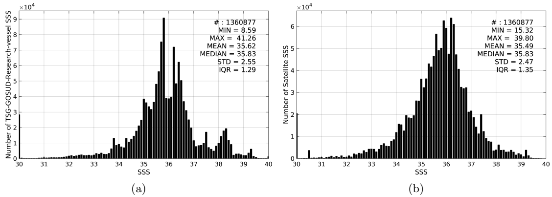
Figure 2: Histograms of SSS from TSG-GOSUD-Research-vessel (a) and SMOS-L3-CATDS-CPDC-V3-10DAYS-25KM (b) considering all match-up pairs per bins of 0.1 over the Global Ocean Pi-MEP region and for the full satellite product period.
