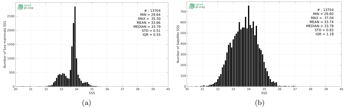
Figure 2: Histograms of SSS from Sea mammals (a) and SMOS-L3-CATDS-CPDC-V3-10DAYS-25KM (b) considering all match-up pairs per bins of 0.1 over the Global Ocean Pi-MEP region and for the full satellite product period.
