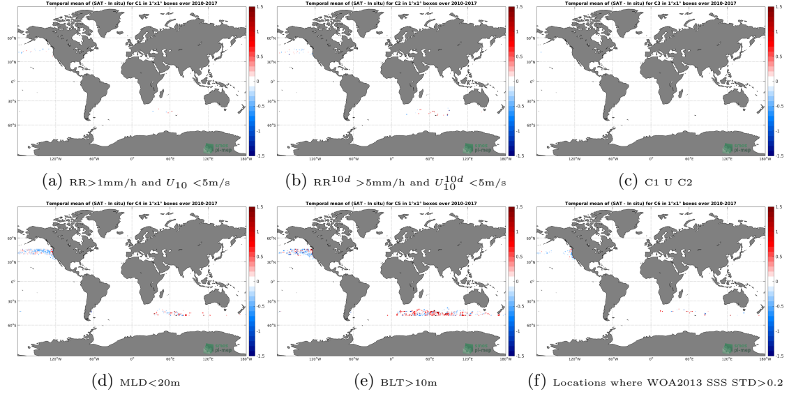
Figure 12: Temporal mean gridded over spatial boxes of size 1^\circ \times 1^\circ of \Delta\text{SSS} (SMOS-L3-CATDS-CPDC-V3-10DAYS-25KM - Sea mammals) for 6 different subdatasets corresponding to: RR > 1\text{mm/h} and U_{10} < 5\text{m/s} (a), RR^{10d} > 5\text{mm/h} and U_{10}^{10d} < 5\text{m/s} (b), C1 U C2 (c), MLD < 20\text{m} (d), BLT > 10\text{m} (e), Locations where WOA2013 SSS STD > 0.2 (f).
