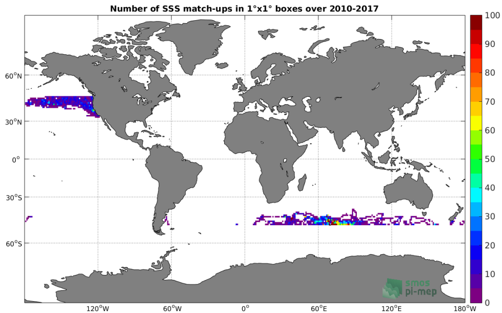
Figure 4: Number of SSS match-ups between Sea mammals SSS and the SMOS-L3-CATDS-CPDC-V3-10DAYS-25KM SSS product for the Global Ocean Pi-MEP region over 1^\circ \times 1^\circ boxes and for the full satellite product period.
