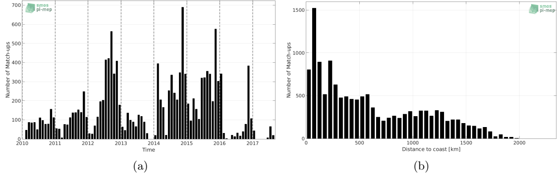
Figure 1: Number of match-ups between Sea mammals and SMOS-L3-CATDS-CPDC-V3-10DAYS-25KM SSS as a function of time (a) and as function of the distance to coast (b) over the Global Ocean Pi-MEP region and for the full satellite product period.
