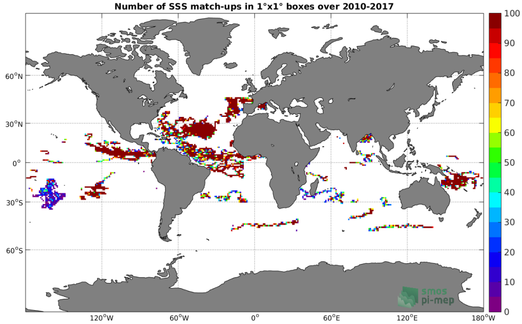
Figure 3: Number of SSS match-ups between Surface drifters SSS and the SMOS-L3-CATDS-CPDC-V3-10DAYS-25KM SSS product for the Global Ocean Pi-MEP region over 1°x1° boxes and for the full satellite product period.
