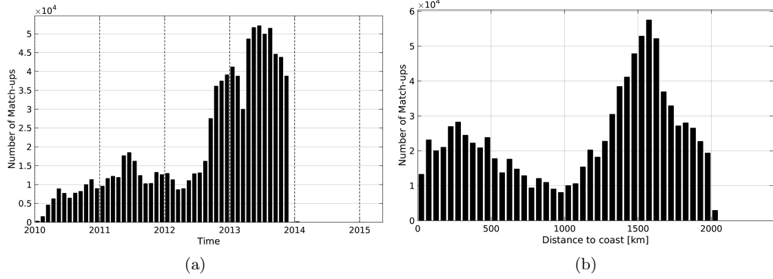
Figure 1: Number of match-ups between Surface drifters and SMOS-L3-CATDS-CPDC-V3-10DAYS-25KM SSS as a function of time (a) and as function of the distance to coast (b) over the Global Ocean Pi-MEP region and for the full satellite product period.
