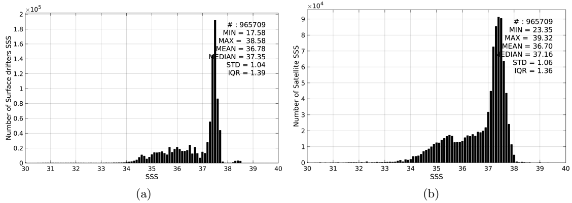
Figure 2: Histograms of SSS from Surface drifters (a) and SMOS-L3-CATDS-CPDC-V3-10DAYS-25KM (b) considering all match-up pairs per bins of 0.1 over the Global Ocean Pi-MEP region and for the full satellite product period.
