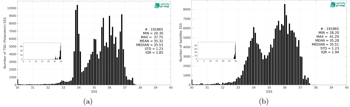
Figure 3: Histograms of SSS from TSG (Polarstern) (a) and SMOS SSS L3 v2 - 9-Days (BEC) (b) considering all match-up pairs per bins of 0.1 over the Global Ocean Pi-MEP region and for the full satellite product period.
