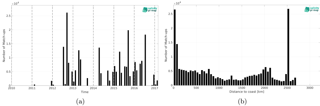
Figure 2: Number of match-ups between TSG (NCEI-0170743) and SMOS SSS L3 v2 - 9-Days (BEC) SSS as a function of time (a) and as function of the distance to coast (b) over the Global Ocean Pi-MEP region and for the full satellite product period.
