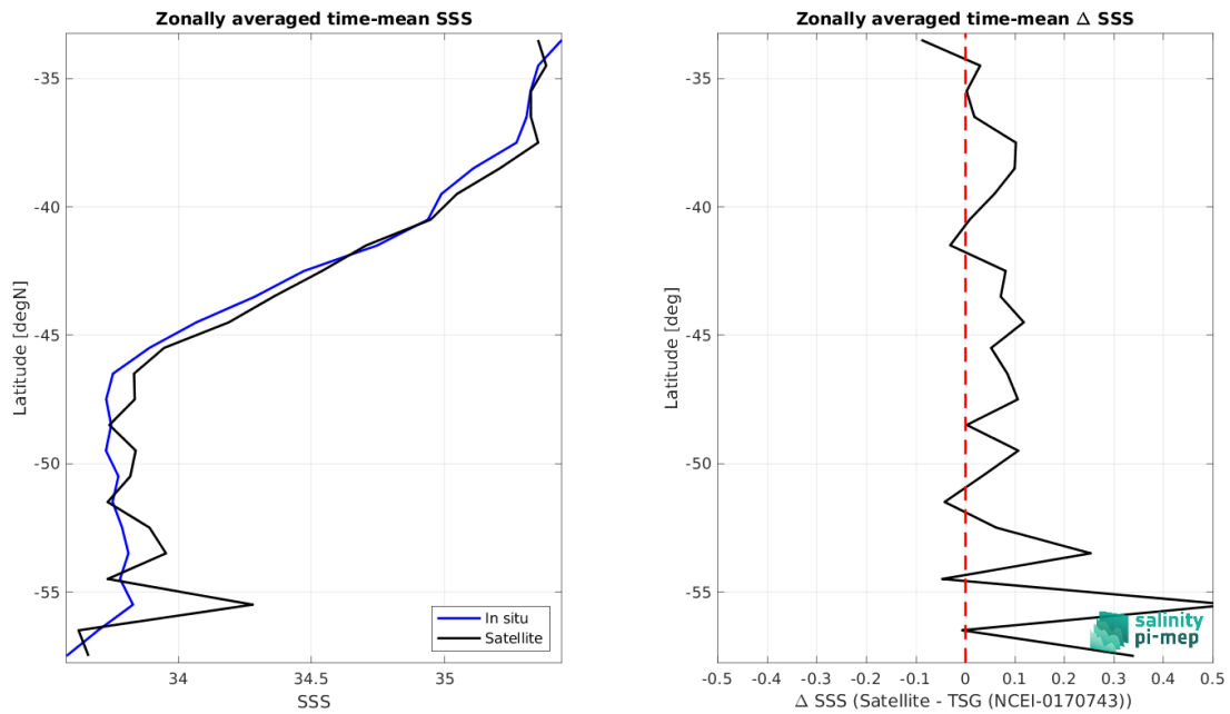
Figure 9: Left panel: Zonal mean SSS from SMOS SSS L3 v2 - 9-Days (BEC) satellite product (black) and from TSG (NCEI-0170743) (blue). Right panel: Zonal mean of \Delta SSS (Satellite - TSG (NCEI-0170743)) for all the collected Pi-MEP match-up pairs estimated over the full satellite product period.
