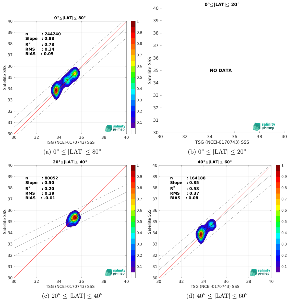
Figure 10: Contour maps of the concentration of SMOS SSS L3 v2 - 9-Days (BEC) SSS (y-axis) versus TSG (NCEI-0170743) SSS (x-axis) at match-up pairs for different latitude bands. For each plot, the red line shows x=y . The black thin and dashed lines indicate a linear fit through the data cloud and the \pm 95\% confidence levels, respectively. The number match-up pairs n , the slope and R^2 coefficient of the linear fit, the root mean square (RMS) and the mean bias between satellite and in situ data are indicated for each latitude band in each plots.
