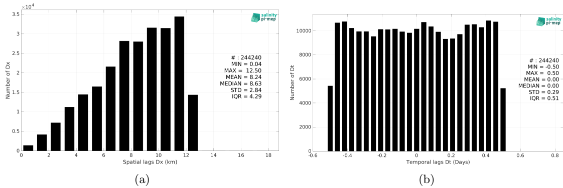
Figure 6: Histograms of the spatial (a) and temporal (b) lags between the location/time of the TSG (NCEI-0170743) measurement and the date of the corresponding SMOS SSS L3 v2 - 9-Days (BEC) SSS pixel.
