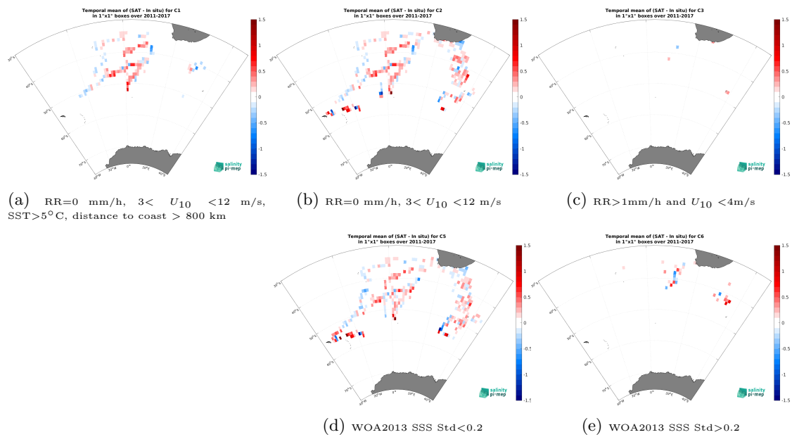
Figure 14: Temporal mean gridded over spatial boxes of size 1^\circ \times 1^\circ of \Delta SSS (SMOS SSS L3 v2 - 9-Days (BEC) - TSG (NCEI-0170743)) for 5 different subdatasets corresponding to:RR=0 mm/h, 3 < U_{10} < 12 m/s, SST >5^\circ\text{C} , distance to coast > 800 km (a), RR=0 mm/h, 3 < U_{10} < 12 m/s (b), RR >1 mm/h and U_{10} < 4 m/s (c), WOA2013 SSS Std <0.2 (d), WOA2013 SSS Std >0.2 (e).
