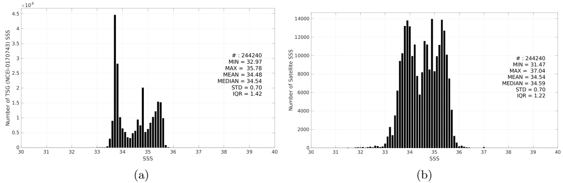
Figure 3: Histograms of SSS from TSG (NCEI-0170743) (a) and SMOS SSS L3 v2 - 9-Days (BEC) (b) considering all match-up pairs per bins of 0.1 over the Global Ocean Pi-MEP region and for the full satellite product period.
