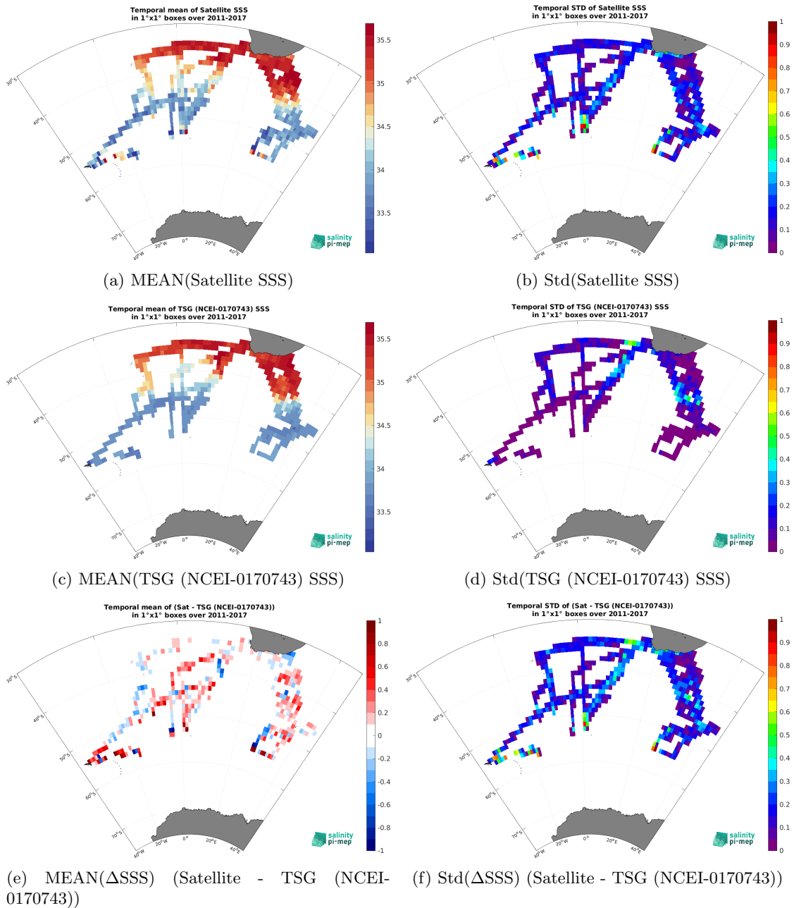
Figure 7: Temporal mean (left) and Std (right) of SSS from SMOS SSS L3 v2 - 9-Days (BEC) (top), TSG (NCEI-0170743) (middle), and of \Delta SSS (Satellite - TSG (NCEI-0170743)). Only match-up pairs are used to generate these maps.
