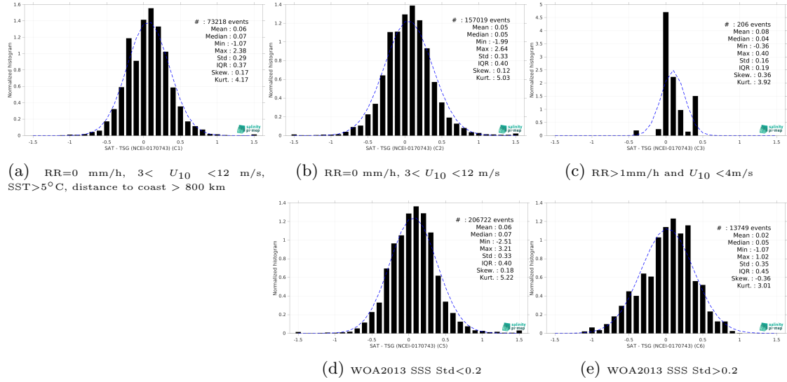
Figure 15: Normalized histogram of \Delta SSS (SMOS SSS L3 v2 - 9-Days (BEC) - TSG (NCEI-0170743)) for 5 different subdatasets corresponding to: RR=0 mm/h, 3 < U_{10} < 12 m/s, SST>5°C, distance to coast > 800 km (a), RR=0 mm/h, 3 < U_{10} < 12 m/s (b), RR>1mm/h and U_{10} < 4 m/s (c), WOA2013 SSS Std<0.2 (d), WOA2013 SSS Std>0.2 (e).
