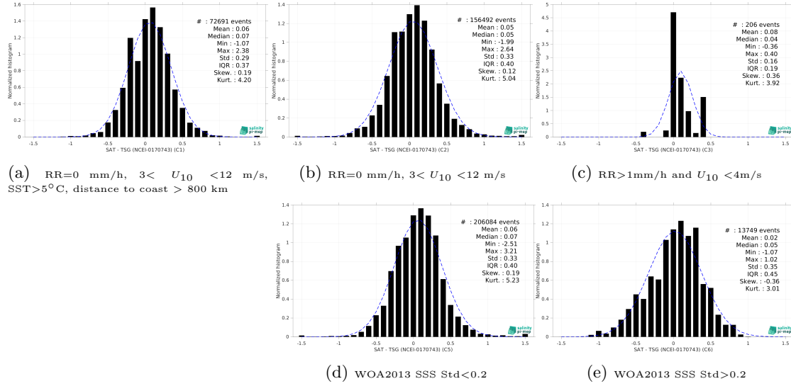
Figure 15: Normalized histogram of \Delta SSS (SMOS SSS L3 v2 - 9-Days (BEC) - TSG (NCEI-0170743)) for 5 different subdatasets corresponding to: RR=0 mm/h, 3 < U_{10} < 12 m/s, SST > 5°C, distance to coast > 800 km (a), RR=0 mm/h, 3 < U_{10} < 12 m/s (b), RR > 1mm/h and U_{10} < 4 m/s (c), WOA2013 SSS Std < 0.2 (d), WOA2013 SSS Std > 0.2 (e).
