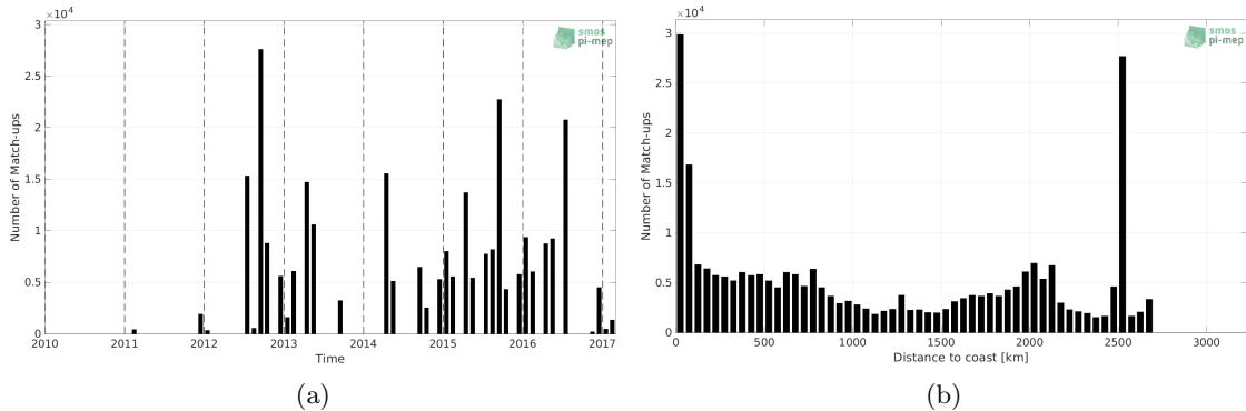
Figure 1: Number of match-ups between TSG (NCEI-0170743) and SMOS SSS L3 v2 - 9-Days (BEC) SSS as a function of time (a) and as function of the distance to coast (b) over the Global Ocean Pi-MEP region and for the full satellite product period.
