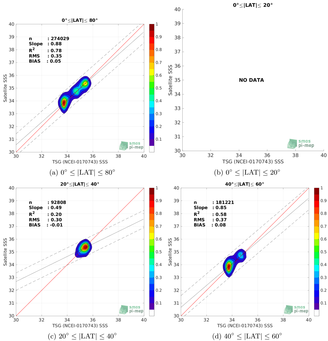
Figure 9: Contour maps of the concentration of SMOS SSS L3 v2 - 9-Days (BEC) SSS (y-axis) versus TSG (NCEI-0170743) SSS (x-axis) at match-up pairs for different latitude bands. For each plot, the red line shows x=y . The black thin and dashed lines indicate a linear fit through the data cloud and the \pm 95\% confidence levels, respectively. The number match-up pairs n , the slope and R^2 coefficient of the linear fit, the root mean square (RMS) and the mean bias between satellite and in situ data are indicated for each latitude band in each plots.
