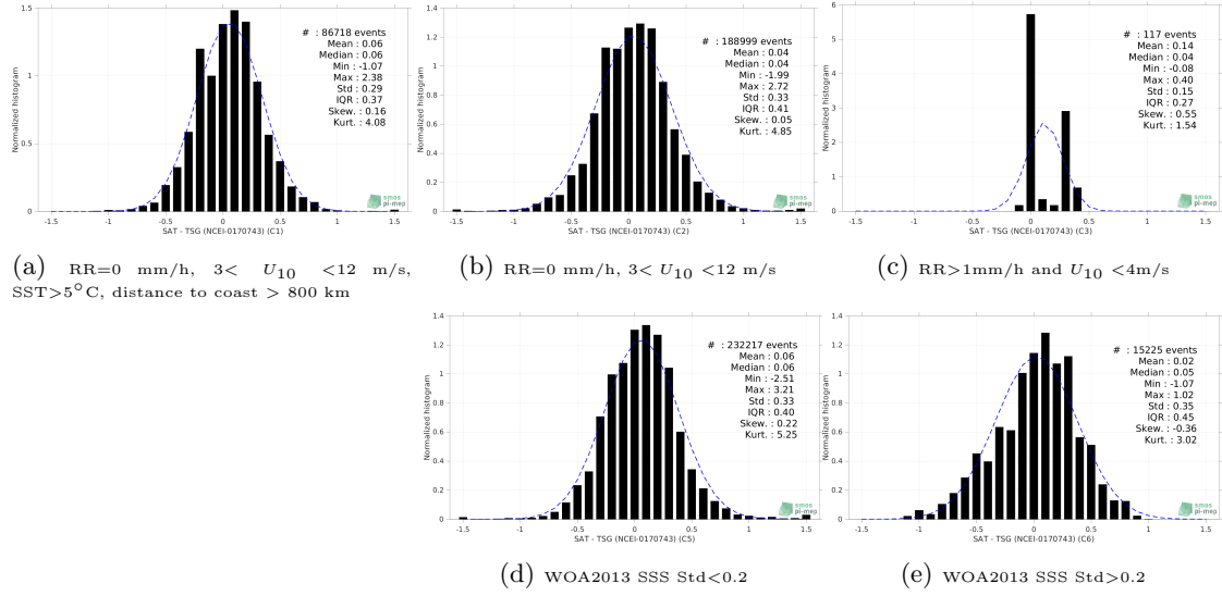
Figure 13: Normalized histogram of \Delta SSS (SMOS SSS L3 v2 - 9-Days (BEC) - TSG (NCEI-0170743)) for 5 different subdatasets corresponding to: RR=0 mm/h, 3 < U_{10} < 12 m/s, SST > 5°C, distance to coast > 800 km (a), RR=0 mm/h, 3 < U_{10} < 12 m/s (b), RR > 1mm/h and U_{10} < 4 m/s (c), WOA2013 SSS Std < 0.2 (d), WOA2013 SSS Std > 0.2 (e).
