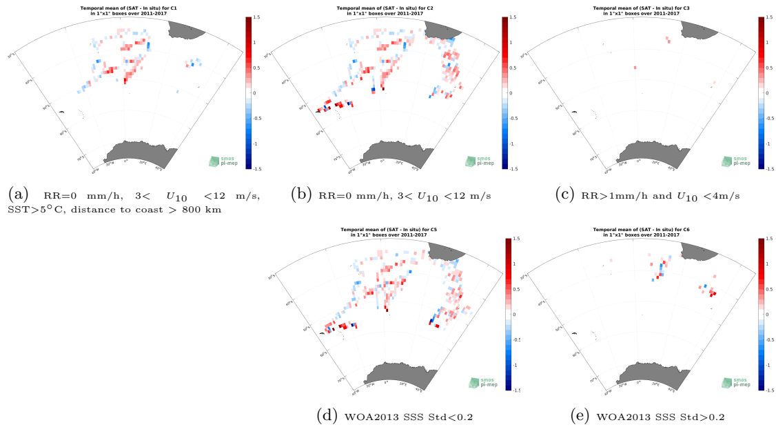
Figure 12: Temporal mean gridded over spatial boxes of size 1^\circ \times 1^\circ of \Delta SSS (SMOS SSS L3 v2 - 9-Days (BEC) - TSG (NCEI-0170743)) for 5 different subdatasets corresponding to:RR=0 mm/h, 3 < U_{10} < 12 m/s, SST > 5^\circ\text{C} , distance to coast > 800 km (a), RR=0 mm/h, 3 < U_{10} < 12 m/s (b), RR > 1 mm/h and U_{10} < 4 m/s (c), WOA2013 SSS Std < 0.2 (d), WOA2013 SSS Std > 0.2 (e).
