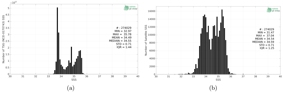
Figure 2: Histograms of SSS from TSG (NCEI-0170743) (a) and SMOS SSS L3 v2 - 9-Days (BEC) (b) considering all match-up pairs per bins of 0.1 over the Global Ocean Pi-MEP region and for the full satellite product period.
