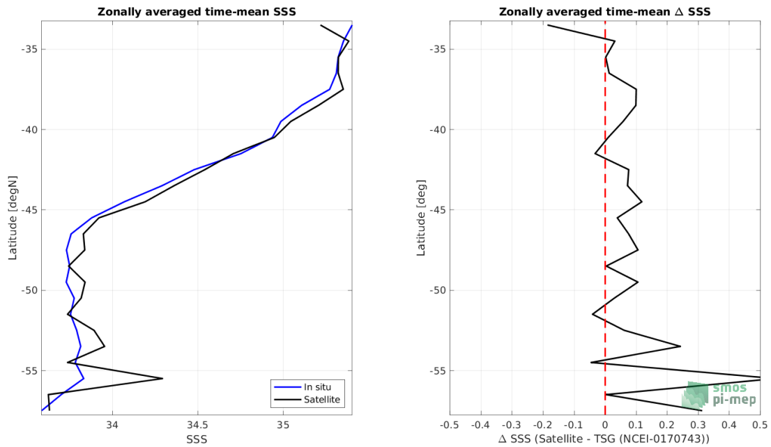
Figure 8: Left panel: Zonal mean SSS from SMOS SSS L3 v2 - 9-Days (BEC) satellite product (black) and from TSG (NCEI-0170743) (blue). Right panel: Zonal mean of \Delta SSS (Satellite - TSG (NCEI-0170743)) for all the collected Pi-MEP match-up pairs estimated over the full satellite product period.
