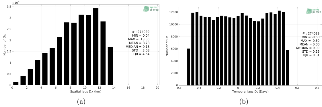
Figure 5: Histograms of the spatial (a) and temporal (b) lags between the location/time of the TSG (NCEI-0170743) measurement and the date of the corresponding SMOS SSS L3 v2 - 9-Days (BEC) SSS pixel.
