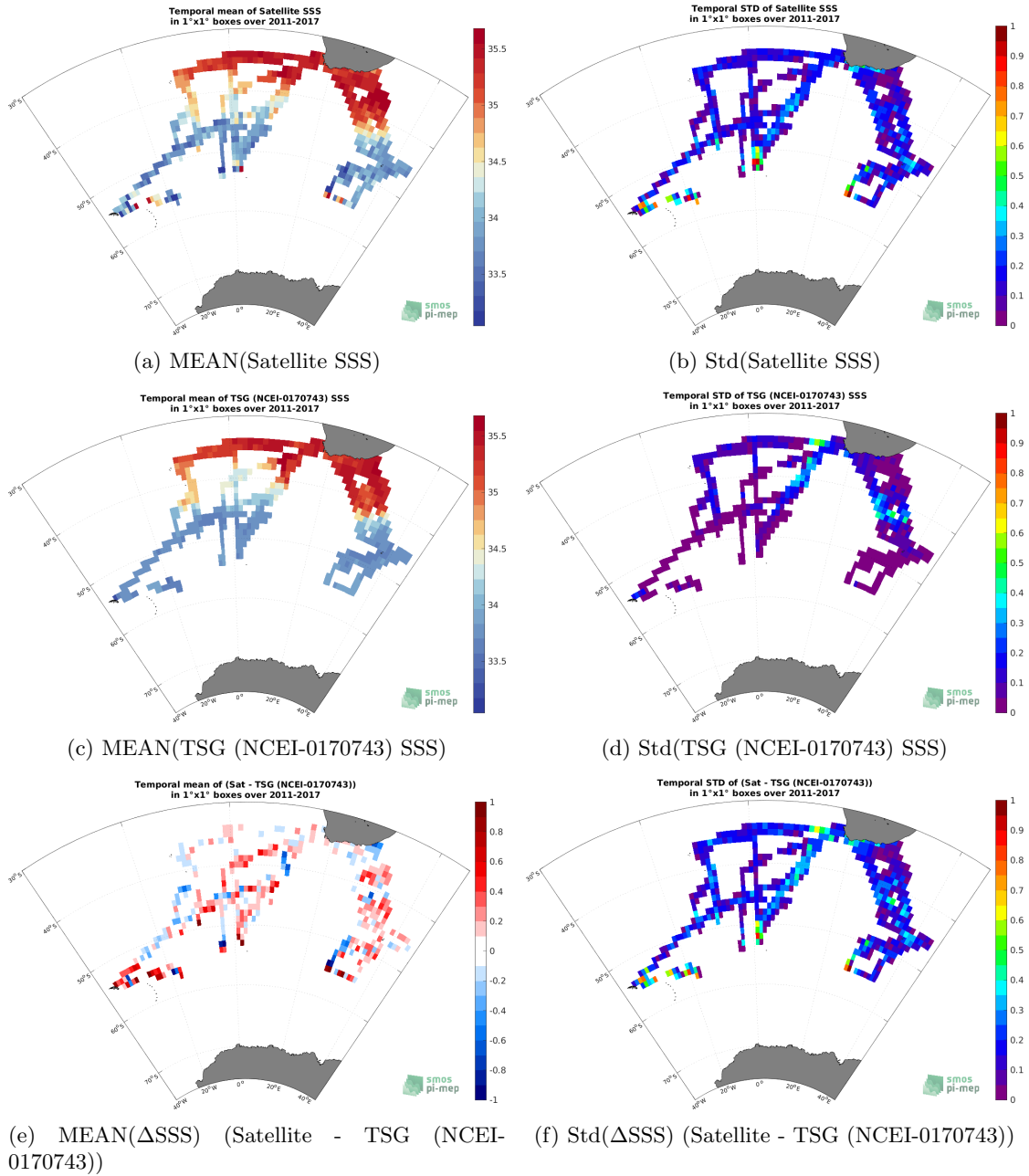
Figure 6: Temporal mean (left) and Std (right) of SSS from SMOS SSS L3 v2 - 9-Days (BEC) (top), TSG (NCEI-0170743) (middle), and of \Delta SSS (Satellite - TSG (NCEI-0170743)). Only match-up pairs are used to generate these maps.
