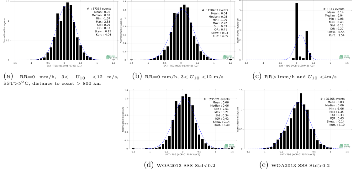
Figure 13: Normalized histogram of \Delta SSS (SMOS SSS L3 v2 - 9-Days (BEC) - TSG (NCEI-0170743)) for 5 different subdatasets corresponding to: RR=0 mm/h, 3 < U_{10} < 12 m/s, SST > 5°C, distance to coast > 800 km (a), RR=0 mm/h, 3 < U_{10} < 12 m/s (b), RR > 1mm/h and U_{10} < 4 m/s (c), WOA2013 SSS Std < 0.2 (d), WOA2013 SSS Std > 0.2 (e).
