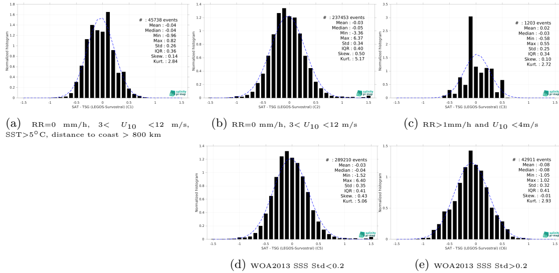
Figure 15: Normalized histogram of \Delta SSS (SMOS SSS L3 v2 - 9-Days (BEC) - TSG (LEGOS-Survostral)) for 5 different subdatasets corresponding to: RR=0 mm/h, 3 < U_{10} < 12 m/s, SST > 5°C, distance to coast > 800 km (a), RR=0 mm/h, 3 < U_{10} < 12 m/s (b), RR > 1mm/h and U_{10} < 4 m/s (c), WOA2013 SSS Std < 0.2 (d), WOA2013 SSS Std > 0.2 (e).
