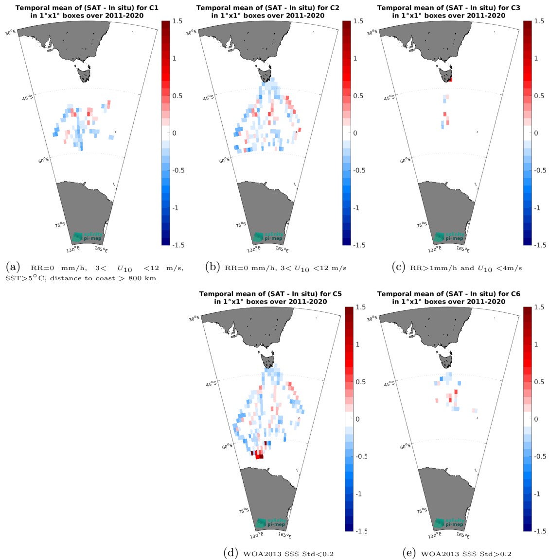
Figure 12: Temporal mean gridded over spatial boxes of size 1^\circ \times 1^\circ of \Delta\text{SSS} (SMOS SSS L3 v2 - 9-Days (BEC) - TSG (LEGOS-Survostral)) for 5 different subdatasets corresponding to: RR=0 mm/h, 3 < U_{10} < 12 m/s, SST > 5^\circ\text{C} , distance to coast > 800 km (a), RR=0 mm/h, 3 < U_{10} < 12 m/s (b), RR > 1 mm/h and U_{10} < 4 m/s (c), WOA2013 SSS Std < 0.2 (d), WOA2013 SSS Std > 0.2 (e).
