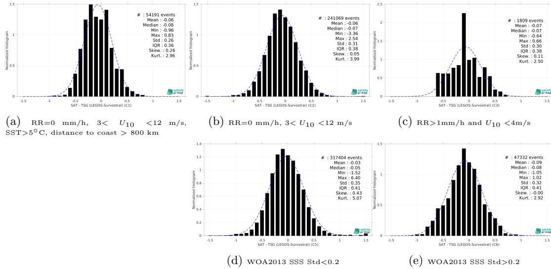
Figure 13: Normalized histogram of \Delta SSS (SMOS SSS L3 v2 - 9-Days (BEC) - TSG (LEGOS-Survostral)) for 5 different subdatasets corresponding to: RR=0 mm/h, 3 < U_{10} < 12 m/s, SST > 5°C, distance to coast > 800 km (a), RR=0 mm/h, 3 < U_{10} < 12 m/s (b), RR > 1mm/h and U_{10} < 4 m/s (c), WOA2013 SSS Std < 0.2 (d), WOA2013 SSS Std > 0.2 (e).
