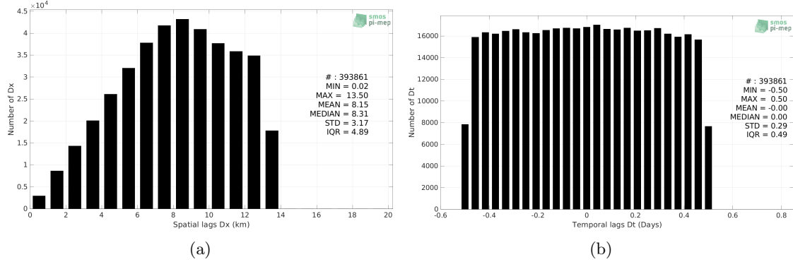
Figure 5: Histograms of the spatial (a) and temporal (b) lags between the location/time of the TSG (LEGOS-Survostral) measurement and the date of the corresponding SMOS SSS L3 v2 - 9-Days (BEC) SSS pixel.
