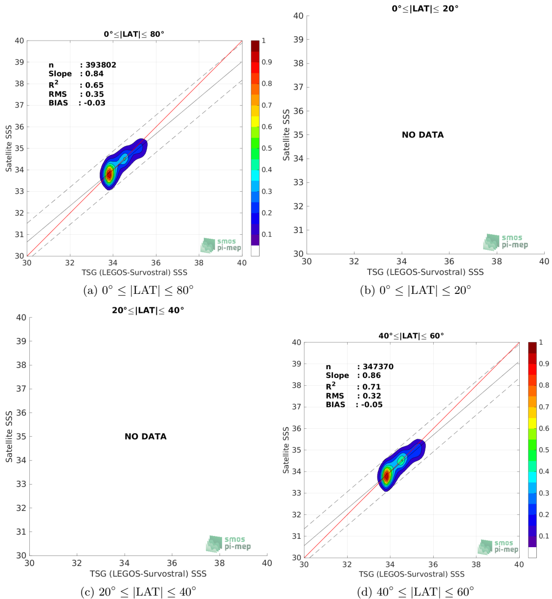
Figure 9: Contour maps of the concentration of SMOS SSS L3 v2 - 9-Days (BEC) SSS (y-axis) versus TSG (LEGOS-Survostral) SSS (x-axis) at match-up pairs for different latitude bands. For each plot, the red line shows x=y . The black thin and dashed lines indicate a linear fit through the data cloud and the \pm 95\% confidence levels, respectively. The number match-up pairs n , the slope and R^2 coefficient of the linear fit, the root mean square (RMS) and the mean bias between satellite and in situ data are indicated for each latitude band in each plots.
