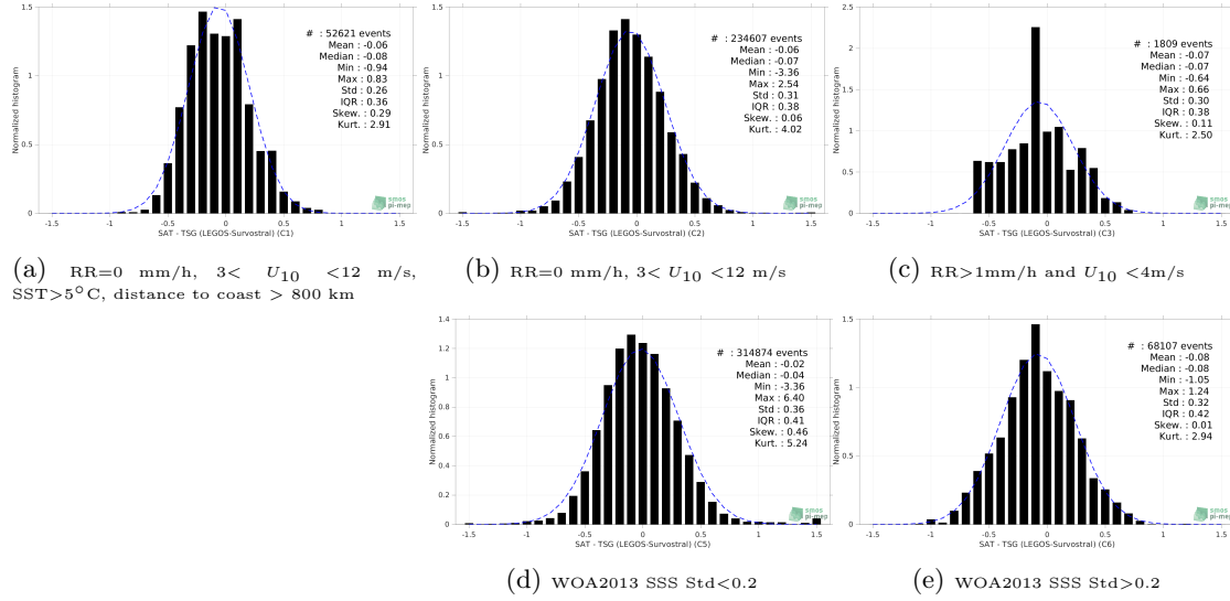
Figure 13: Normalized histogram of \Delta SSS (SMOS SSS L3 v2 - 9-Days (BEC) - TSG (LEGOS-Survostral)) for 5 different subdatasets corresponding to: RR=0 mm/h, 3 < U_{10} < 12 m/s, SST>5°C, distance to coast > 800 km (a), RR=0 mm/h, 3 < U_{10} < 12 m/s (b), RR>1mm/h and U_{10} < 4 m/s (c), WOA2013 SSS Std<0.2 (d), WOA2013 SSS Std>0.2 (e).
