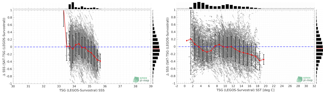
(a) TSG (LEGOS-Survostral) SSS
