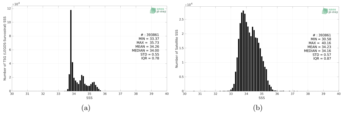
Figure 2: Histograms of SSS from TSG (LEGOS-Survostral) (a) and SMOS SSS L3 v2 - 9-Days (BEC) (b) considering all match-up pairs per bins of 0.1 over the Global Ocean Pi-MEP region and for the full satellite product period.
