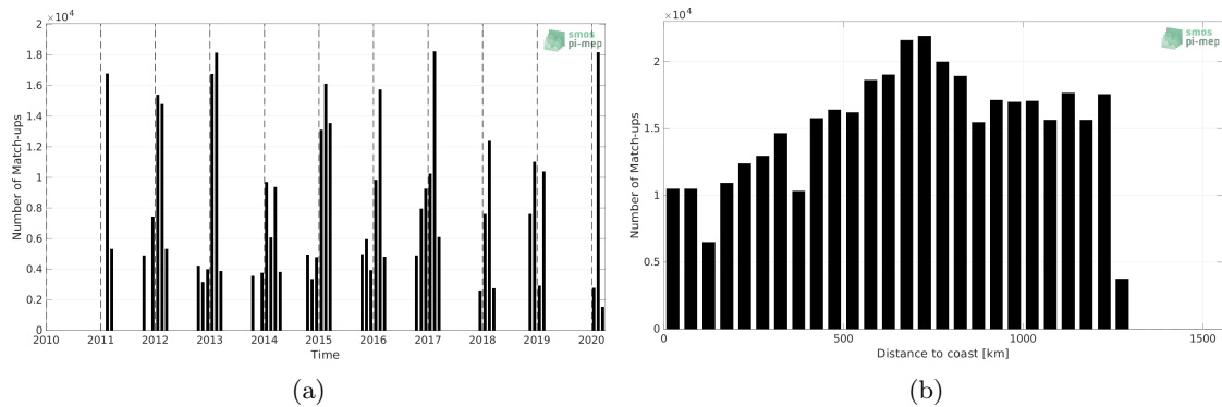
Figure 1: Number of match-ups between TSG (LEGOS-Survostral) and SMOS SSS L3 v2 - 9-Days (BEC) SSS as a function of time (a) and as function of the distance to coast (b) over the Global Ocean Pi-MEP region and for the full satellite product period.
