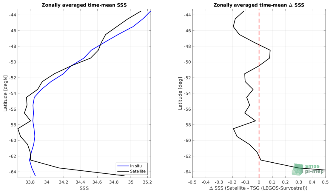
Figure 8: Left panel: Zonal mean SSS from SMOS SSS L3 v2 - 9-Days (BEC) satellite product (black) and from TSG (LEGOS-Survostral) (blue). Right panel: Zonal mean of \Delta SSS (Satellite - TSG (LEGOS-Survostral)) for all the collected Pi-MEP match-up pairs estimated over the full satellite product period.
