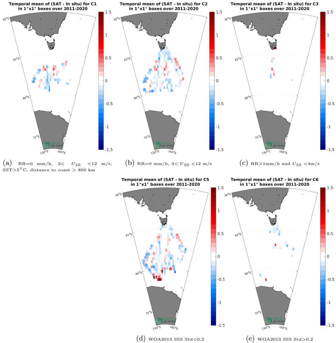
Figure 12: Temporal mean gridded over spatial boxes of size 1°x1° of \Delta SSS (SMOS SSS L3 v2 - 9-Days (BEC) - TSG (LEGOS-Survostral)) for 5 different subdatasets corresponding to:RR=0 mm/h, 3 < U_{10} < 12 m/s, SST>5°C, distance to coast > 800 km (a), RR=0 mm/h, 3 < U_{10} < 12 m/s (b), RR>1mm/h and U_{10} < 4 m/s (c), WOA2013 SSS Std<0.2 (d), WOA2013 SSS Std>0.2 (e).
