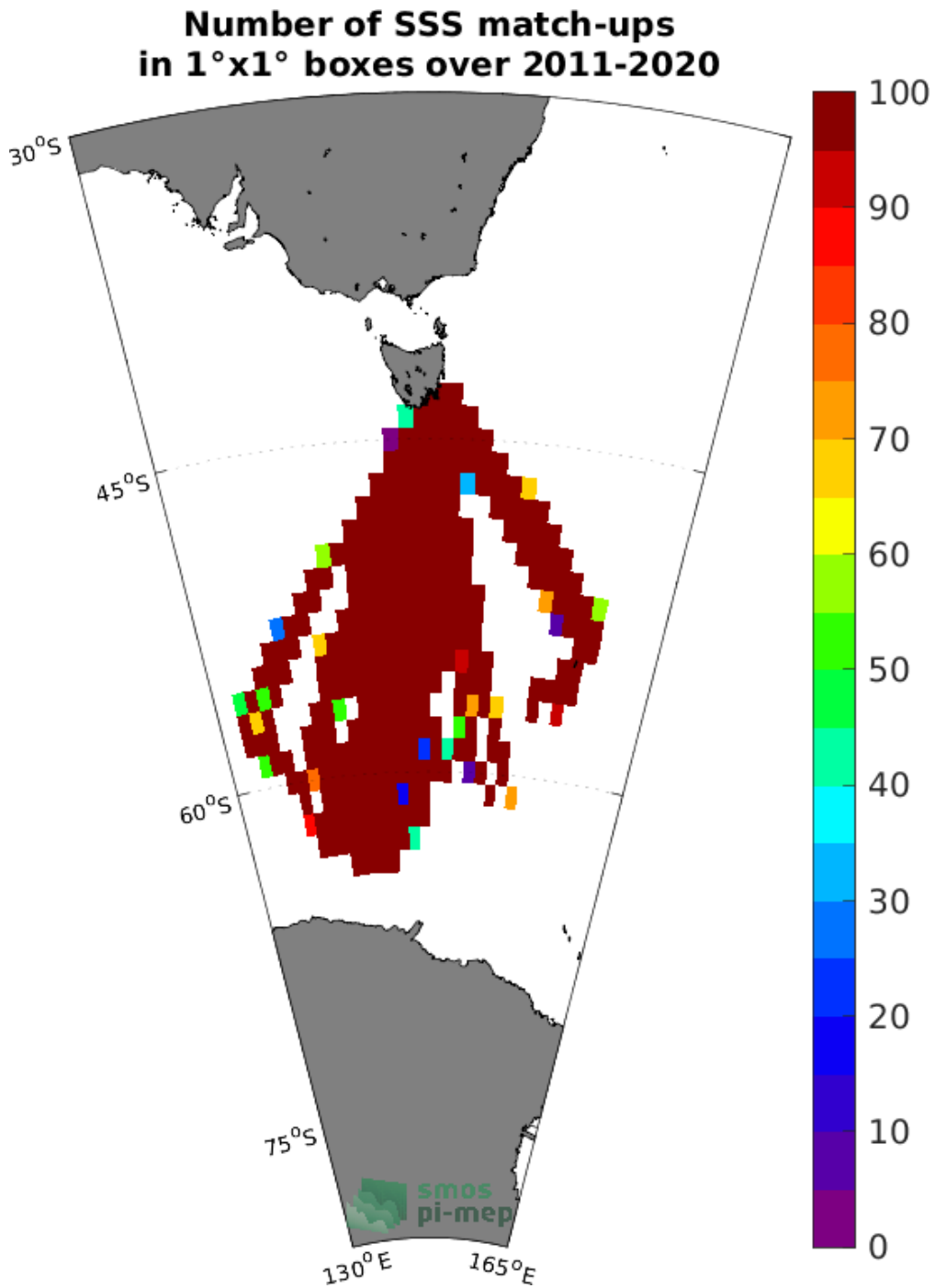
Figure 4: Number of SSS match-ups between TSG (LEGOS-Survostral) SSS and the SMOS SSS L3 v2 - 9-Days (BEC) SSS product for the Global Ocean Pi-MEP region over 1°x1° boxes and for the full satellite product period.
