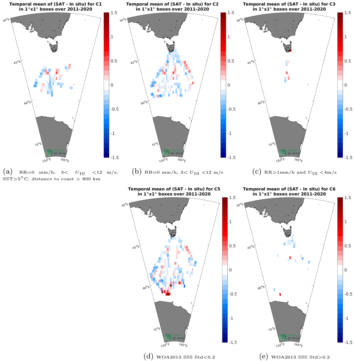
Figure 12: Temporal mean gridded over spatial boxes of size 1^\circ \times 1^\circ of \Delta SSS (SMOS SSS L3 v2 - 9-Days (BEC) - TSG (LEGOS-Survostral)) for 5 different subdatasets corresponding to:RR=0 mm/h, 3 < U_{10} < 12 m/s, SST>5°C, distance to coast > 800 km (a), RR=0 mm/h, 3 < U_{10} < 12 m/s (b), RR>1mm/h and U_{10} < 4 m/s (c), WOA2013 SSS Std<0.2 (d), WOA2013 SSS Std>0.2 (e).
