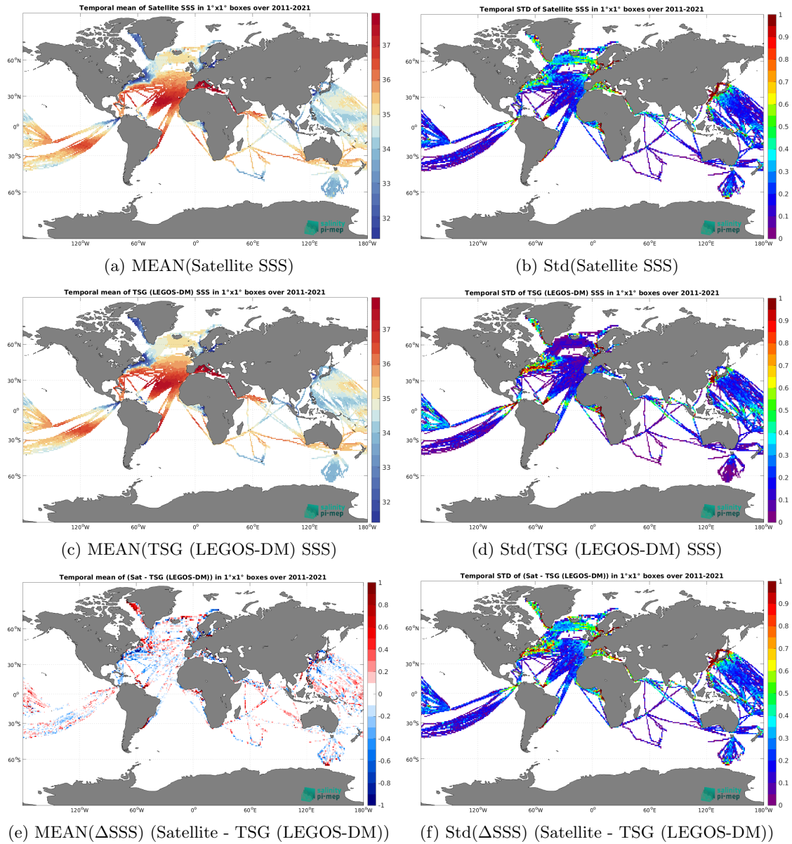
Figure 7: Temporal mean (left) and Std (right) of SSS from SMOS SSS L3 v2 - 9-Days (BEC) (top), TSG (LEGOS-DM) (middle), and of \Delta SSS (Satellite - TSG (LEGOS-DM)). Only match-pair are used to generate these maps.
