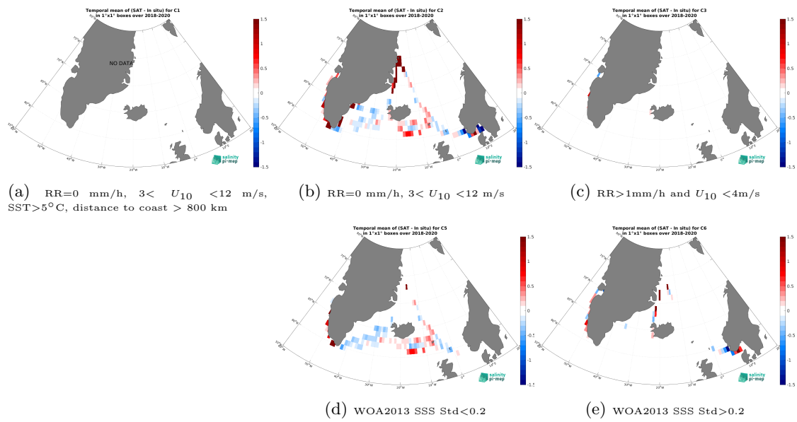
Figure 14: Temporal mean gridded over spatial boxes of size 1^\circ \times 1^\circ of \Delta SSS (SMOS SSS L3 v2 - 9-Days (BEC) - TSG (Lauge-Koch)) for 5 different subdatasets corresponding to:RR=0 mm/h, 3 < U_{10} < 12 m/s, SST > 5^\circ\text{C} , distance to coast > 800 km (a), RR=0 mm/h, 3 < U_{10} < 12 m/s (b), RR > 1 mm/h and U_{10} < 4 m/s (c), WOA2013 SSS Std < 0.2 (d), WOA2013 SSS Std > 0.2 (e).
