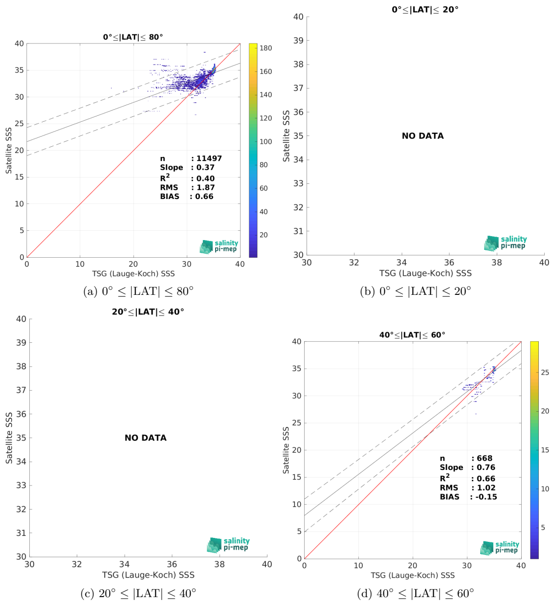
Figure 10: Contour maps of the concentration of SMOS SSS L3 v2 - 9-Days (BEC) SSS (y-axis) versus TSG (Lauge-Koch) SSS (x-axis) at match-up pairs for different latitude bands. For each plot, the red line shows x=y . The black thin and dashed lines indicate a linear fit through the data cloud and the \pm 95\% confidence levels, respectively. The number match-up pairs n , the slope and R^2 coefficient of the linear fit, the root mean square (RMS) and the mean bias between satellite and in situ data are indicated for each latitude band in each plots.
