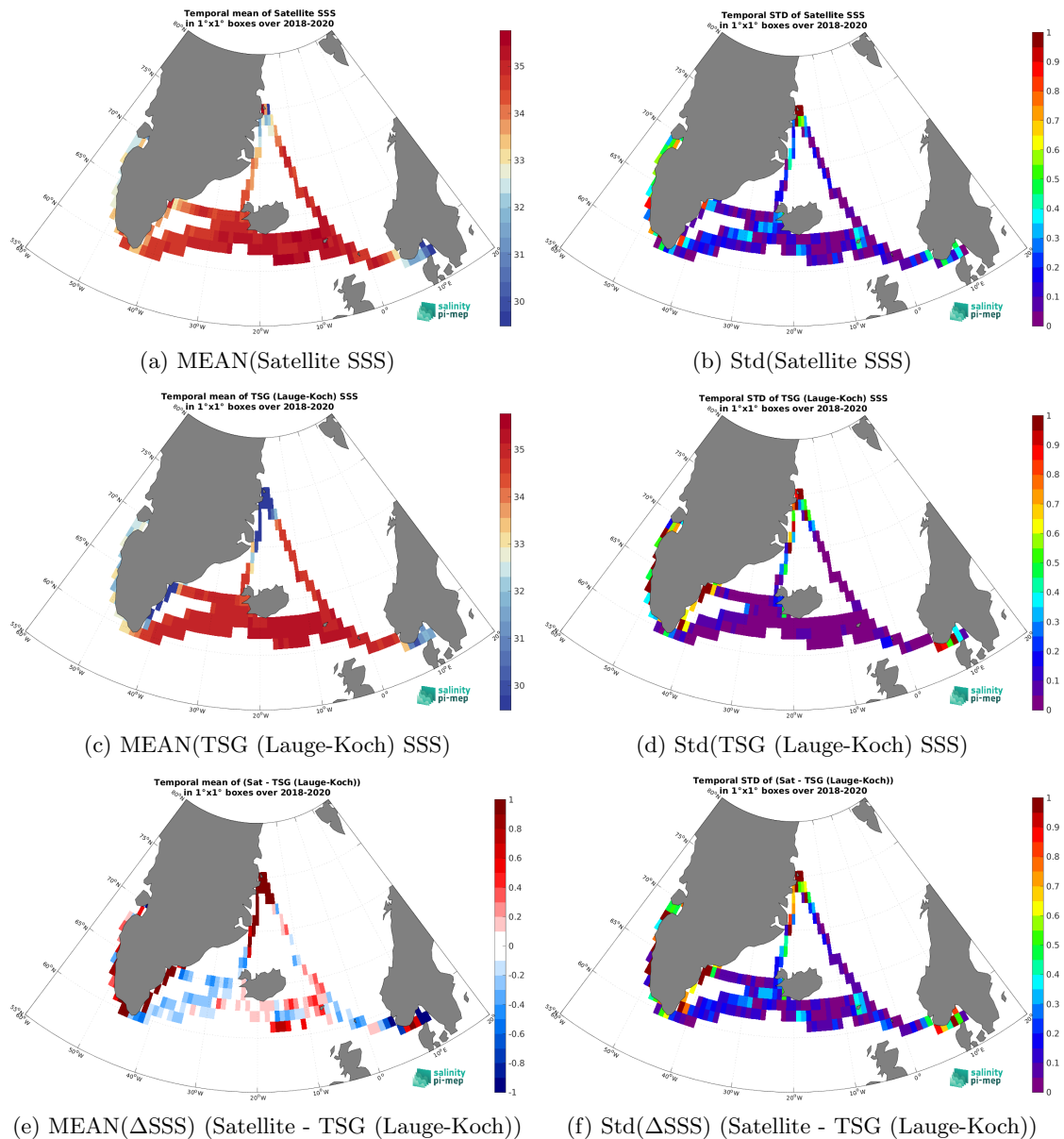
Figure 7: Temporal mean (left) and Std (right) of SSS from SMOS SSS L3 v2 - 9-Days (BEC) (top), TSG (Lauge-Koch) (middle), and of \Delta SSS (Satellite - TSG (Lauge-Koch)). Only match-up pairs are used to generate these maps.
