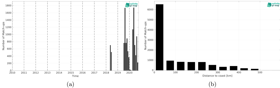
Figure 2: Number of match-ups between TSG (Lauge-Koch) and SMOS SSS L3 v2 - 9-Days (BEC) SSS as a function of time (a) and as function of the distance to coast (b) over the Global Ocean Pi-MEP region and for the full satellite product period.
