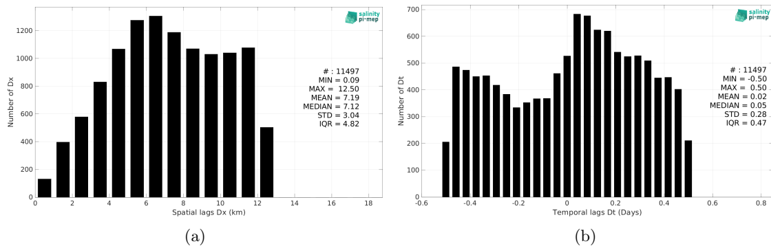
Figure 6: Histograms of the spatial (a) and temporal (b) lags between the location/time of the TSG (Lauge-Koch) measurement and the date of the corresponding SMOS SSS L3 v2 - 9-Days (BEC) SSS pixel.
