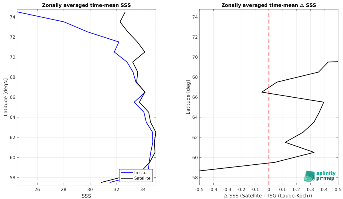
Figure 9: Left panel: Zonal mean SSS from SMOS SSS L3 v2 - 9-Days (BEC) satellite product (black) and from TSG (Lauge-Koch) (blue). Right panel: Zonal mean of \Delta SSS (Satellite - TSG (Lauge-Koch)) for all the collected Pi-MEP match-up pairs estimated over the full satellite product period.
