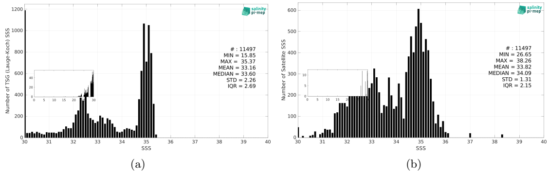
Figure 3: Histograms of SSS from TSG (Lauge-Koch) (a) and SMOS SSS L3 v2 - 9-Days (BEC) (b) considering all match-up pairs per bins of 0.1 over the Global Ocean Pi-MEP region and for the full satellite product period.
