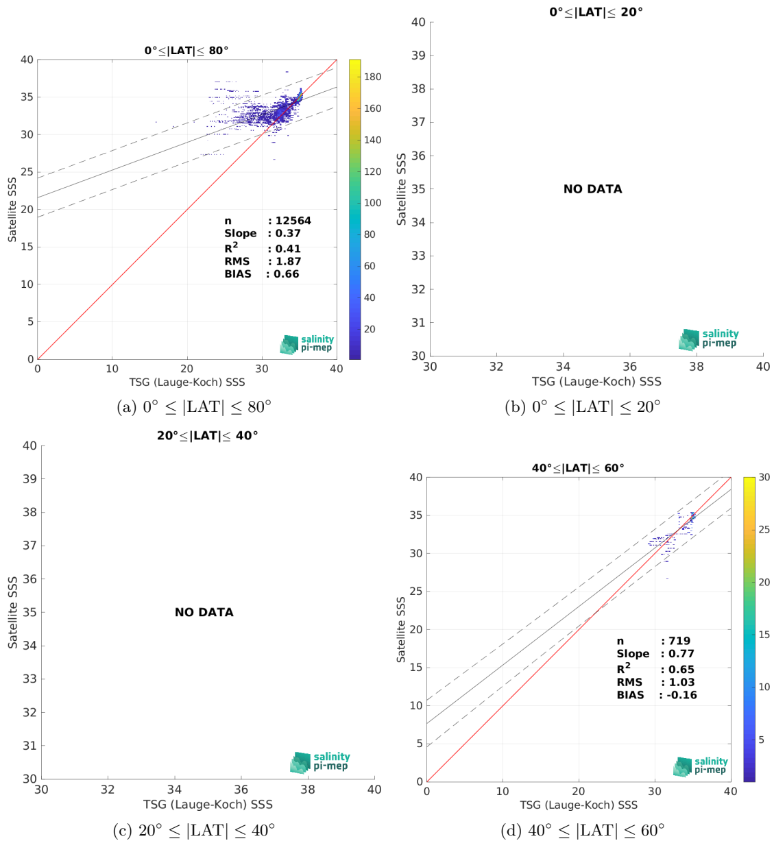
Figure 9: Contour maps of the concentration of SMOS SSS L3 v2 - 9-Days (BEC) SSS (y-axis) versus TSG (Lauge-Koch) SSS (x-axis) at match-up pairs for different latitude bands. For each plot, the red line shows x=y . The black thin and dashed lines indicate a linear fit through the data cloud and the \pm 95\% confidence levels, respectively. The number match-up pairs n , the slope and R^2 coefficient of the linear fit, the root mean square (RMS) and the mean bias between satellite and in situ data are indicated for each latitude band in each plots.
