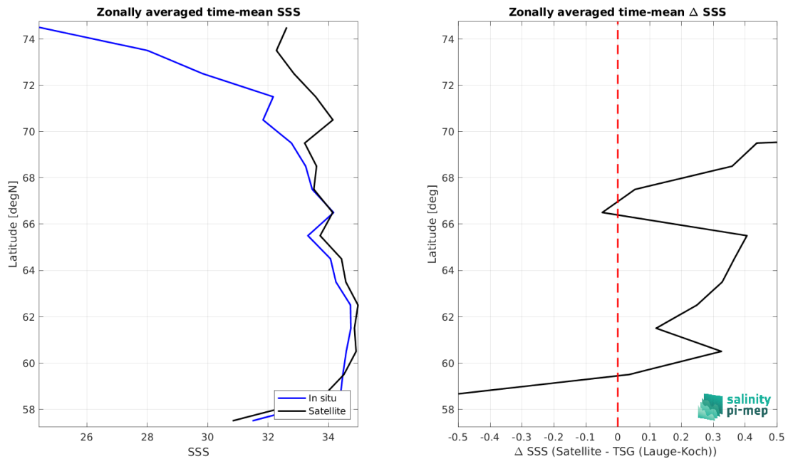
Figure 8: Left panel: Zonal mean SSS from SMOS SSS L3 v2 - 9-Days (BEC) satellite product (black) and from TSG (Lauge-Koch) (blue). Right panel: Zonal mean of \Delta SSS (Satellite - TSG (Lauge-Koch)) for all the collected Pi-MEP match-up pairs estimated over the full satellite product period.
