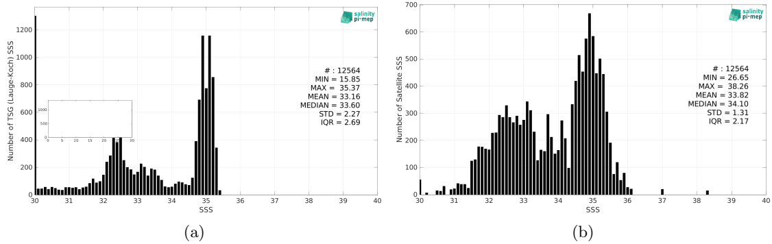
Figure 2: Histograms of SSS from TSG (Lauge-Koch) (a) and SMOS SSS L3 v2 - 9-Days (BEC) (b) considering all match-up pairs per bins of 0.1 over the Global Ocean Pi-MEP region and for the full satellite product period.
