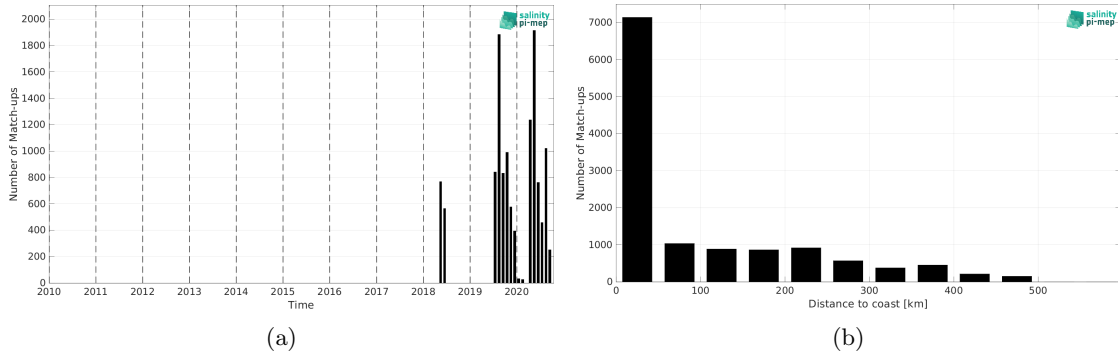
Figure 1: Number of match-ups between TSG (Lauge-Koch) and SMOS SSS L3 v2 - 9-Days (BEC) SSS as a function of time (a) and as function of the distance to coast (b) over the Global Ocean Pi-MEP region and for the full satellite product period.
