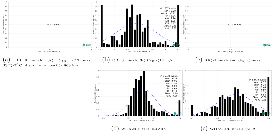
Figure 13: Normalized histogram of \Delta SSS (SMOS SSS L3 v2 - 9-Days (BEC) - TSG (Lauge-Koch)) for 5 different subdatasets corresponding to: RR=0 mm/h, 3 < U_{10} < 12 m/s, SST > 5°C, distance to coast > 800 km (a), RR=0 mm/h, 3 < U_{10} < 12 m/s (b), RR > 1mm/h and U_{10} < 4 m/s (c), WOA2013 SSS Std < 0.2 (d), WOA2013 SSS Std > 0.2 (e).
