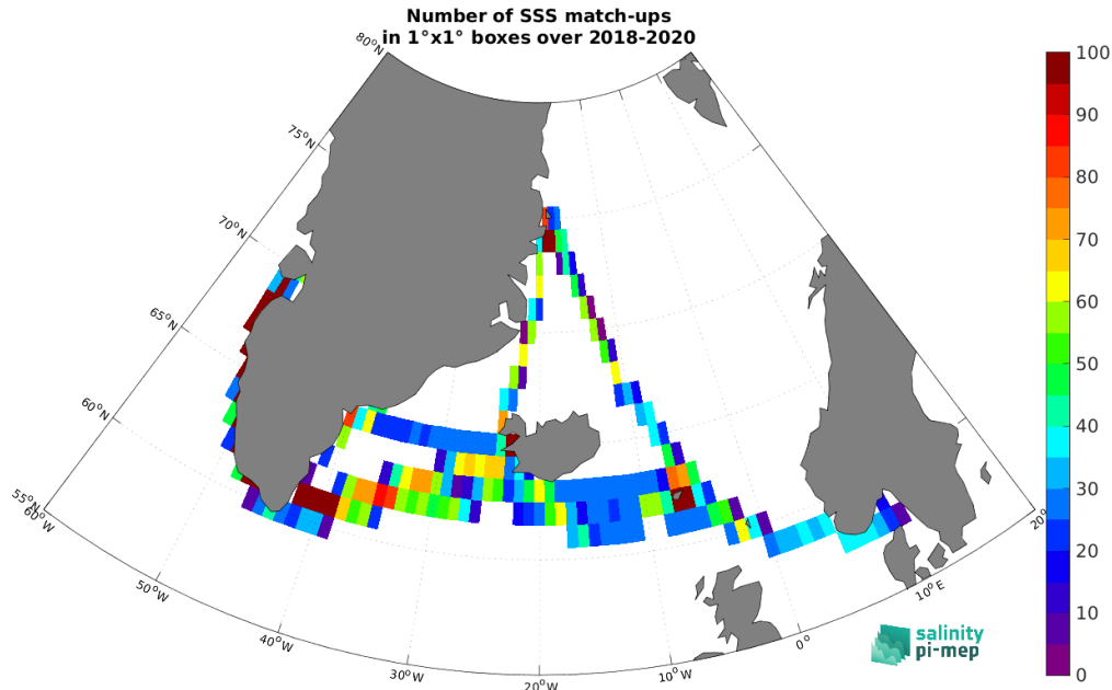
Figure 4: Number of SSS match-ups between TSG (Lauge-Koch) SSS and the SMOS SSS L3 v2 - 9-Days (BEC) SSS product for the Global Ocean Pi-MEP region over 1^\circ \times 1^\circ boxes and for the full satellite product period.
