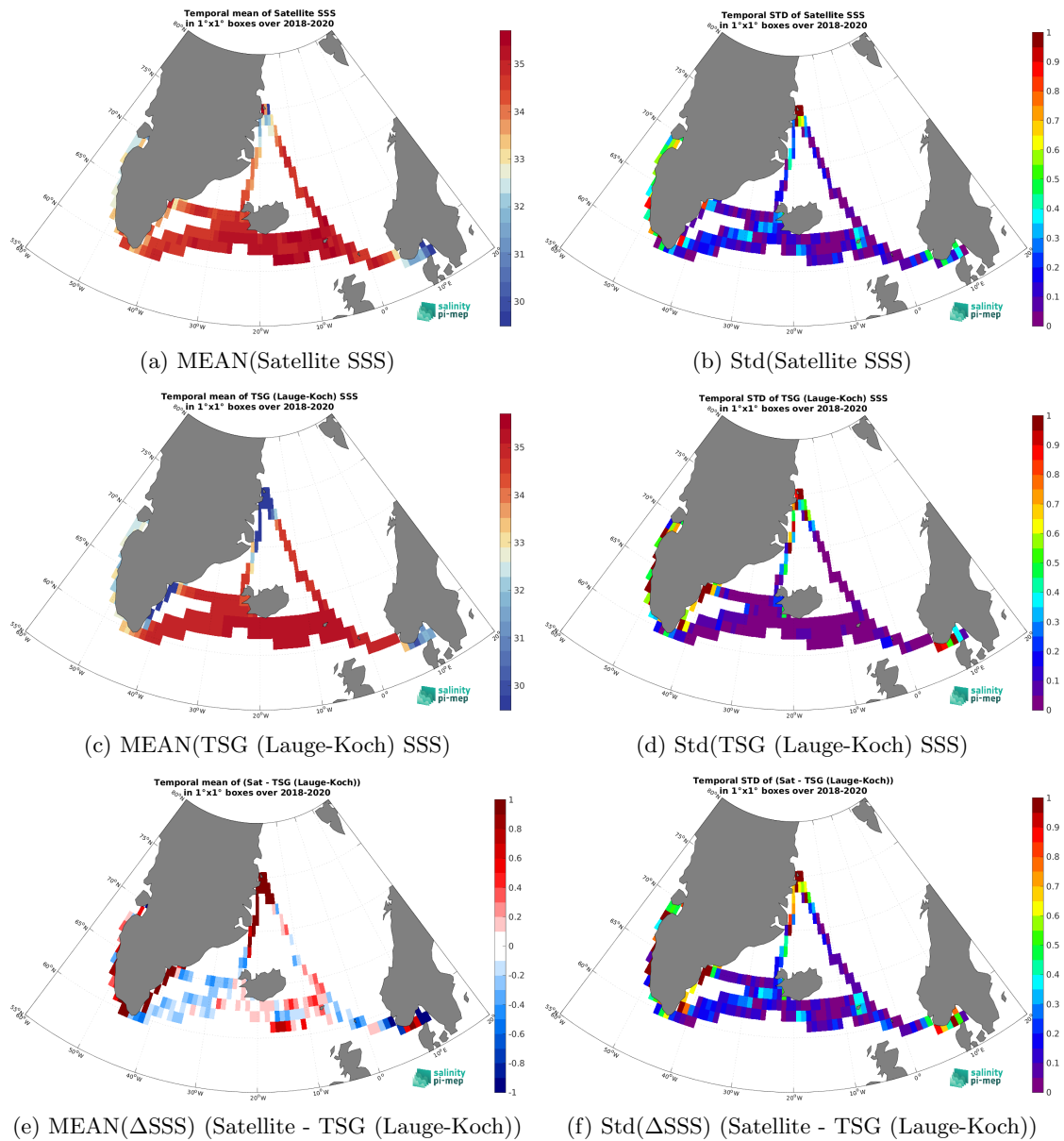
Figure 6: Temporal mean (left) and Std (right) of SSS from SMOS SSS L3 v2 - 9-Days (BEC) (top), TSG (Lauge-Koch) (middle), and of \Delta SSS (Satellite - TSG (Lauge-Koch)). Only match-up pairs are used to generate these maps.
