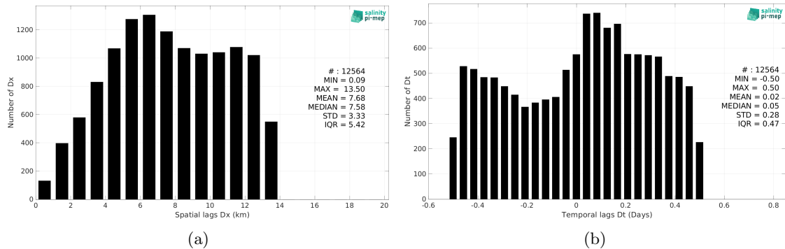
Figure 5: Histograms of the spatial (a) and temporal (b) lags between the location/time of the TSG (Lauge-Koch) measurement and the date of the corresponding SMOS SSS L3 v2 - 9-Days (BEC) SSS pixel.
