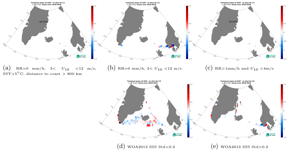
Figure 12: Temporal mean gridded over spatial boxes of size 1^{\circ}\times 1^{\circ} of \Delta\text{SSS} (SMOS SSS L3 v2 - 9-Days (BEC) - TSG (Lauge-Koch)) for 5 different subdatasets corresponding to:RR=0 mm/h, 3 < U_{10} < 12 m/s, SST > 5^{\circ}\text{C} , distance to coast > 800 km (a), RR=0 mm/h, 3 < U_{10} < 12 m/s (b), RR > 1 mm/h and U_{10} < 4 m/s (c), WOA2013 SSS Std < 0.2 (d), WOA2013 SSS Std > 0.2 (e).
