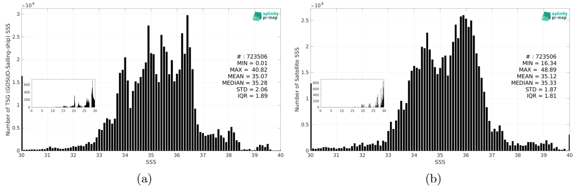
Figure 3: Histograms of SSS from TSG (GOSUD-Sailing-ship) (a) and SMOS SSS L3 v2 - 9-Days (BEC) (b) considering all match-up pairs per bins of 0.1 over the Global Ocean Pi-MEP region and for the full satellite product period.
