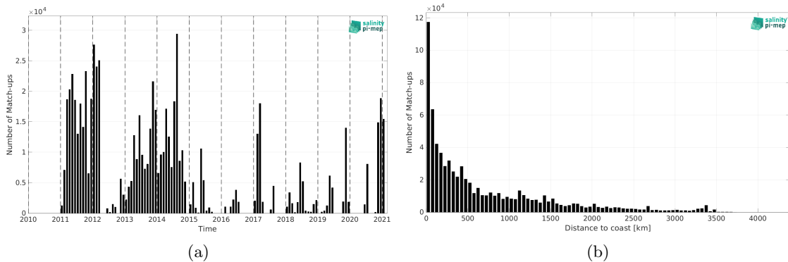
Figure 2: Number of match-ups between TSG (GOSUD-Sailing-ship) and SMOS SSS L3 v2 - 9-Days (BEC) SSS as a function of time (a) and as function of the distance to coast (b) over the Global Ocean Pi-MEP region and for the full satellite product period.
