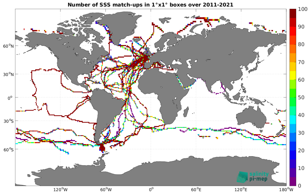
Figure 5: Number of SSS match-ups between TSG (GOSUD-Sailing-ship) SSS and the SMOS SSS L3 v2 - 9-Days (BEC) SSS product for the Global Ocean Pi-MEP region over 1^\circ \times 1^\circ boxes and for the full satellite product period.
