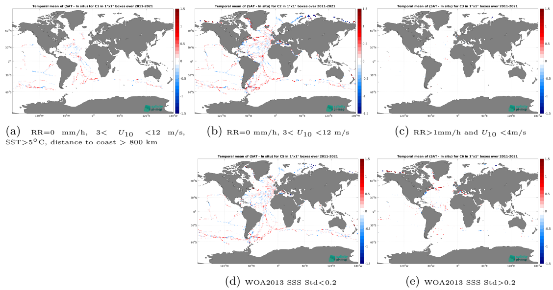
Figure 14: Temporal mean gridded over spatial boxes of size 1^\circ \times 1^\circ of \Delta SSS (SMOS SSS L3 v2 - 9-Days (BEC) - TSG (GOSUD-Sailing-ship)) for 5 different subdatasets corresponding to: RR=0 mm/h, 3 < U_{10} < 12 m/s, SST > 5°C, distance to coast > 800 km (a), RR=0 mm/h, 3 < U_{10} < 12 m/s (b), RR > 1mm/h and U_{10} < 4 m/s (c), WOA2013 SSS Std < 0.2 (d), WOA2013 SSS Std > 0.2 (e).
