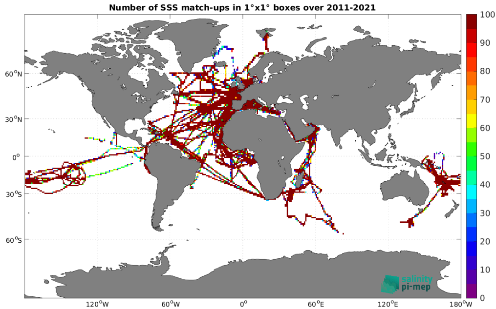
Figure 4: Number of SSS match-ups between TSG (GOSUD-Research-vessel) SSS and the SMOS SSS L3 v2 - 9-Days (BEC) SSS product for the Global Ocean Pi-MEP region over 1^{\circ} \times 1^{\circ} boxes and for the full satellite product period.
