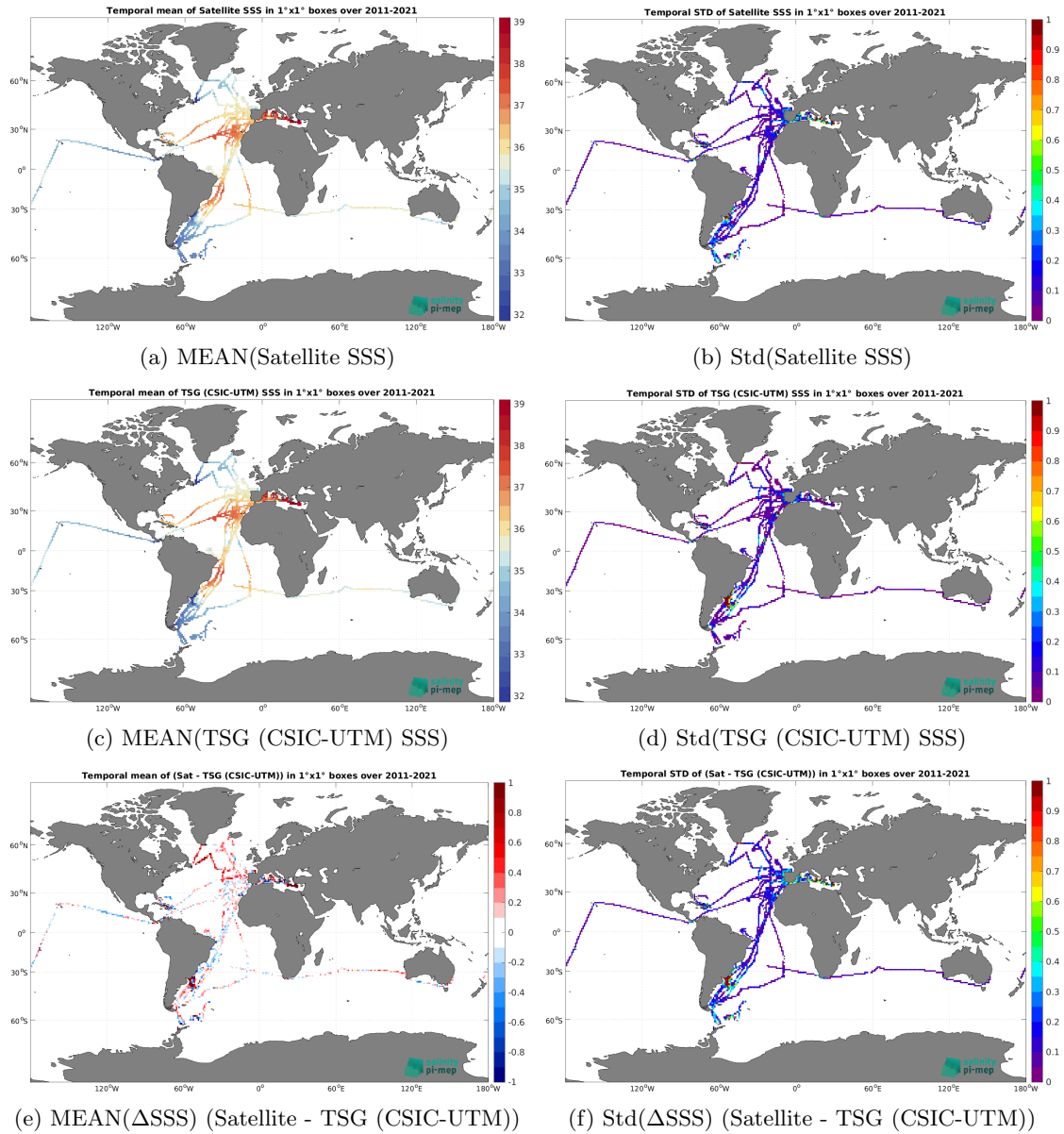
Figure 7: Temporal mean (left) and Std (right) of SSS from SMOS SSS L3 v2 - 9-Days (BEC) (top), TSG (CSIC-UTM) (middle), and of \Delta SSS (Satellite - TSG (CSIC-UTM)). Only match-up pairs are used to generate these maps.
