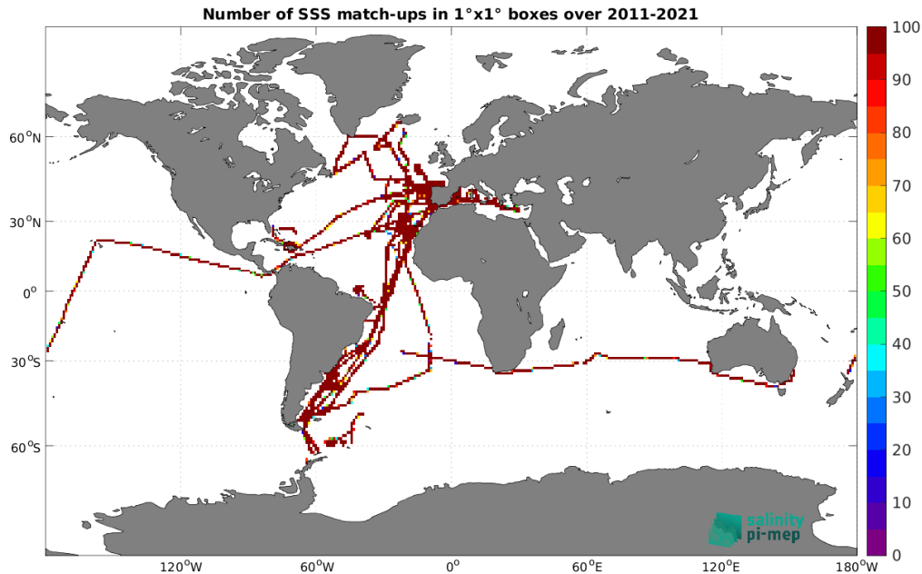
Figure 5: Number of SSS match-ups between TSG (CSIC-UTM) SSS and the SMOS SSS L3 v2 - 9-Days (BEC) SSS product for the Global Ocean Pi-MEP region over 1^\circ \times 1^\circ boxes and for the full satellite product period.
