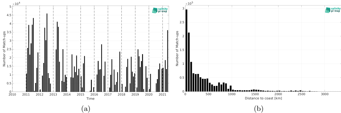
Figure 2: Number of match-ups between TSG (CSIC-UTM) and SMOS SSS L3 v2 - 9-Days (BEC) SSS as a function of time (a) and as function of the distance to coast (b) over the Global Ocean Pi-MEP region and for the full satellite product period.
