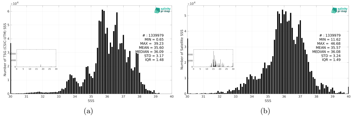
Figure 3: Histograms of SSS from TSG (CSIC-UTM) (a) and SMOS SSS L3 v2 - 9-Days (BEC) (b) considering all match-up pairs per bins of 0.1 over the Global Ocean Pi-MEP region and for the full satellite product period.
