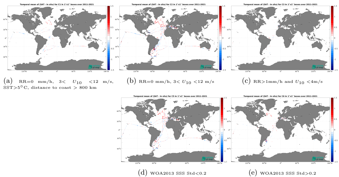
Figure 14: Temporal mean gridded over spatial boxes of size 1^\circ \times 1^\circ of \Delta SSS (SMOS SSS L3 v2 - 9-Days (BEC) - TSG (CSIC-UTM)) for 5 different subdatasets corresponding to:RR=0 mm/h, 3 < U_{10} < 12 m/s, SST > 5^\circ\text{C} , distance to coast > 800 km (a), RR=0 mm/h, 3 < U_{10} < 12 m/s (b), RR > 1 mm/h and U_{10} < 4 m/s (c), WOA2013 SSS Std < 0.2 (d), WOA2013 SSS Std > 0.2 (e).
