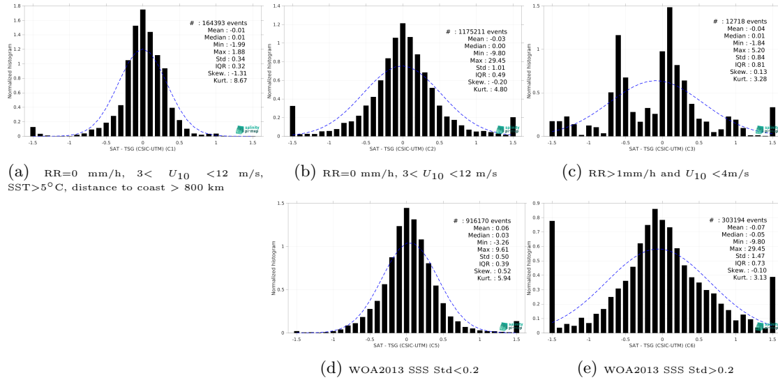
Figure 13: Normalized histogram of \Delta\text{SSS} (SMOS SSS L3 v2 - 9-Days (BEC) - TSG (CSIC-UTM)) for 5 different subdatasets corresponding to: RR=0 mm/h, 3 < U_{10} < 12 m/s, SST>5°C, distance to coast > 800 km (a), RR=0 mm/h, 3 < U_{10} < 12 m/s (b), RR>1mm/h and U_{10} < 4 m/s (c), WOA2013 SSS Std<0.2 (d), WOA2013 SSS Std>0.2 (e).
