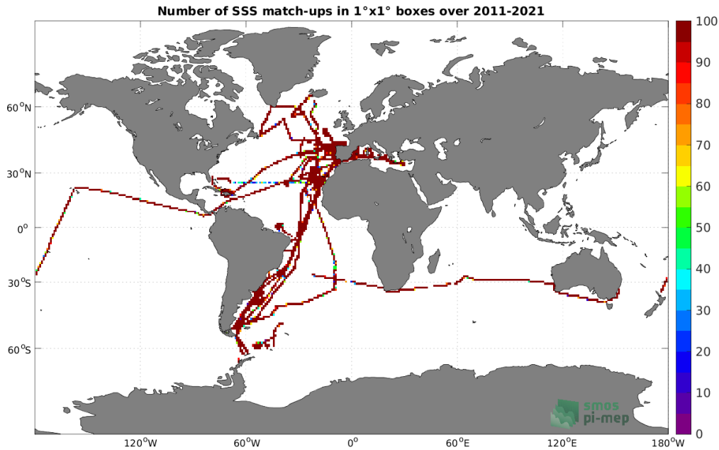
Figure 4: Number of SSS match-ups between TSG (CSIC-UTM) SSS and the SMOS SSS L3 v2 - 9-Days (BEC) SSS product for the Global Ocean Pi-MEP region over 1^\circ \times 1^\circ boxes and for the full satellite product period.
