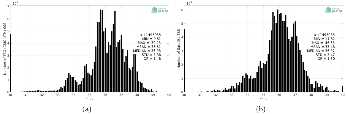
Figure 2: Histograms of SSS from TSG (CSIC-UTM) (a) and SMOS SSS L3 v2 - 9-Days (BEC) (b) considering all match-up pairs per bins of 0.1 over the Global Ocean Pi-MEP region and for the full satellite product period.
