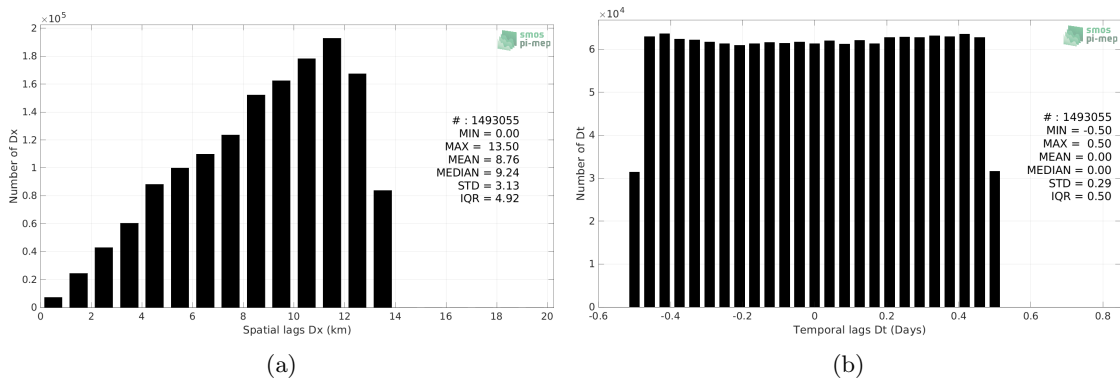
Figure 5: Histograms of the spatial (a) and temporal (b) lags between the location/time of the TSG (CSIC-UTM) measurement and the date of the corresponding SMOS SSS L3 v2 - 9-Days (BEC) SSS pixel.
