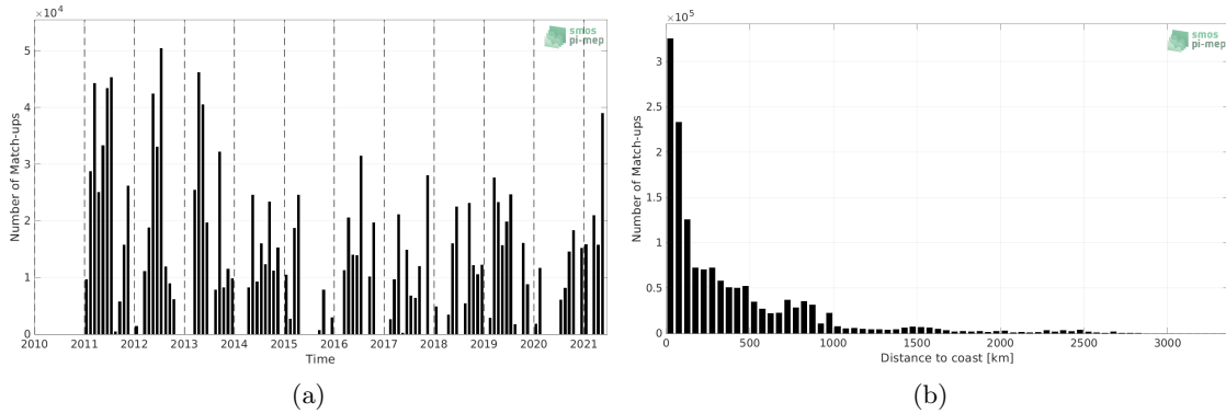
Figure 1: Number of match-ups between TSG (CSIC-UTM) and SMOS SSS L3 v2 - 9-Days (BEC) SSS as a function of time (a) and as function of the distance to coast (b) over the Global Ocean Pi-MEP region and for the full satellite product period.
