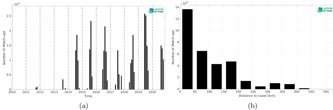
Figure 2: Number of match-ups between TSG (Amundsen) and SMOS SSS L3 v2 - 9-Days (BEC) SSS as a function of time (a) and as function of the distance to coast (b) over the Global Ocean Pi-MEP region and for the full satellite product period.
