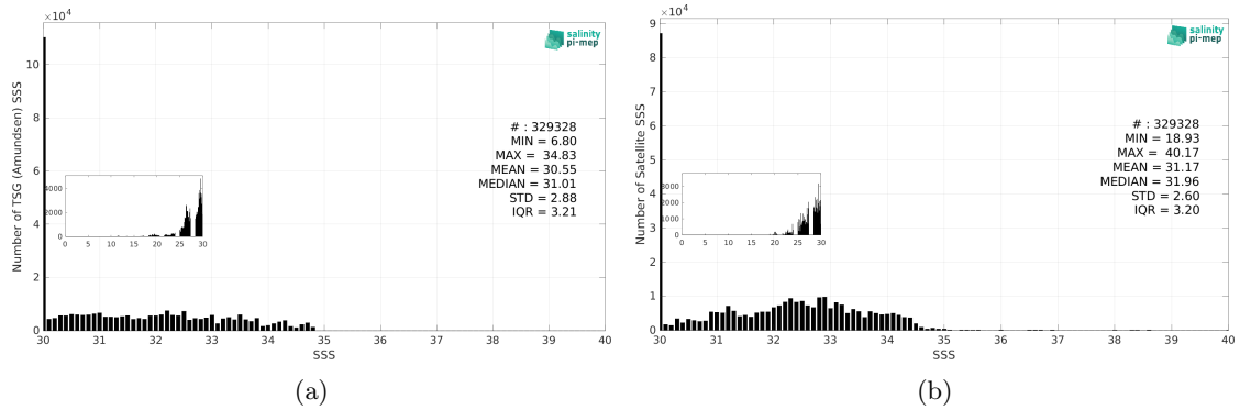
Figure 3: Histograms of SSS from TSG (Amundsen) (a) and SMOS SSS L3 v2 - 9-Days (BEC) (b) considering all match-up pairs per bins of 0.1 over the Global Ocean Pi-MEP region and for the full satellite product period.
